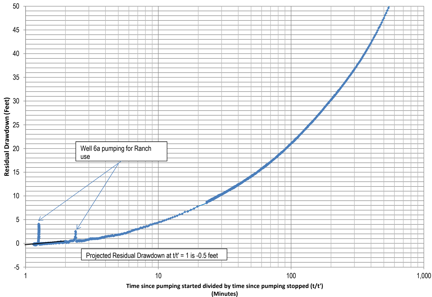
Figure 27. Well 6B Recovery Analysis, Well 6A/6B 72 Hour Constant Rate Test
