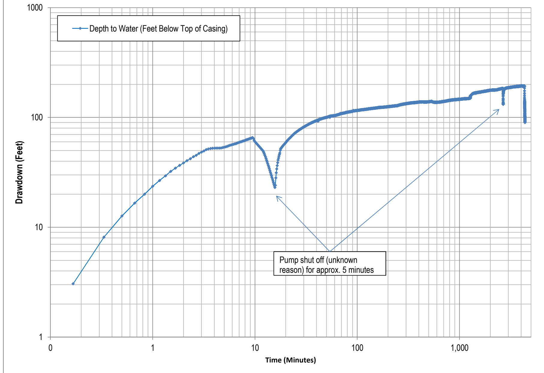
Figure 29. Well 8 72 Hour Constant Rate Test Log Water Level Drawdown
