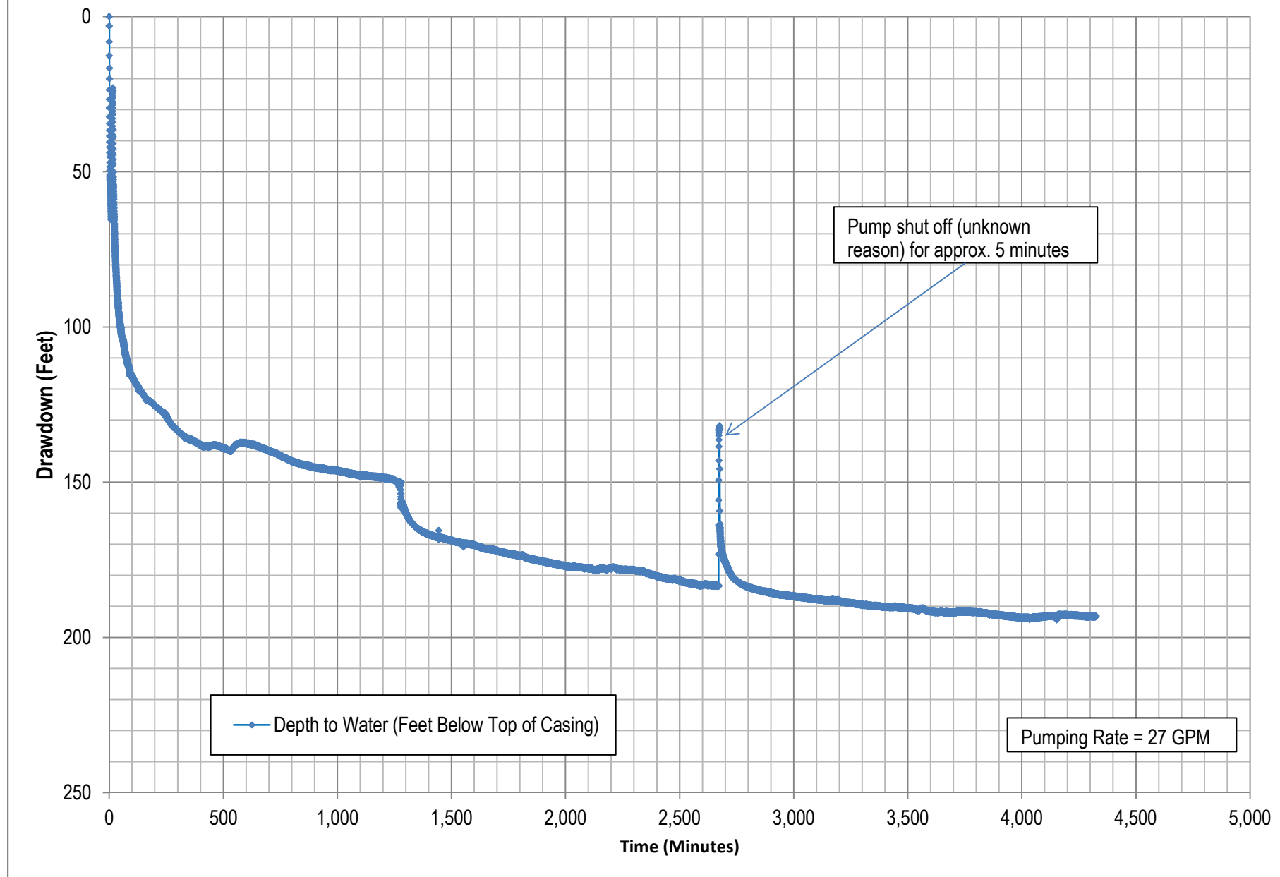
Figure 28. Well 8 72 Hour Constant Rate Test Water Level Drawdown
