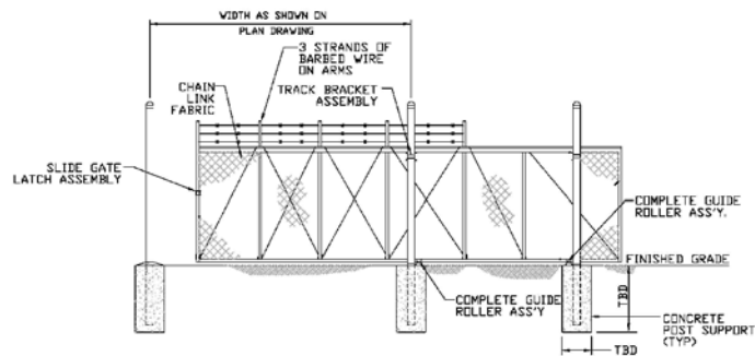
TYPICAL CANTILEVER SLIDING GATE NOT TO SCALE
