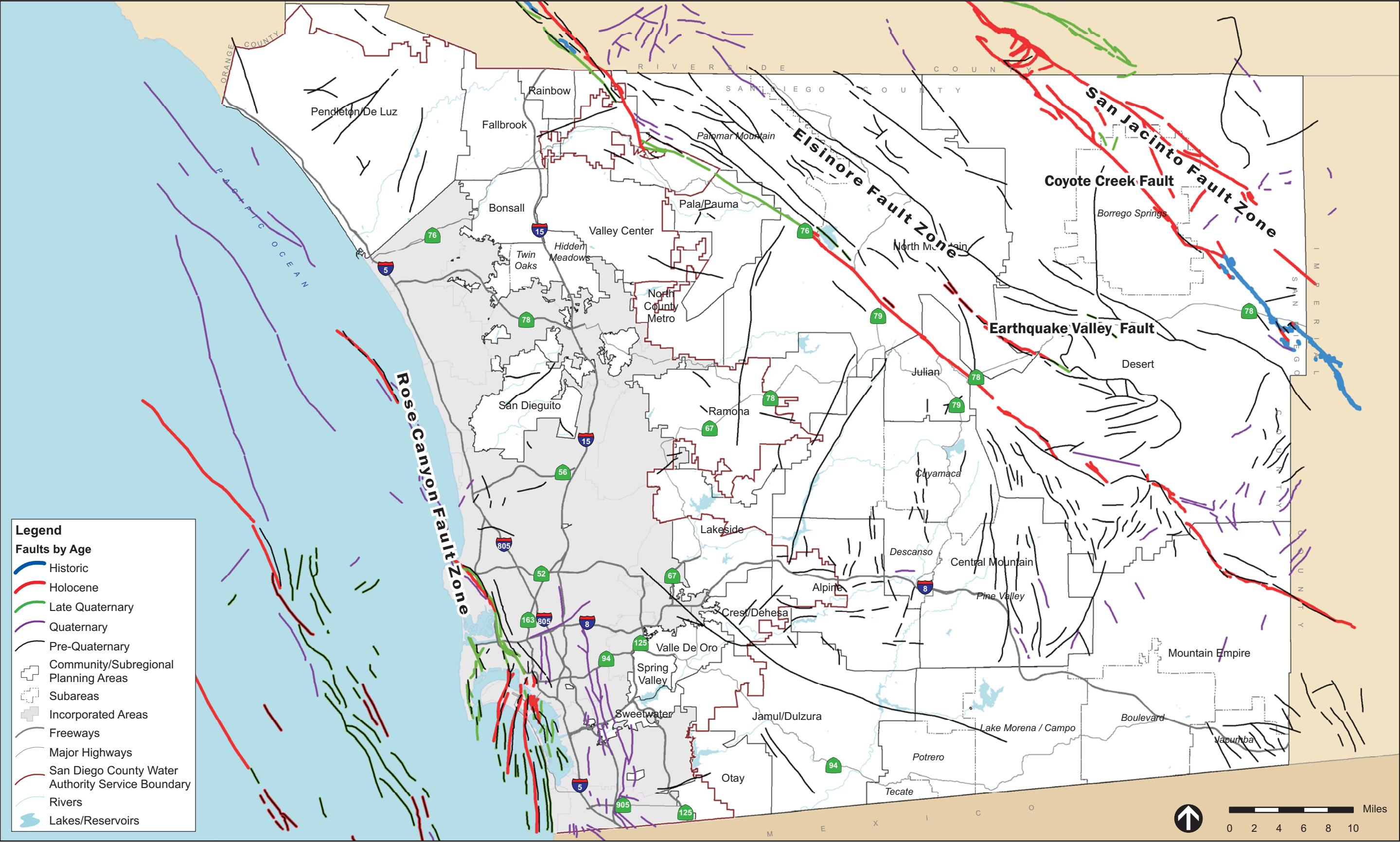
MAPPED FAULTS
