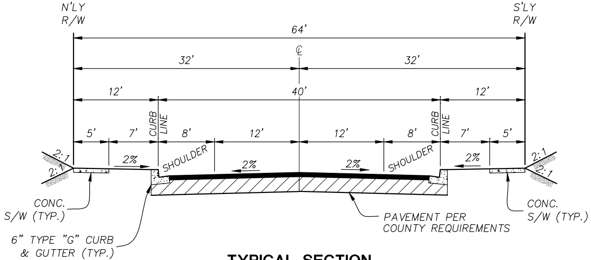
TYPICAL SECTION 2.2C LIGHT COLLECTOR
