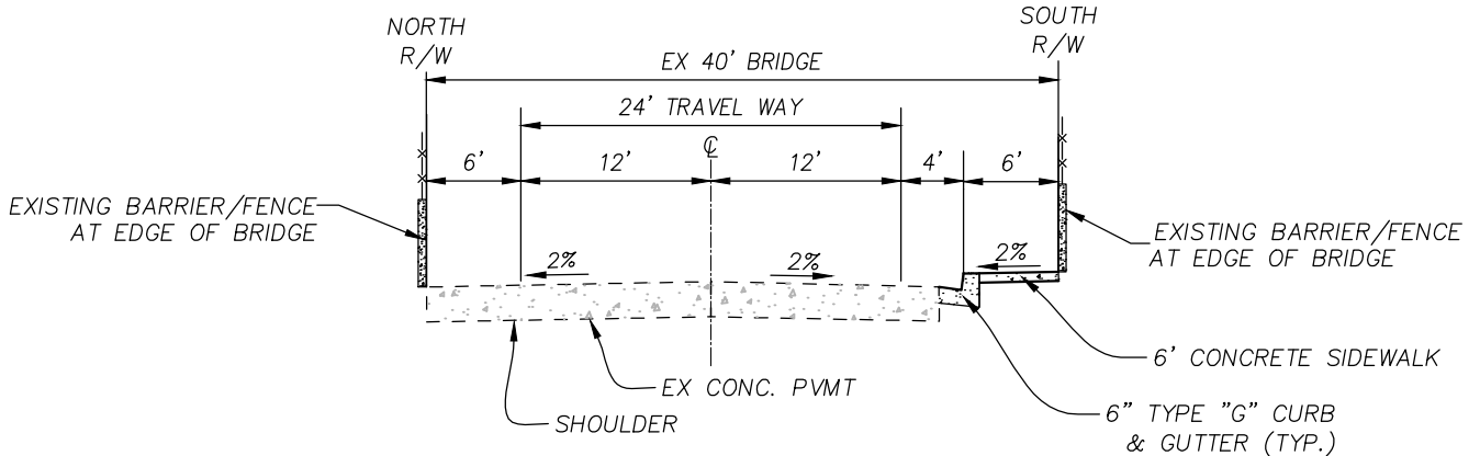
PROPOSED TYPICAL SECTION (2.2C LIGHT COLLECTOR) WEST LILAC RD OVER I-15 BRIDGE
