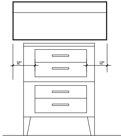
PIZZA OVEN ELEVATION
