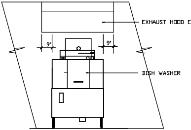
DISH WASHER HOOD ELEVATION
