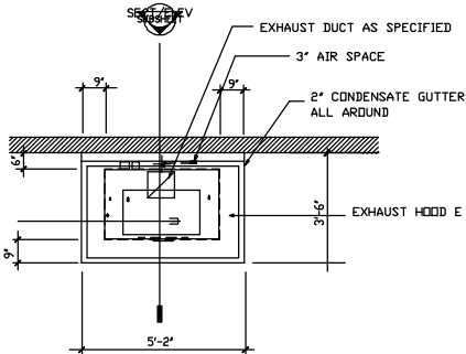
DISH WASHER HOOD PLAN VIEW
