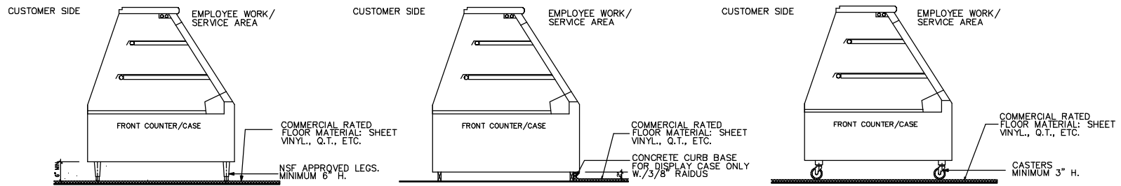
Ⓐ TYP. NSF LEGS DETAIL @ DISPLAY CASE
