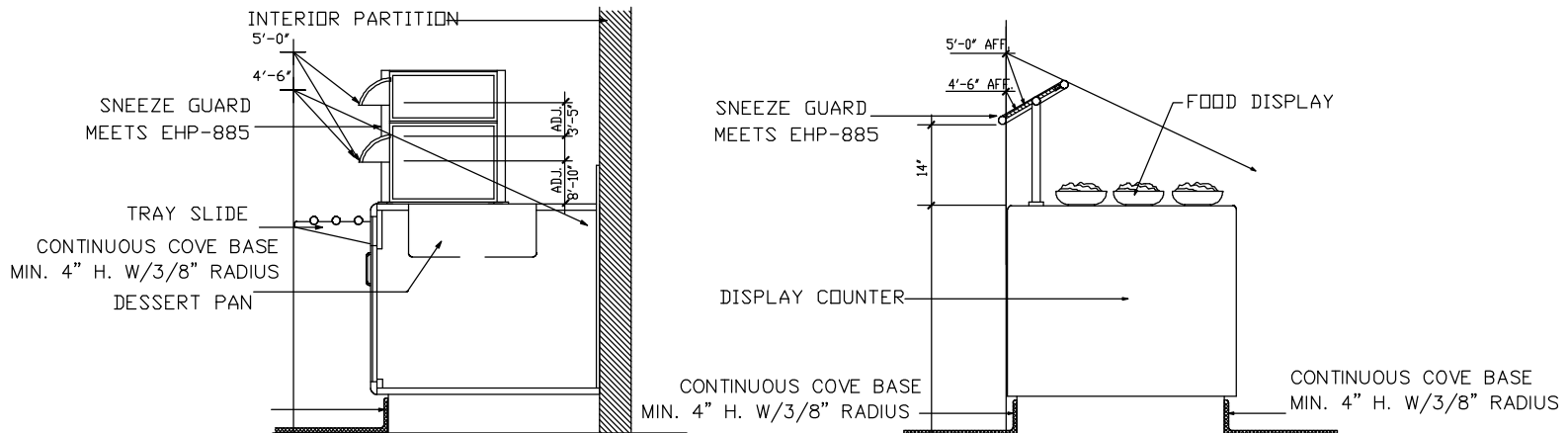
Ⓒ TYP. SNEEZE GUARD @ DESSERT COUNTER
