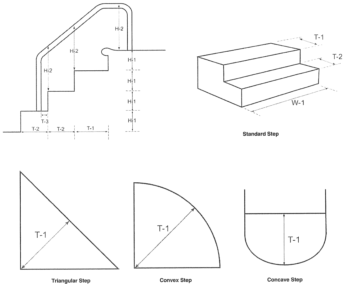
FIGURE 31B-7 STAIR AND HANDRAIL DIMENSIONS
