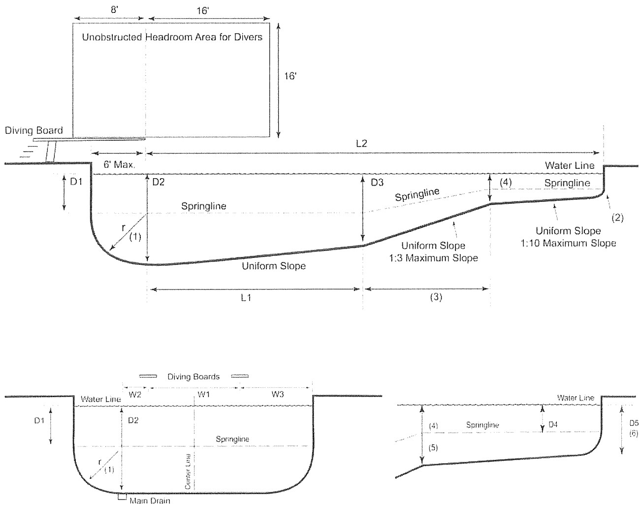
Transverse Section Deep End Through Main Drain
