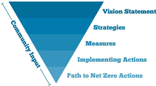
Figure 11 GHG Reduction Framework
