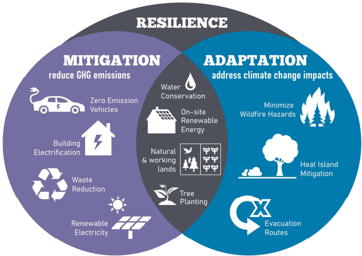
Figure 4 Climate Resilience, Adaptation, and Mitigation
