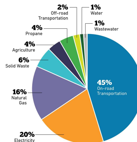
Figure 9 County GHG Emissions by Emissions Category (2019)
