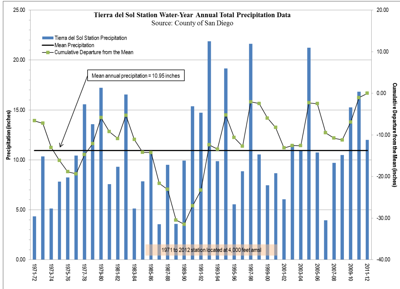
Exhibit 2-B Annual Precipitation Data Tierra del Sol Station 1971 to 2011
