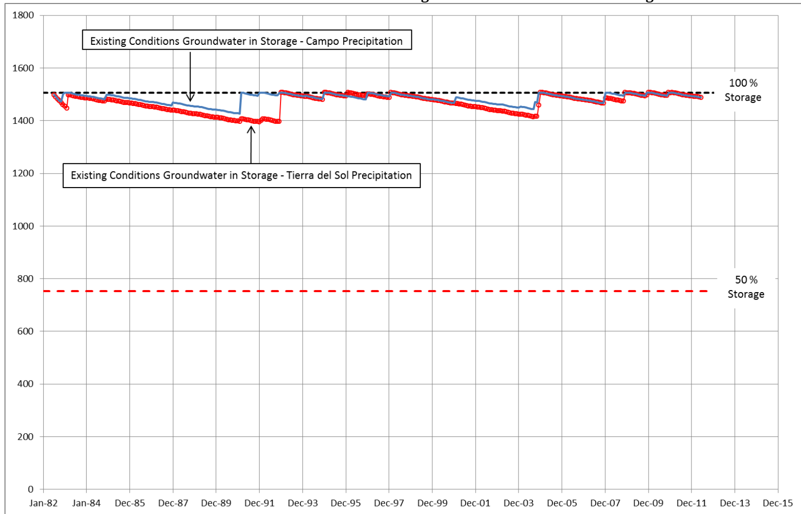
Exhibit 3-A Scenario 1—Well 6a/6b Existing Demand Groundwater in Storage
