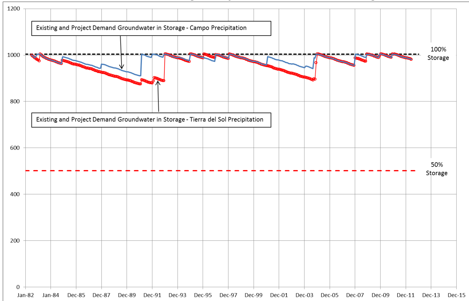
Exhibit 3-E Scenario 2 - Well 8 Existing and Project Demand Groundwater in Storage
