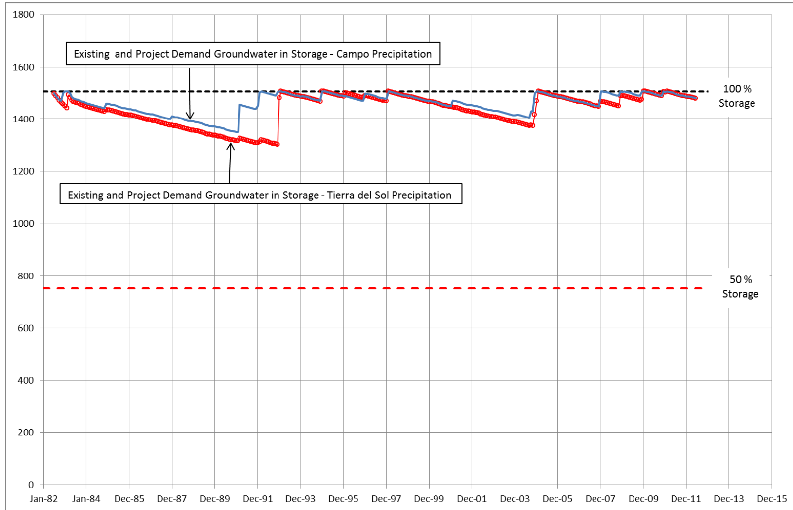
Exhibit 3-B Scenario 2 - Well 6a/6b Existing and Project Demand Groundwater in Storage
