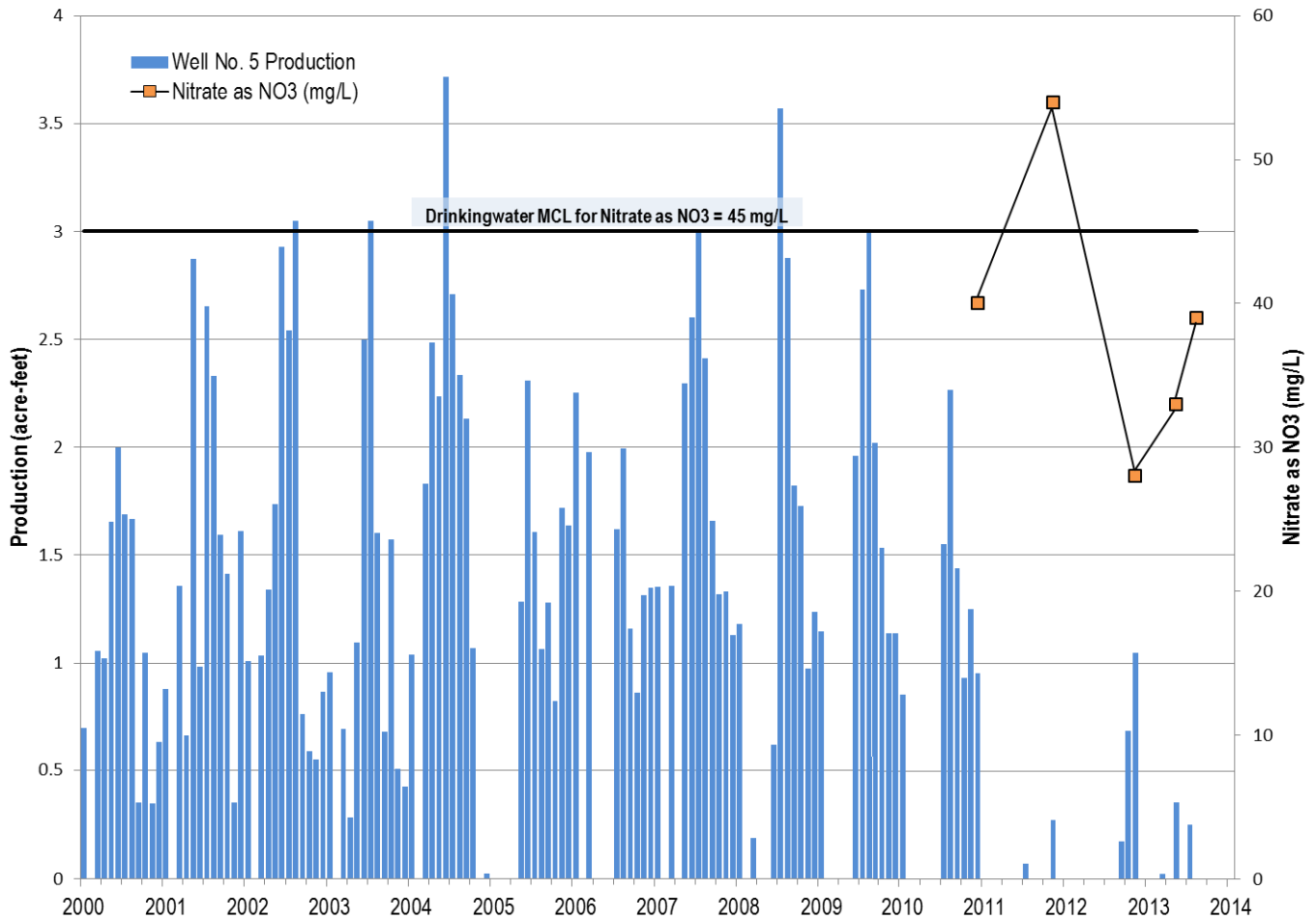
Exhibit 4-A Well No. 5 Production and Nitrate Results
