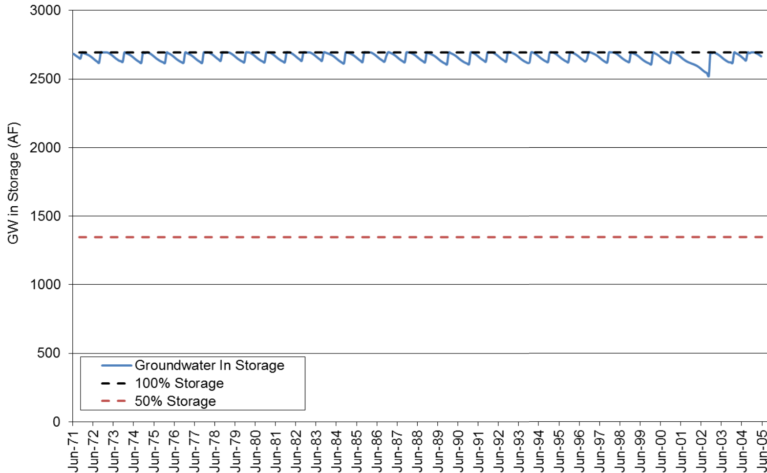
Exhibit 3-B Pine North Basin Scenario 2 – Existing Demand Plus Project Demand
