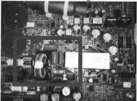
Board Level Filtering and EMI Reduction Layout
