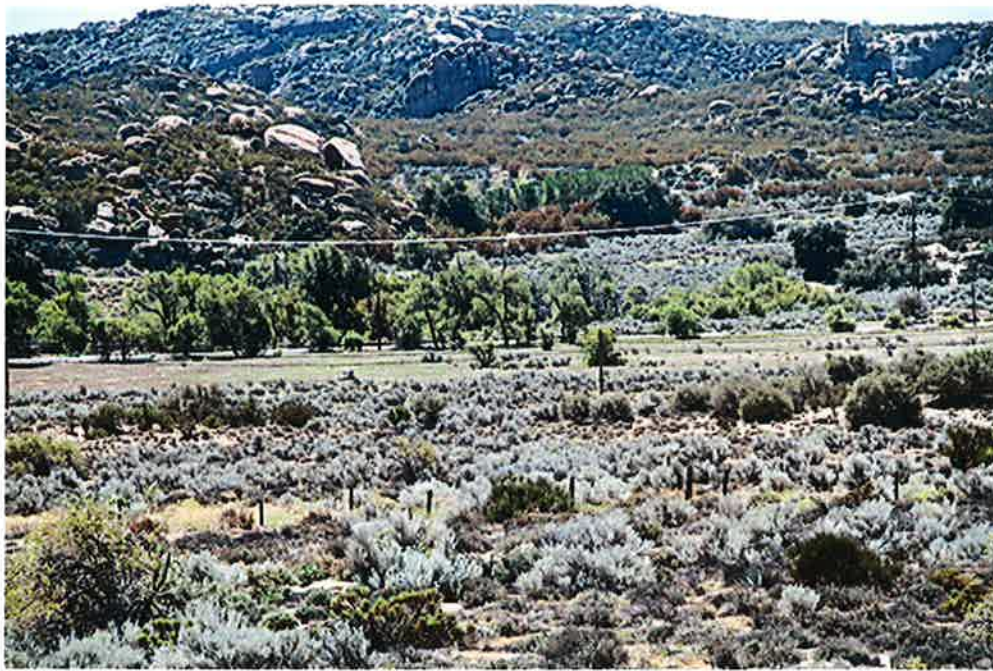
Fig. 46 River willows within the Walker Creek meadow.
