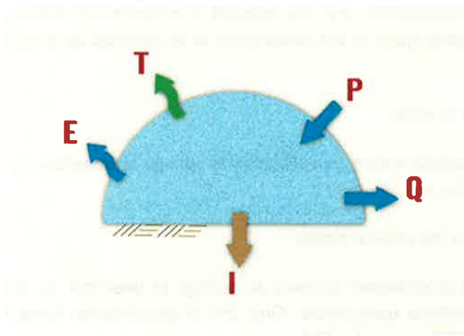
Fig. 18 Components of the water balance.
