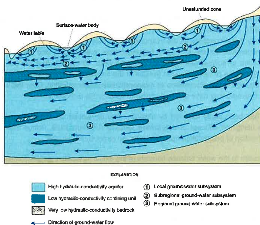
Fig. 17 Typical pattern and direction of groundwater flow
