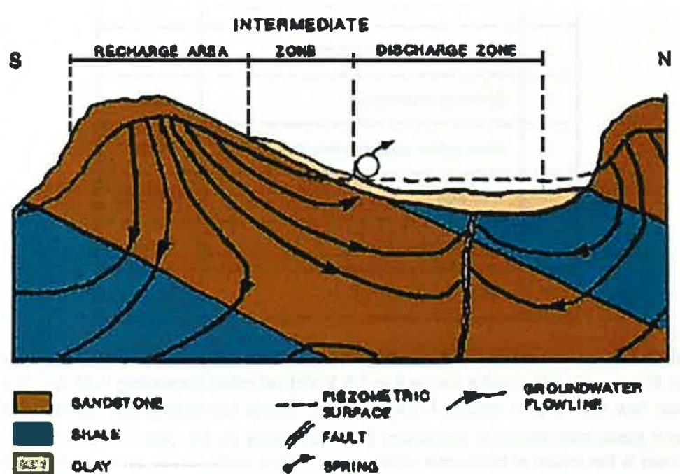
Fig. 20. Recharge to and discharge from groundwater
