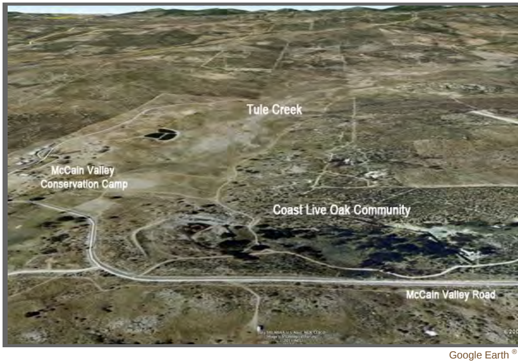
Fig. 27 A community of coast live oak in the foothills of the McCain valley.
