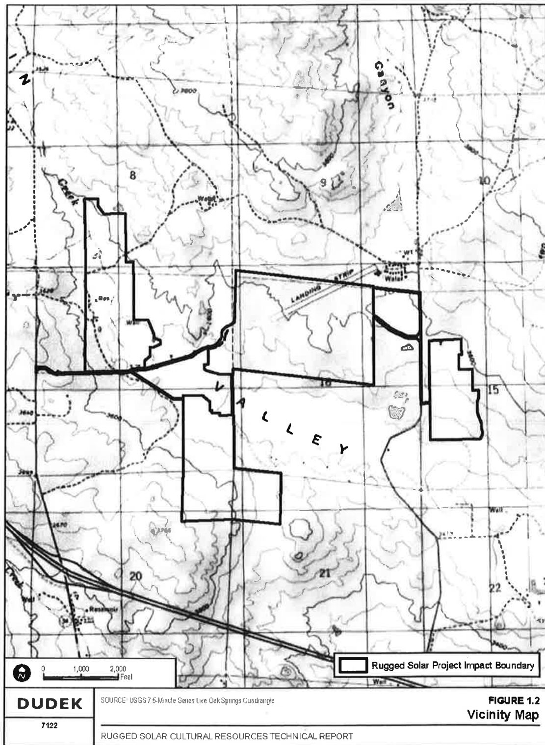
Figure 1.2 Vicinity map
