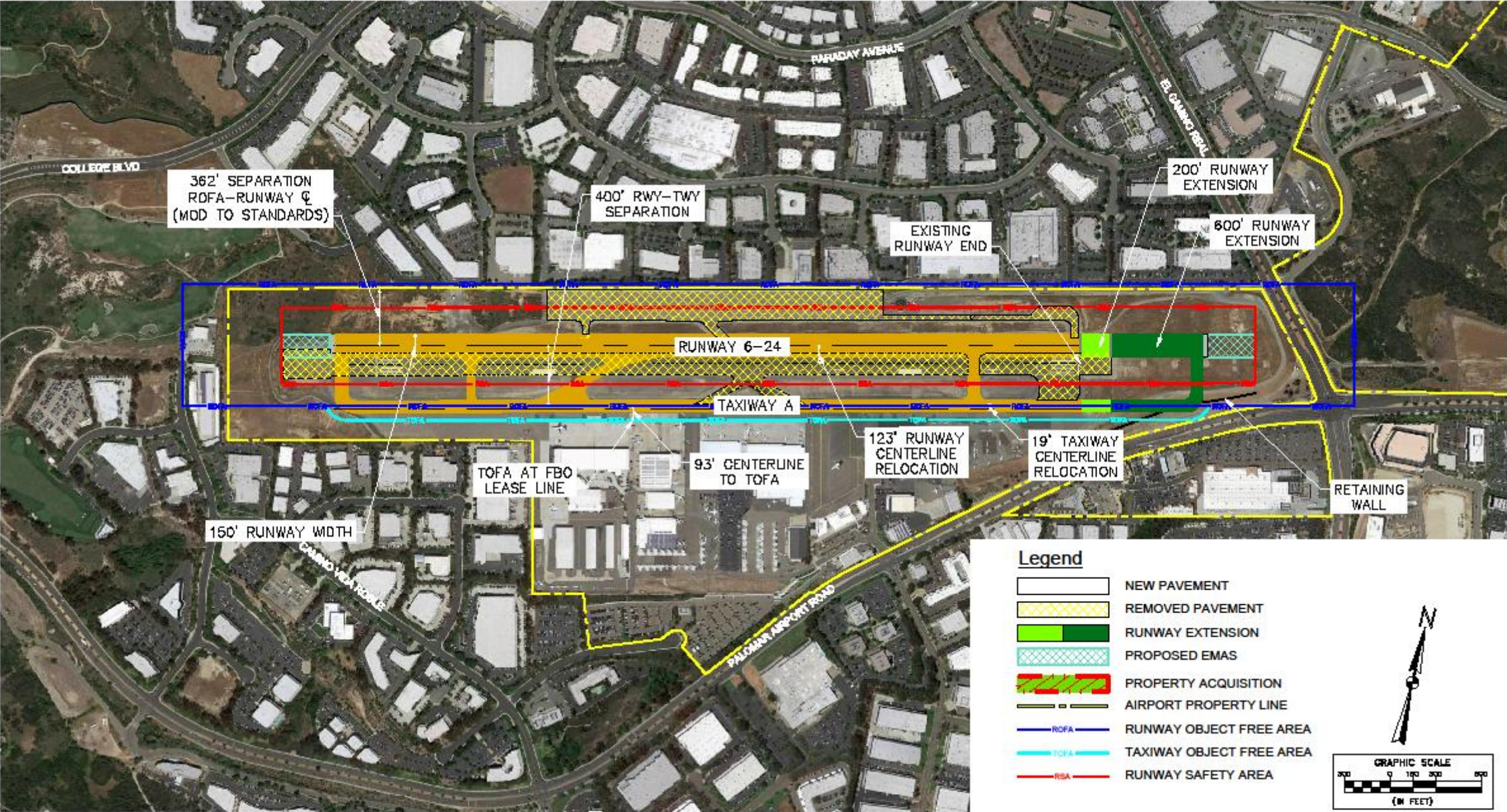
Exhibit 5.7 Airport Alternative 6 – ARC C-III Modified Standards Compliance
