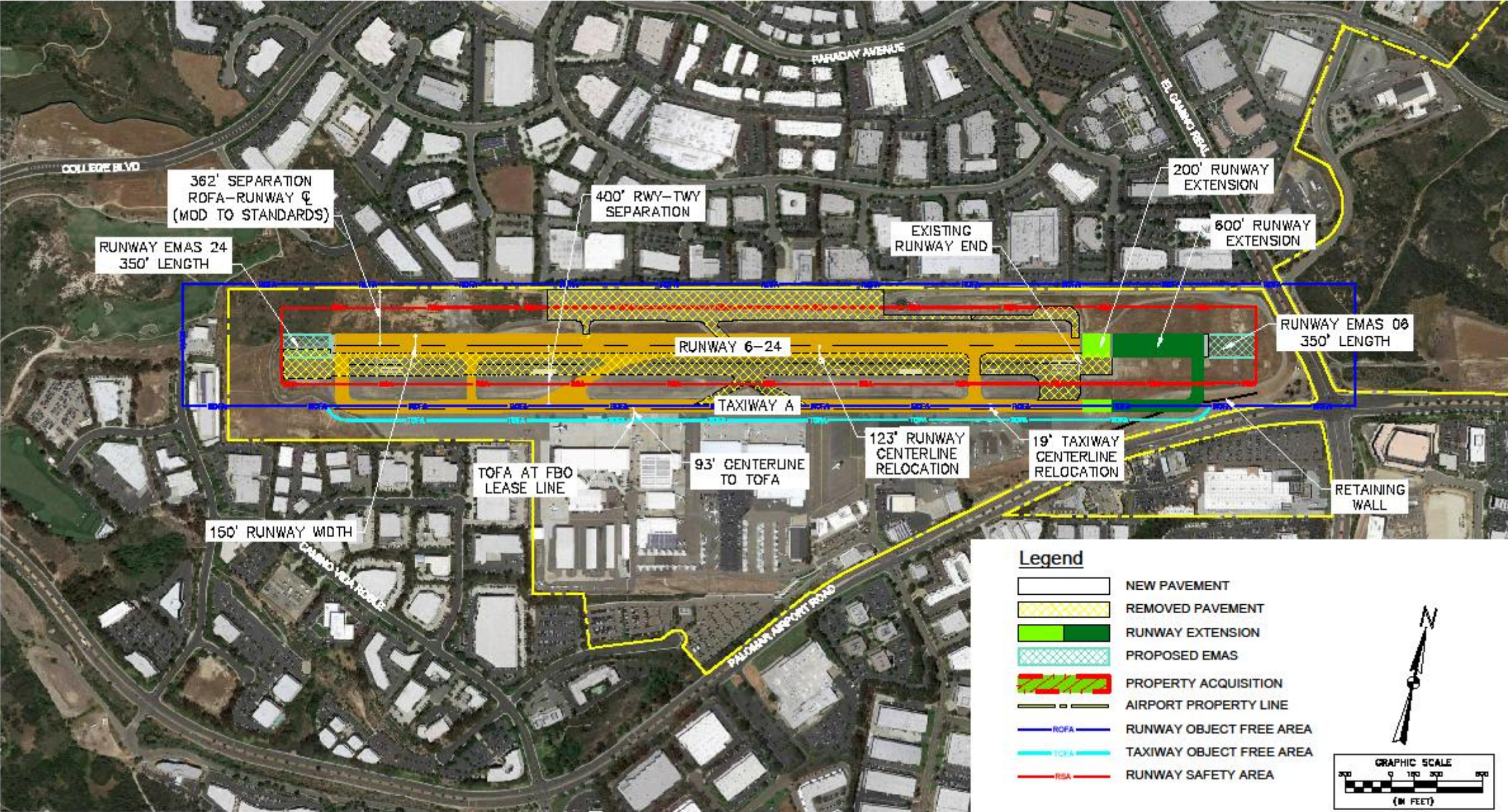
Exhibit 5.6 Airport Alternative 5 – ARC D-III Modified Standards Compliance
