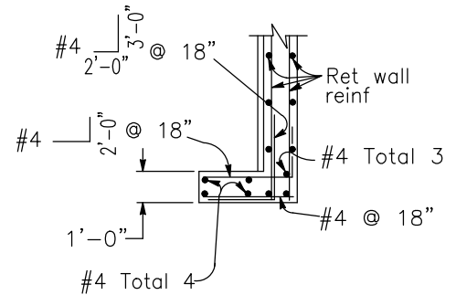
PLAN (For return wall type "D")
