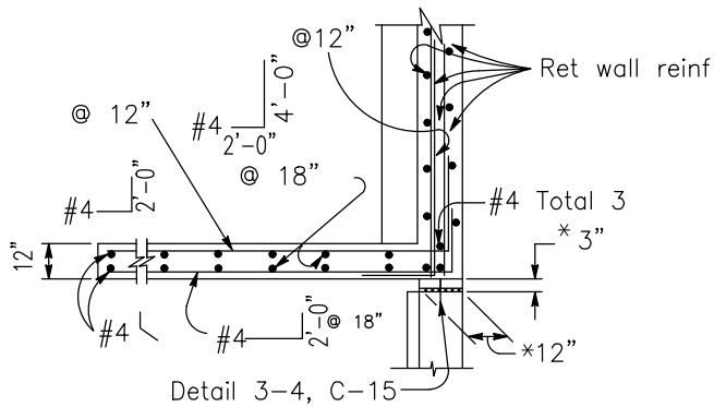
PLAN (For return wall type "B")
