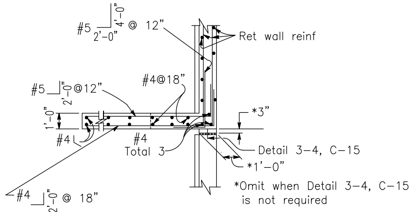
PLAN (For return wall type "A")
