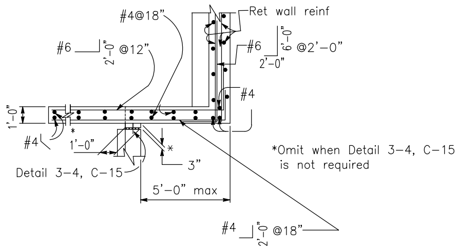
PLAN (For return wall type "B")
