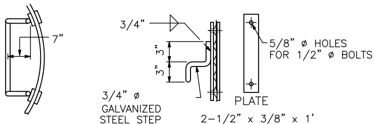
STEP DETAIL H=3'-6" TO 4'-11"
