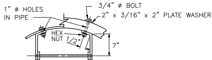
LADDER DETAIL H=5' OR GREATER
