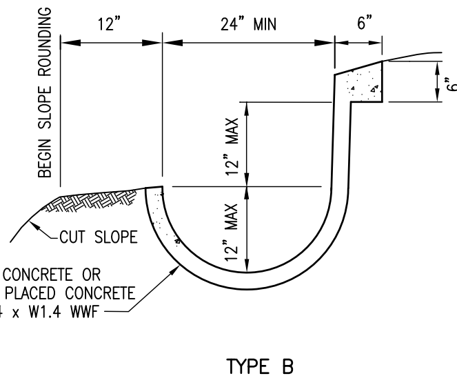
BROW DITCH
