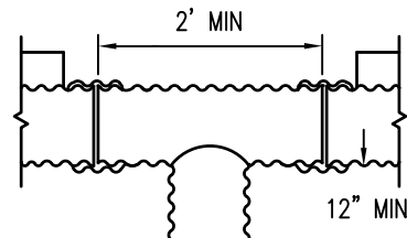
TEE-SAG CONDITION
