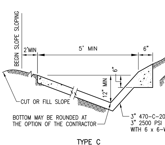
TERRACE DITCH
