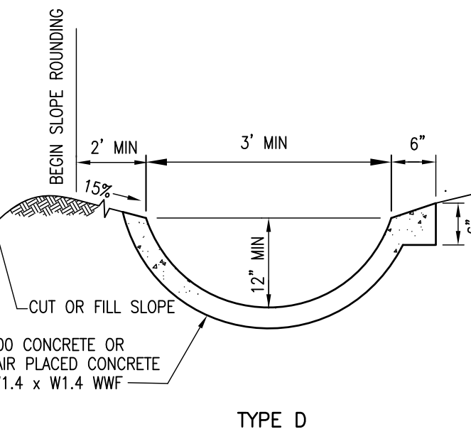
TERRACE DITCH
