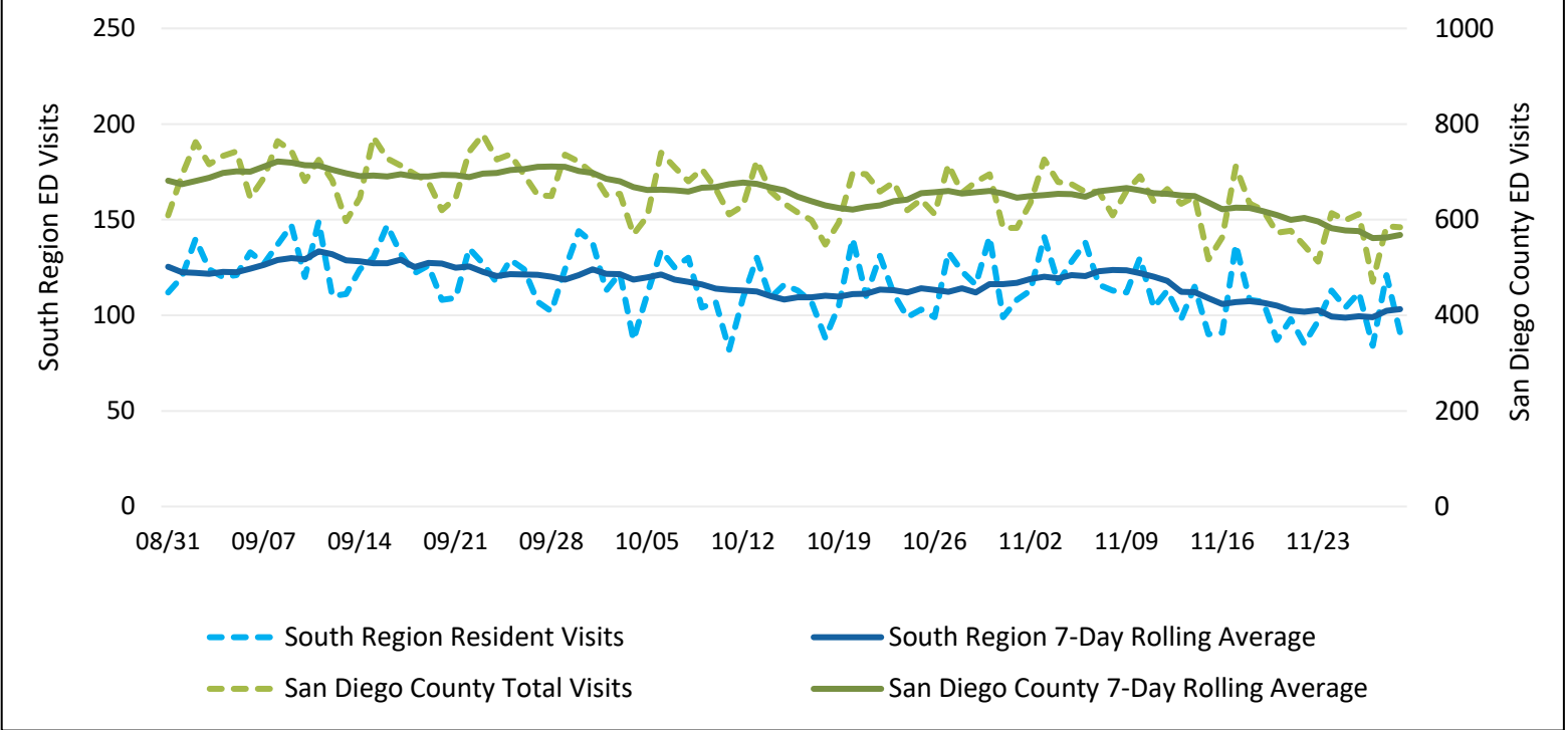
Figure 1. Gastrointestinal Symptoms Emergency Department Visits, San Diego County, Previous 3 Months
