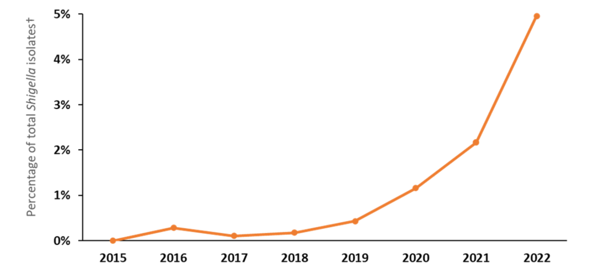
Figure: Percentage of Shigella isolates that showed an extensively drug resistant (XDR)* phenotype or genotype in the United States, by year, 2015–2022†
