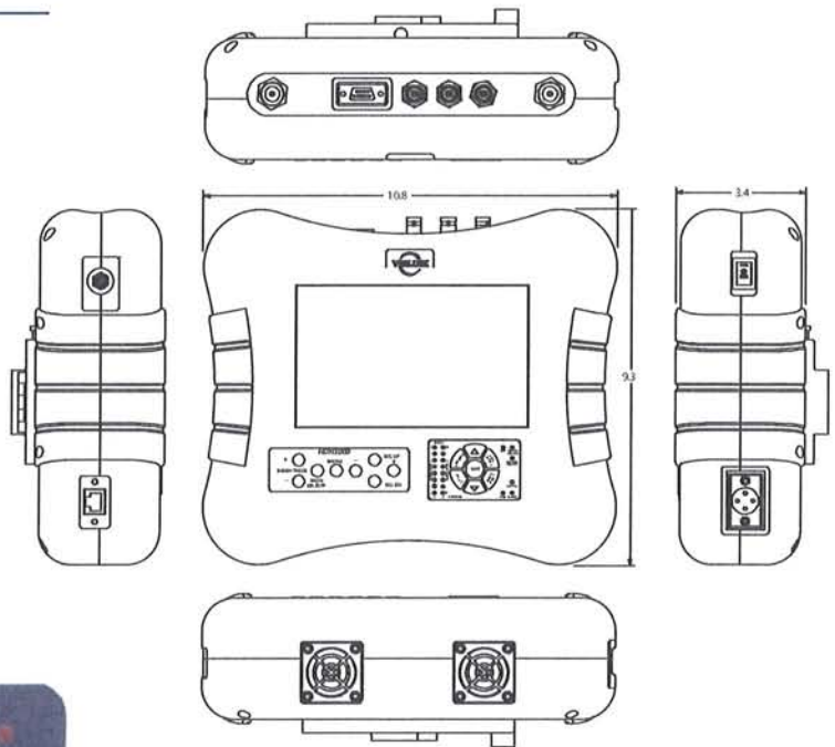
HDH-1000 Dimensions
