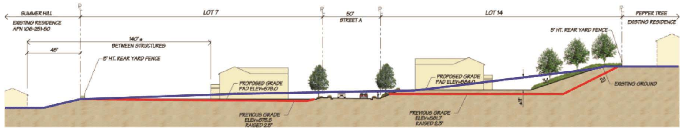
SECTION B-B
