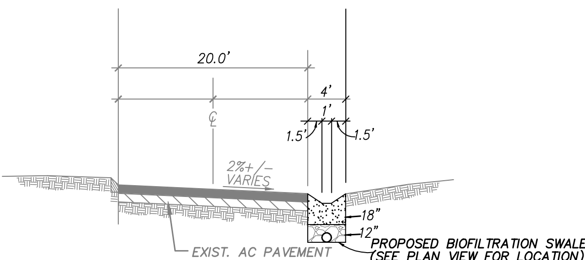
ORO VERDE ROAD PROPOSED PRIVATE ROAD EASEMENT 25 MPH DESIGN SPEED
