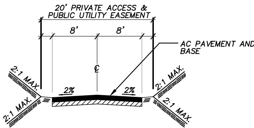
PROPOSED PRIVATE DRIVEWAY LOTS 1, PORTION OF 2 & 3, & 6-10 25 MPH DESIGN SPEED
