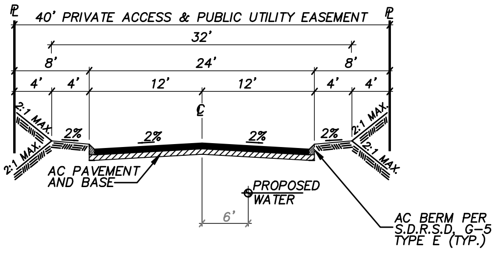
PRIVATE ROAD "A" PROPOSED PRIVATE ROAD 25 MPH DESIGN SPEED
