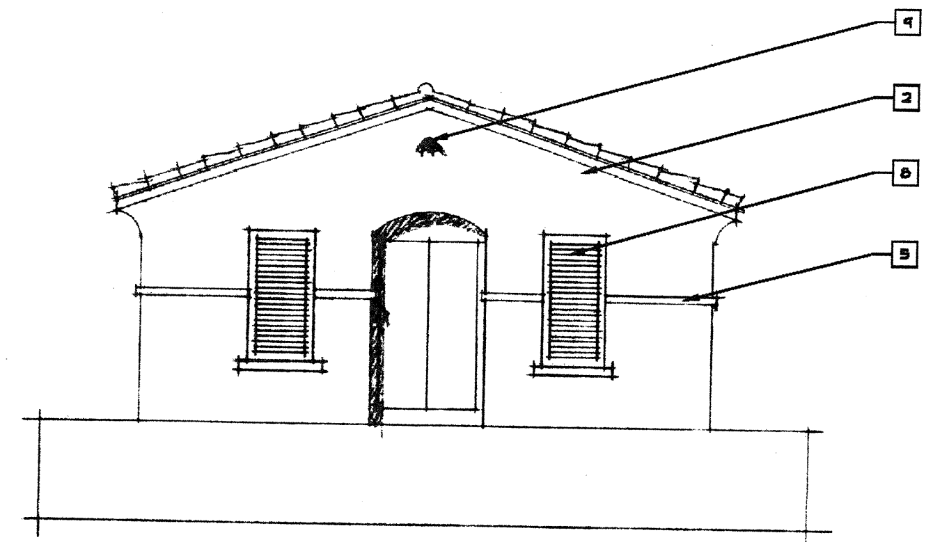
REAR ELEVATION
