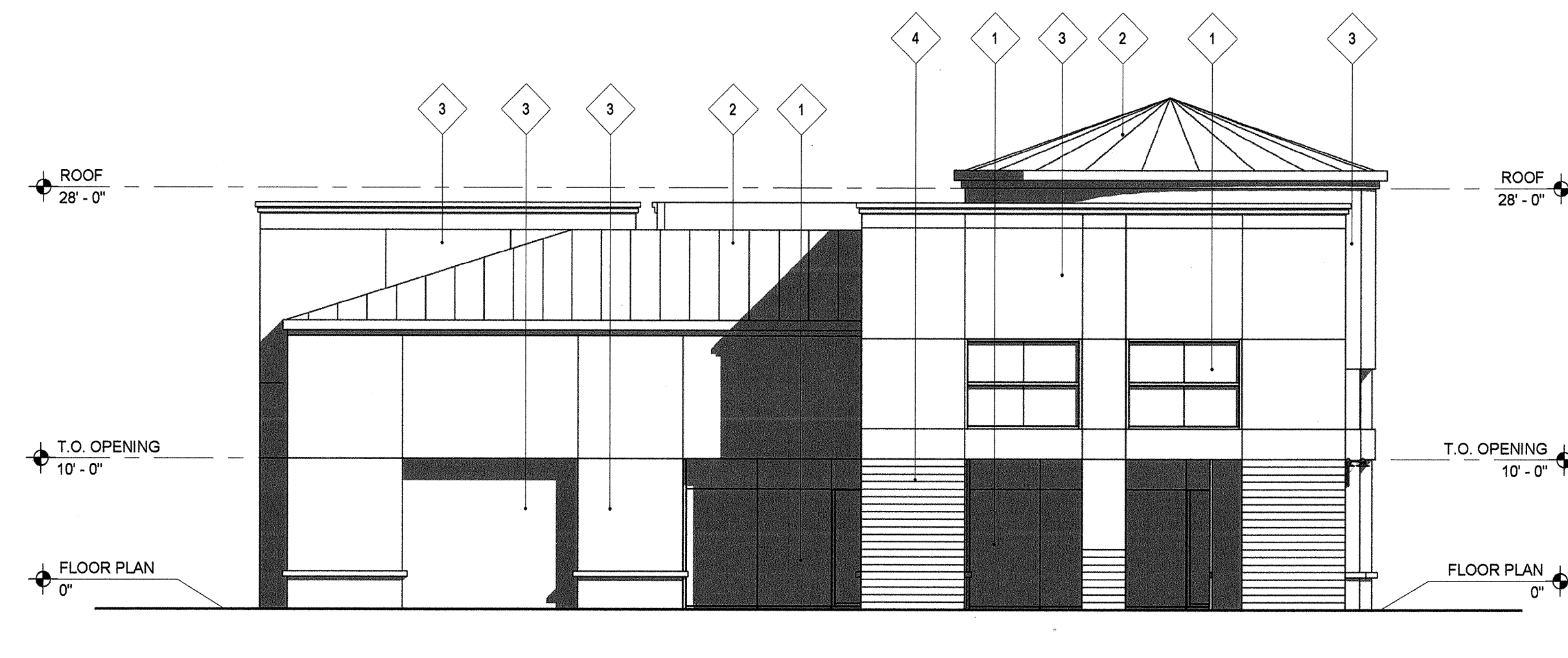
2 BLDG D - SOUTH ELEVATION 1/8" = 1'-0"
