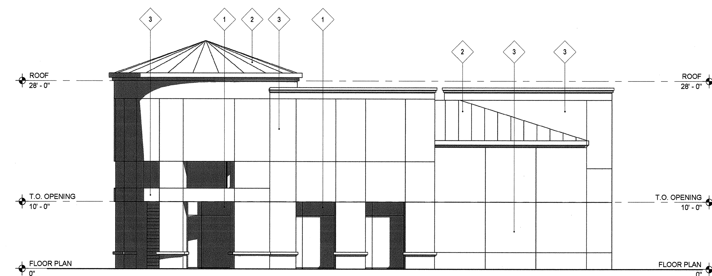
4 BLDG D - NORTH ELEVATION 1/8" = 1'-0"
