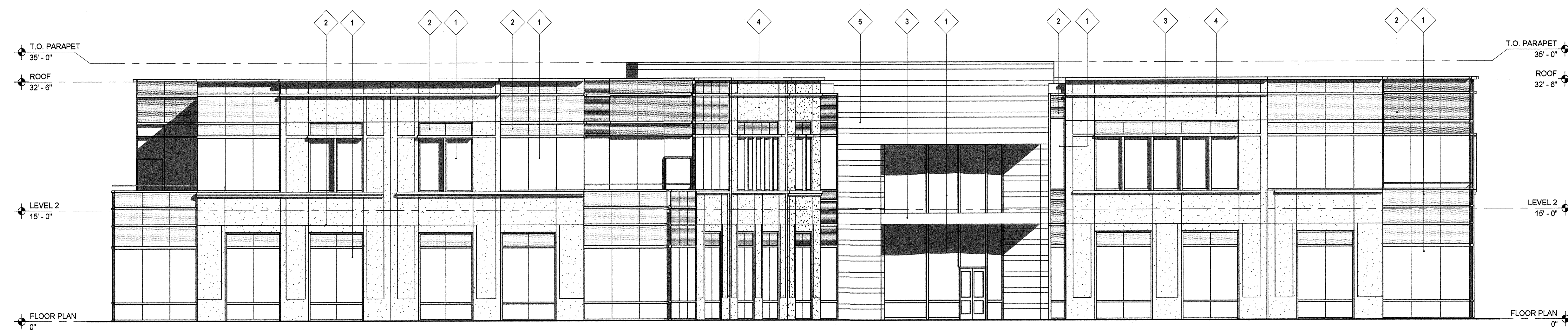
1 BUILDING A - EAST ELEVATION 1/8" = 1'-0"
