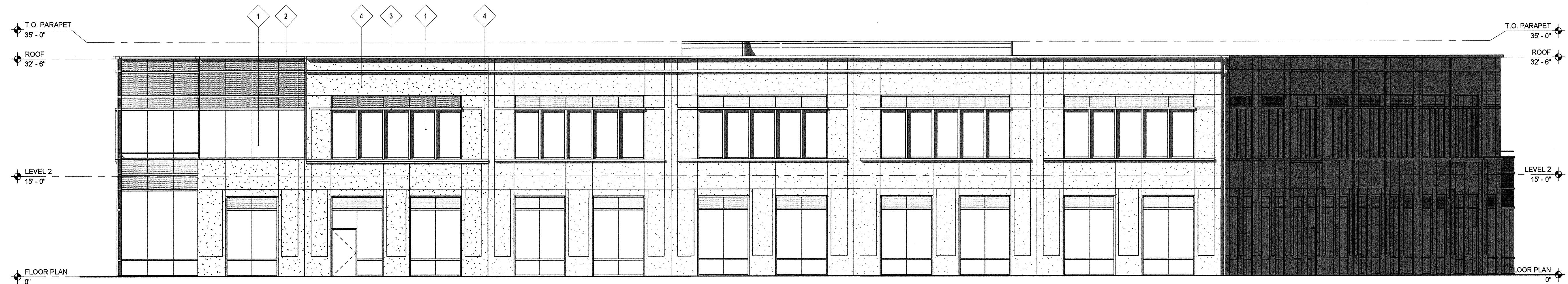
2 BLDG B - EAST ELEVATION 1/8" = 1'-0"
