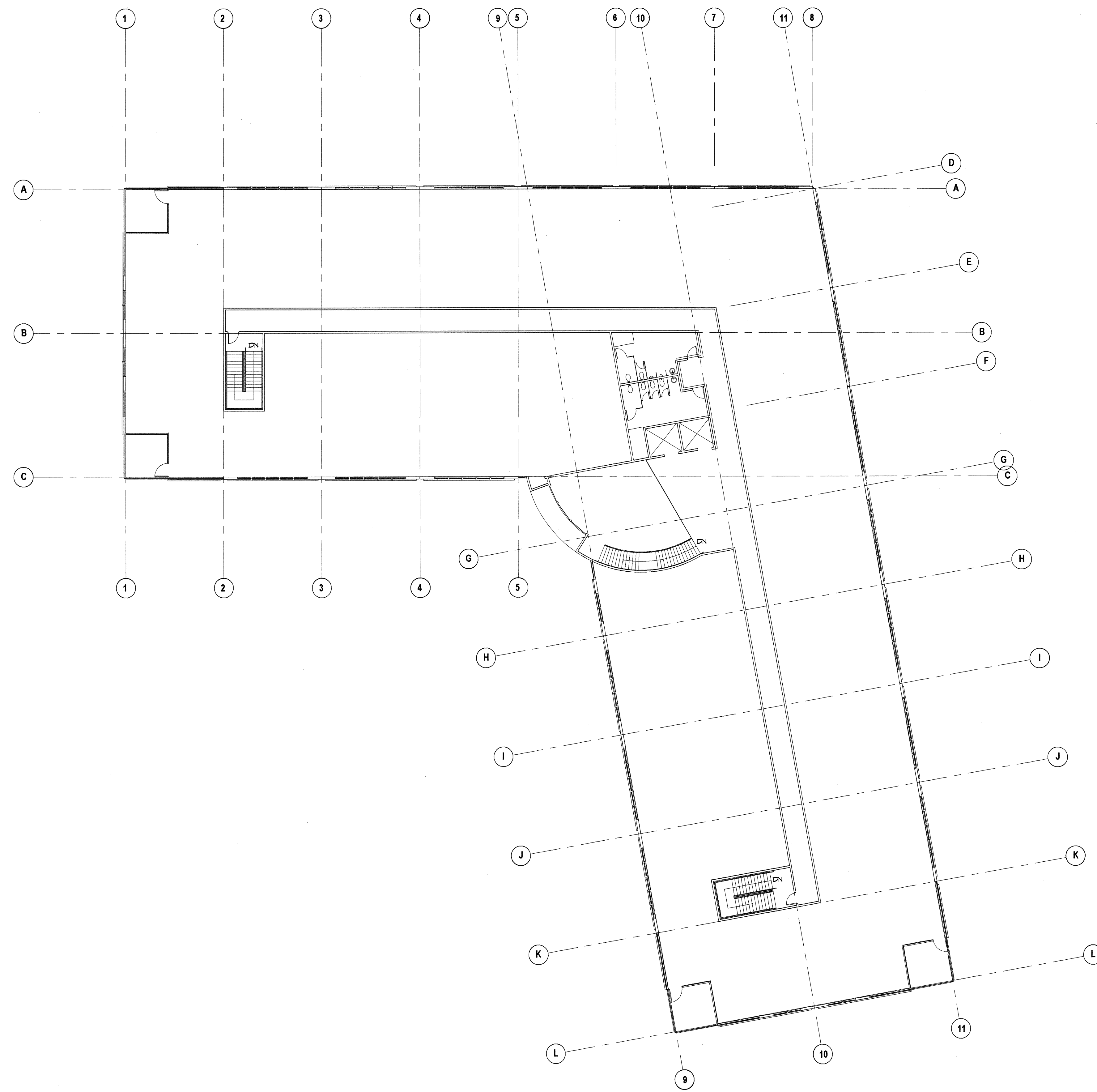
2 BUILDING C - FLOOR PLAN - LEVEL 2 1/16" = 1'-0"
