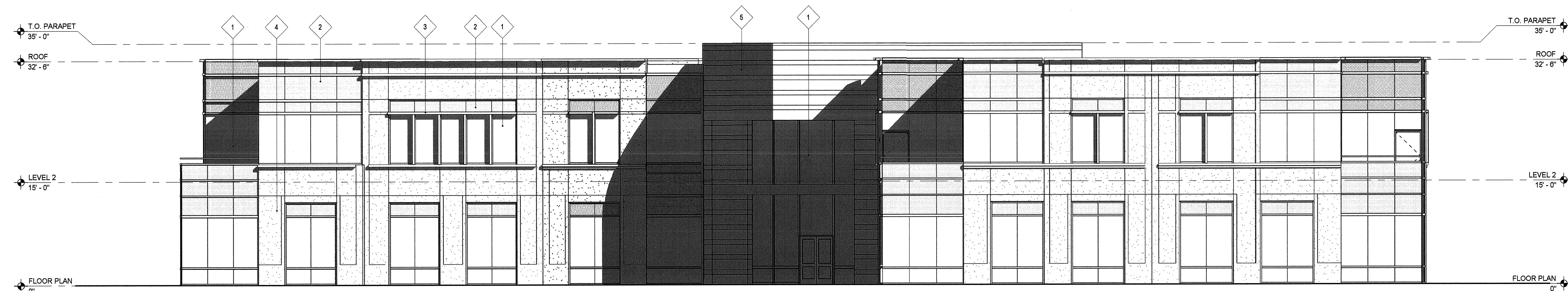
4 BUILDING A - NORTH ELEVATION 1/8" = 1'-0"
