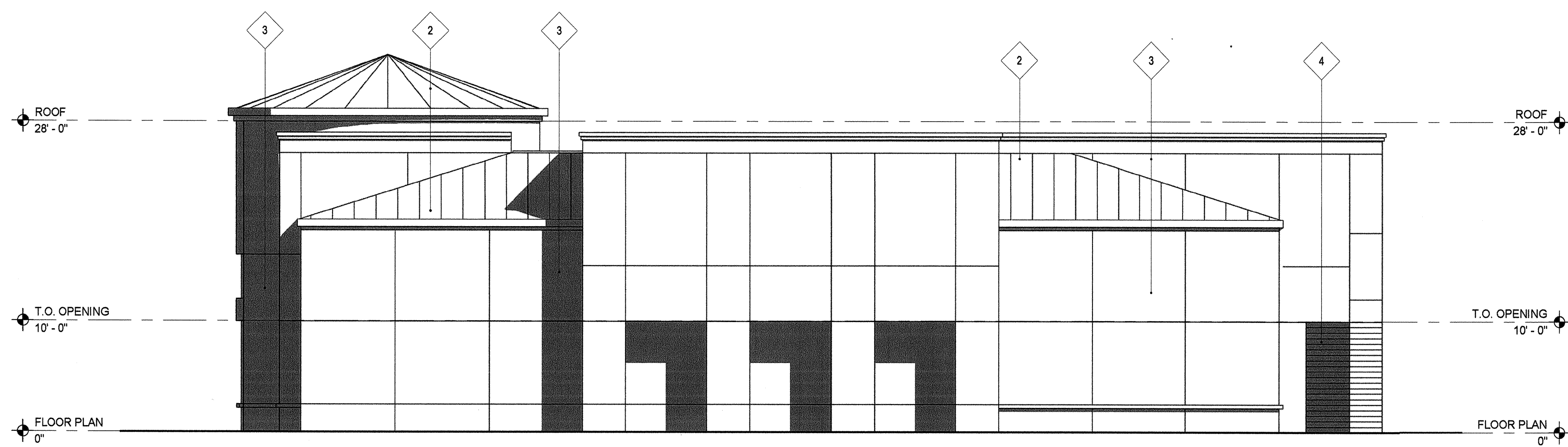
3 BLDG D - WEST ELEVATION 1/8" = 1'-0"
