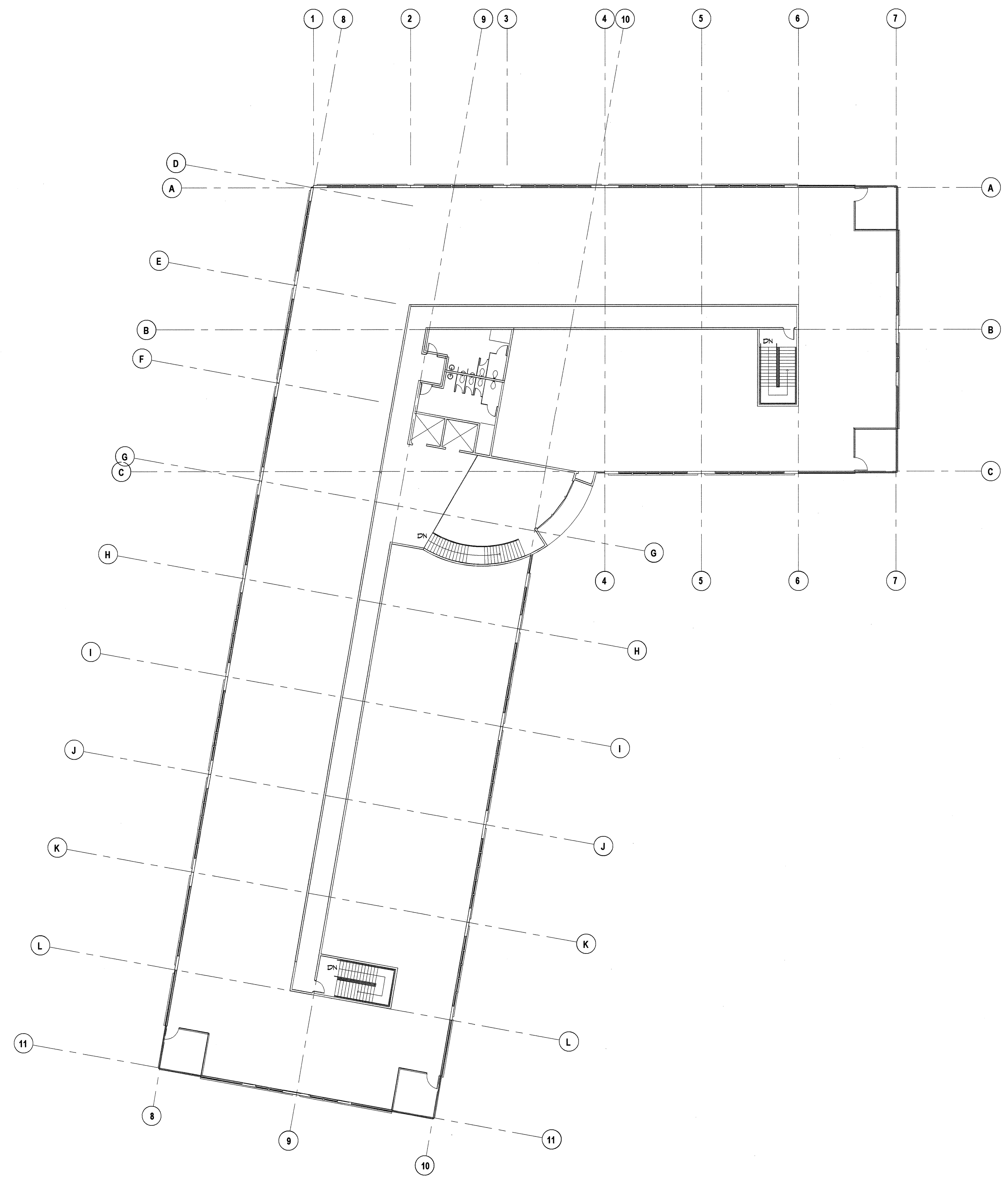
2 BUILDING B - FLOOR PLAN - LEVEL 2 1/16" = 1'-0"
