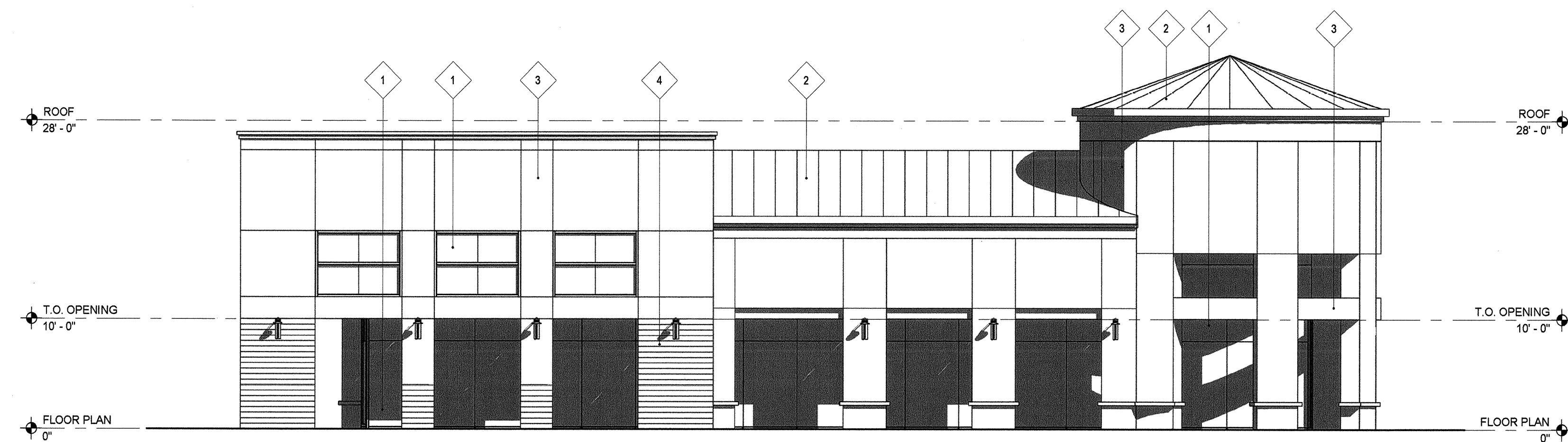
1 BLDG D - EAST ELEVATION 1/8" = 1'-0"
