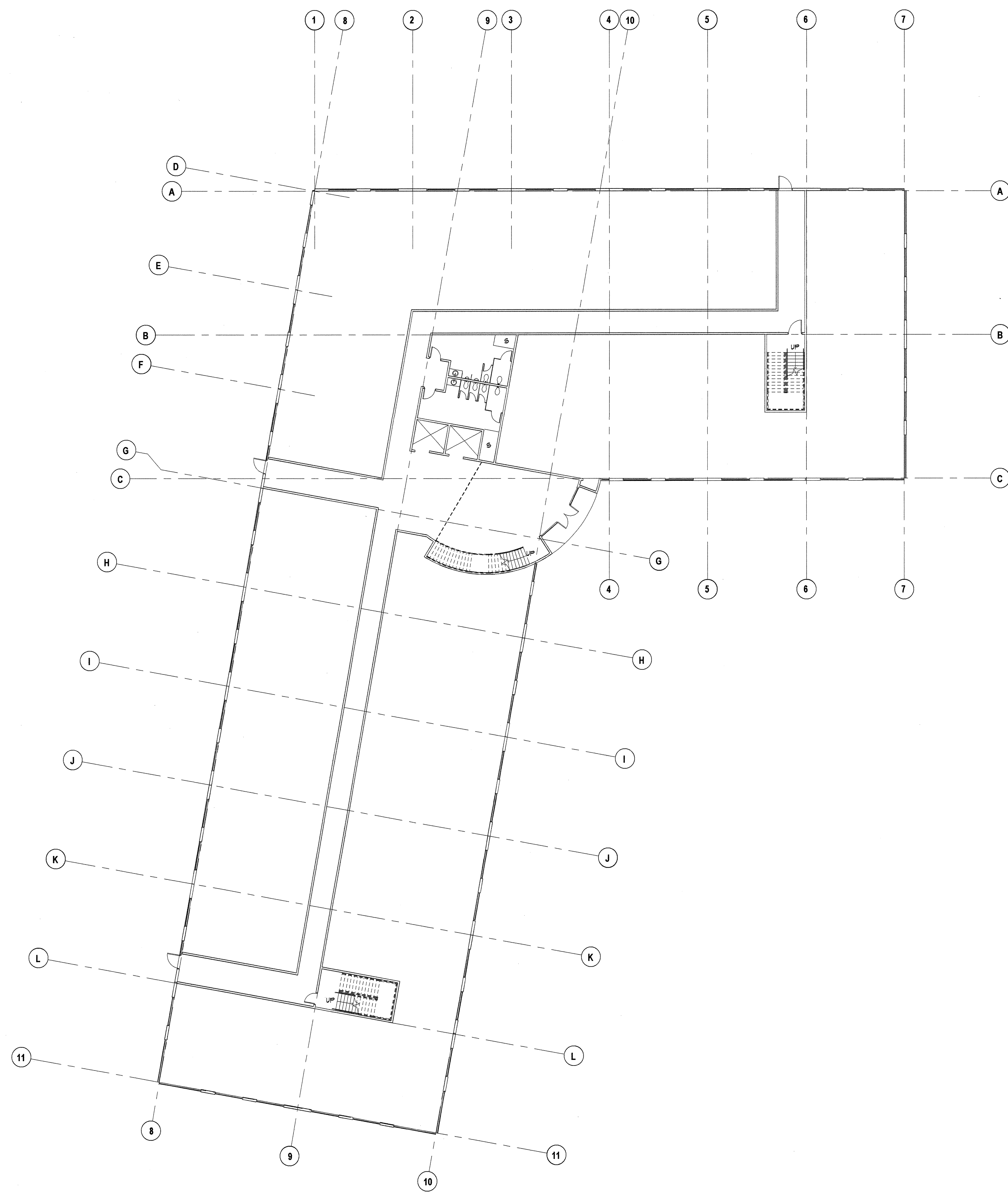
1 BUILDING B - FLOOR PLAN - LEVEL 1 1/16" = 1'-0"
