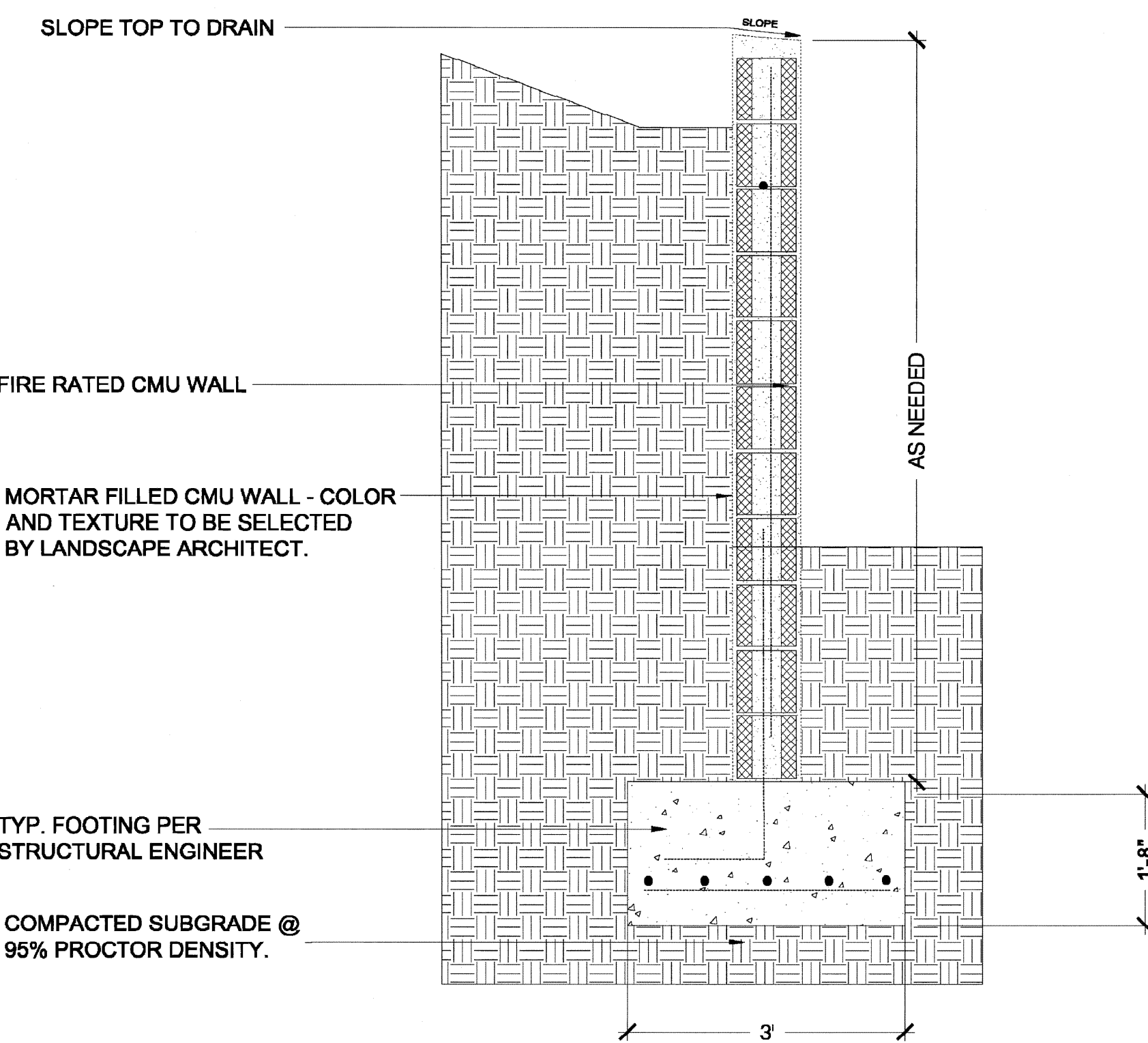
RETAINING CMU BLOCK WALL
