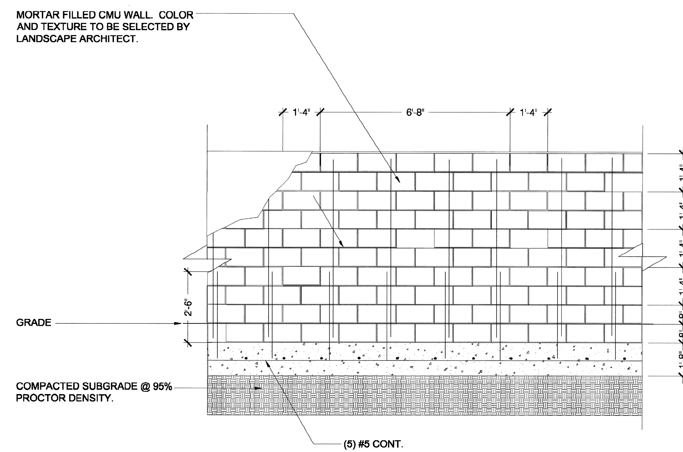
CMU BLOCK SOUND BARRIER
