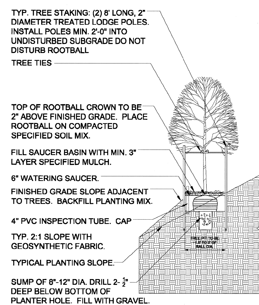
SECTION-TREE PLANTING ON SLOPE
