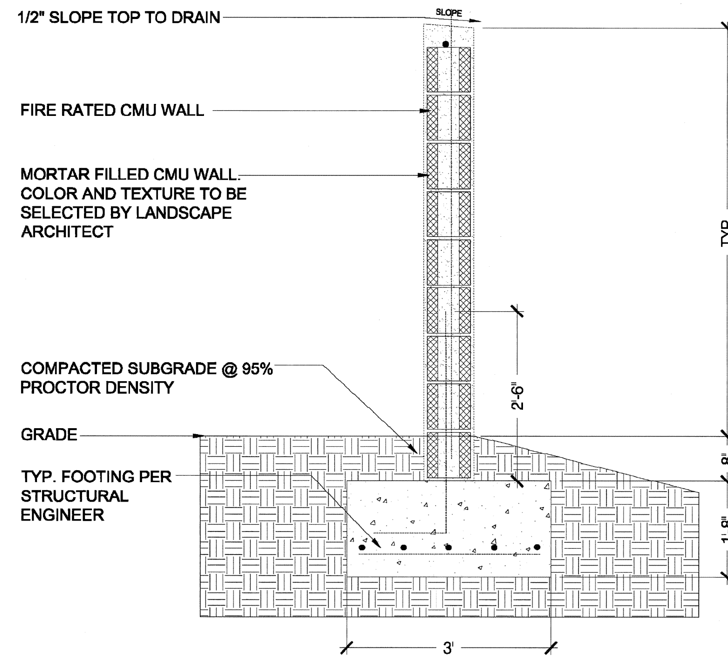
CMU BLOCK SOUND WALL
