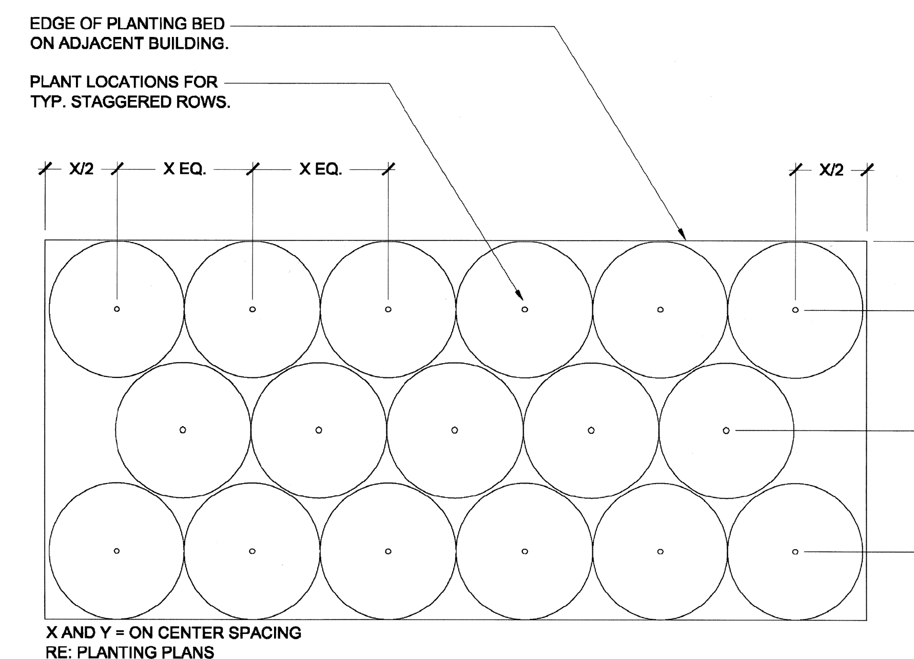
PLAN-SHRUB/GROUNDCOVER SPACING
