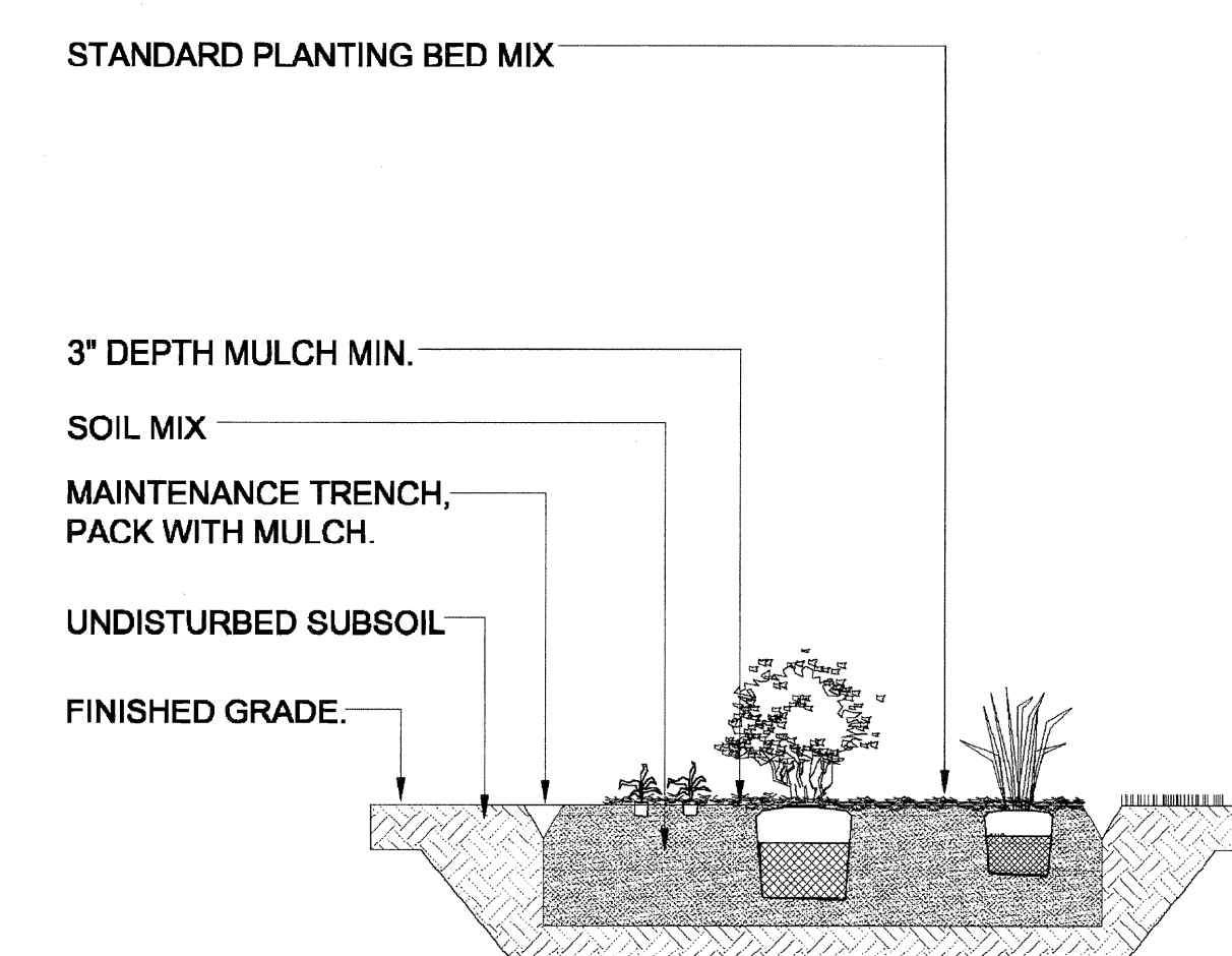
SECTION-SHRUB/GROUNDCOVER PLANTING
