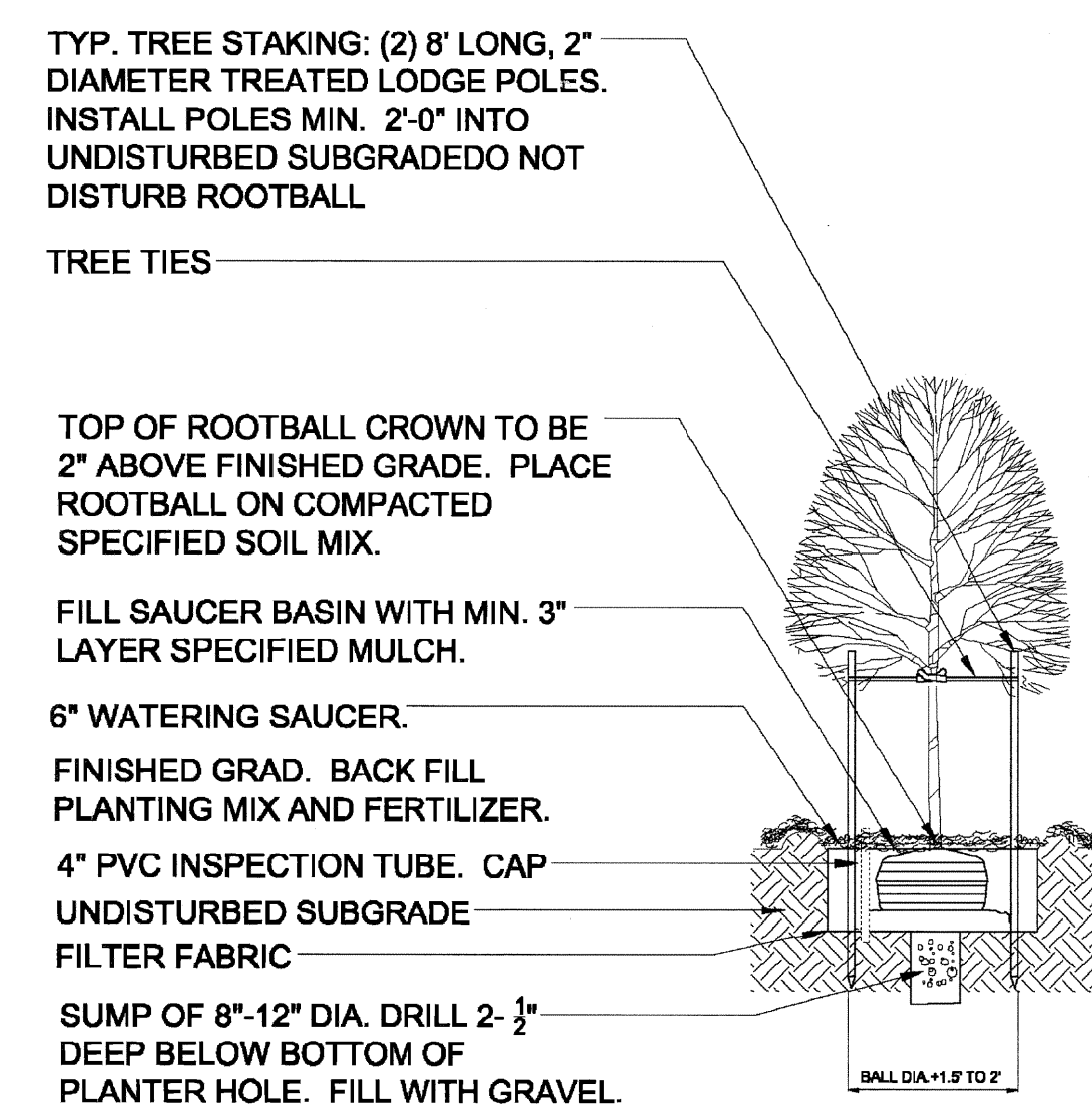
SECTION-TREE PLANTING
