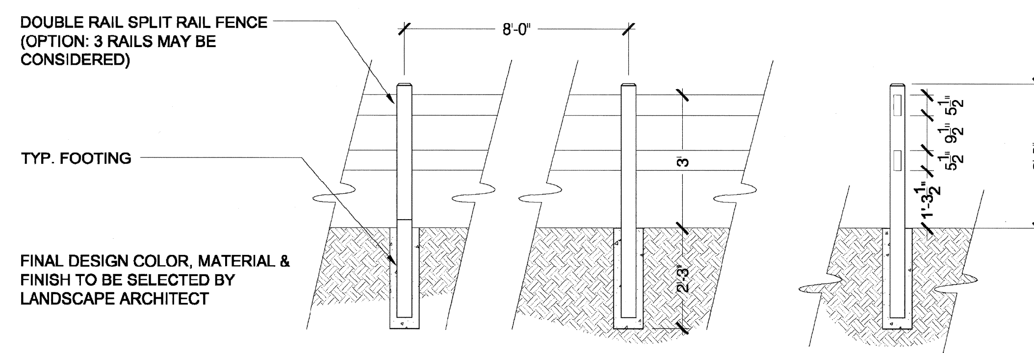
SECTION/ELEVATION-SPLIT RAIL FENCE
