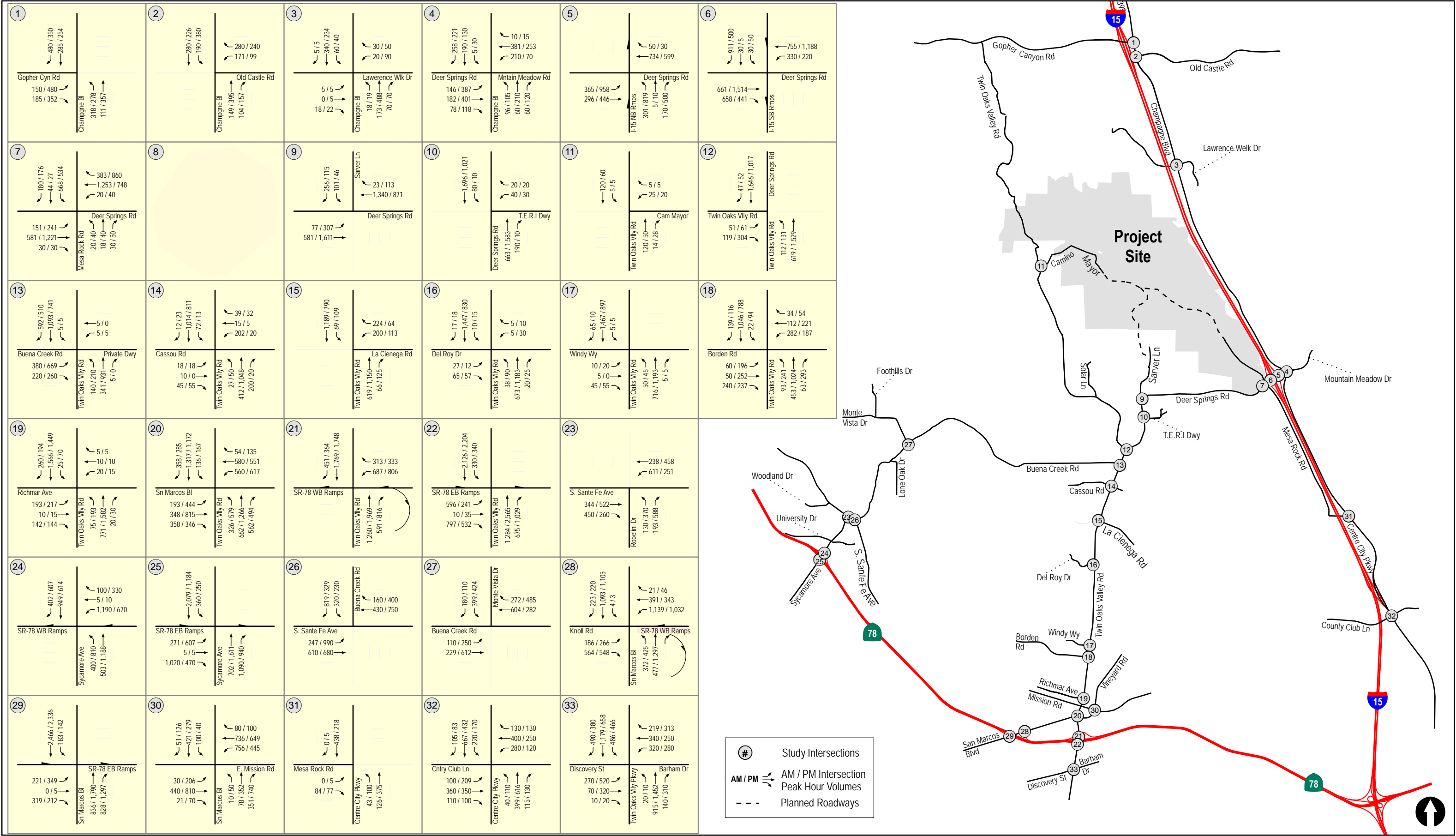
Figure 9-6 Existing + Project + Cumulative Projects AM / PM Peak Hour Traffic Volumes
