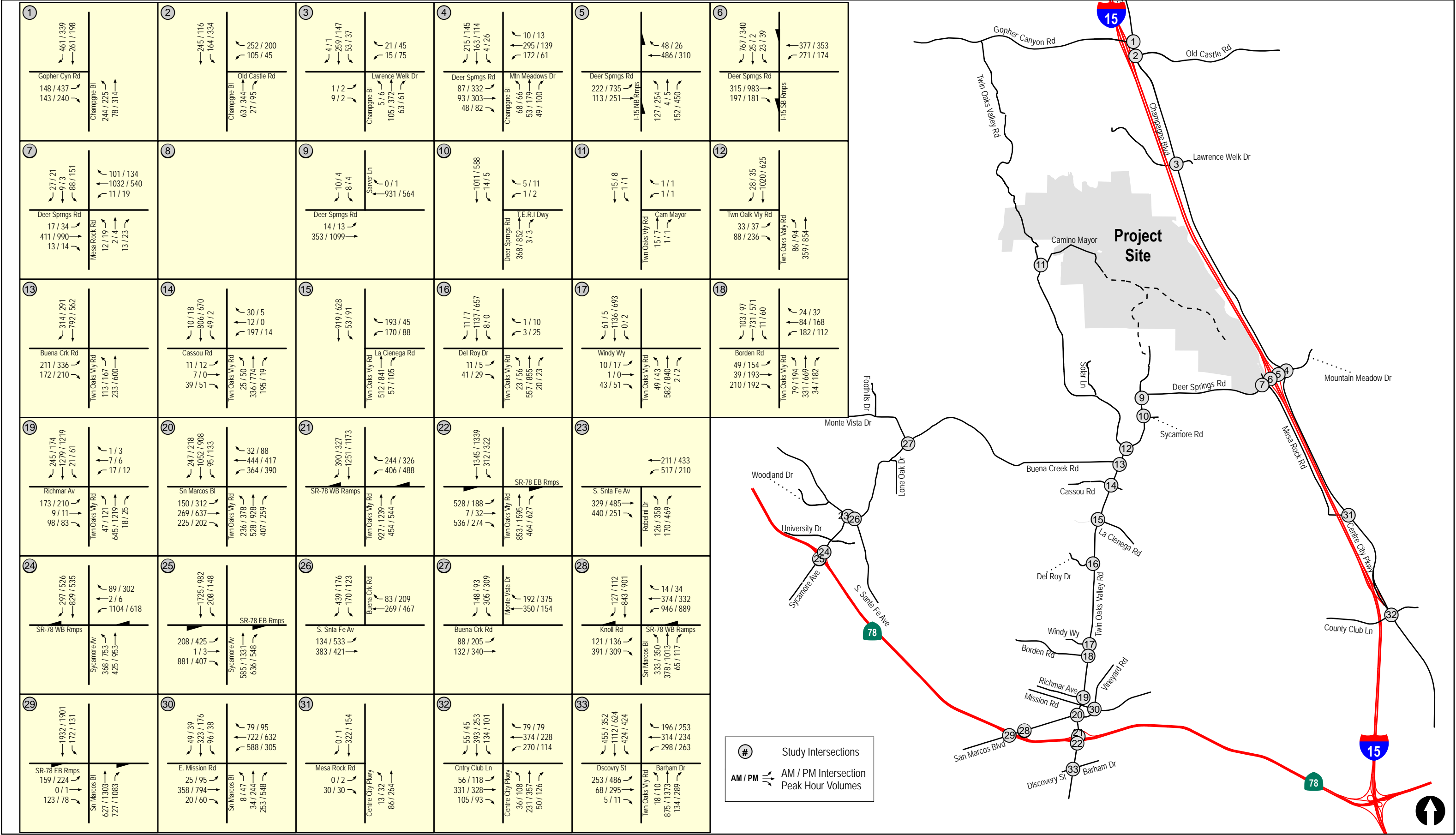
Figure 4-3 Existing AM / PM Peak Hour Traffic Volumes
