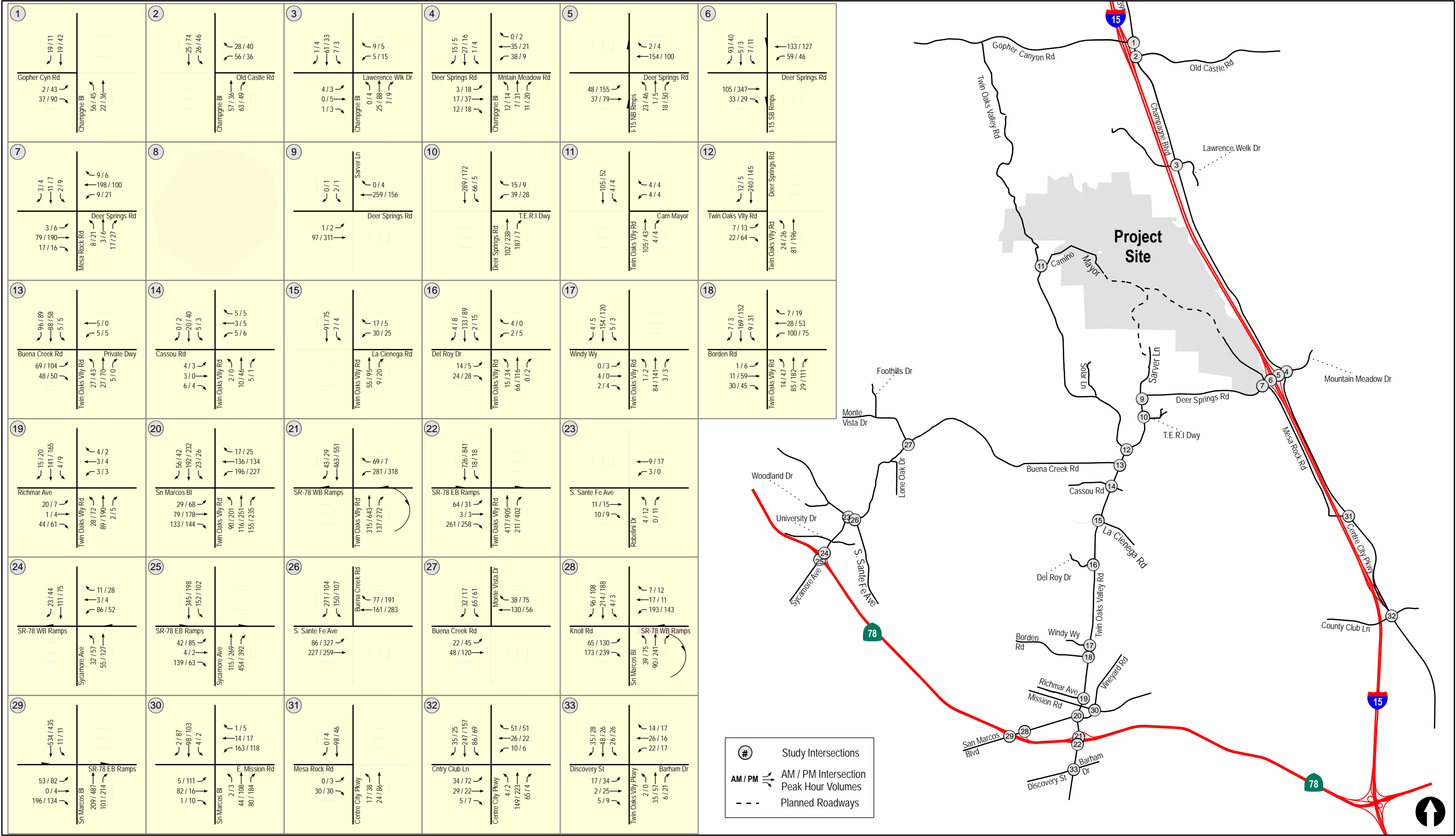
Figure 9-2 Cumulative Projects AM / PM Peak Hour Traffic Volumes
