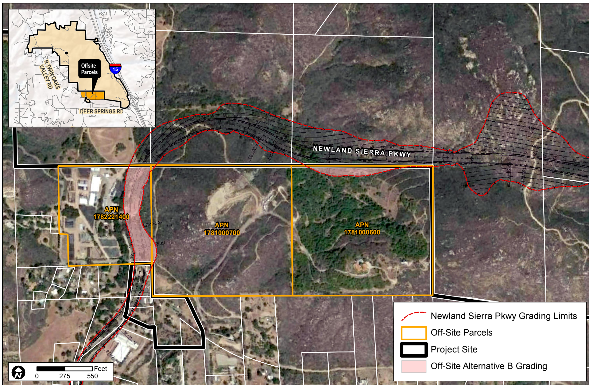
FIGURE 4-6 Newland Sierra Parkway Alternative B - Impacts to Off-Site Parcels
