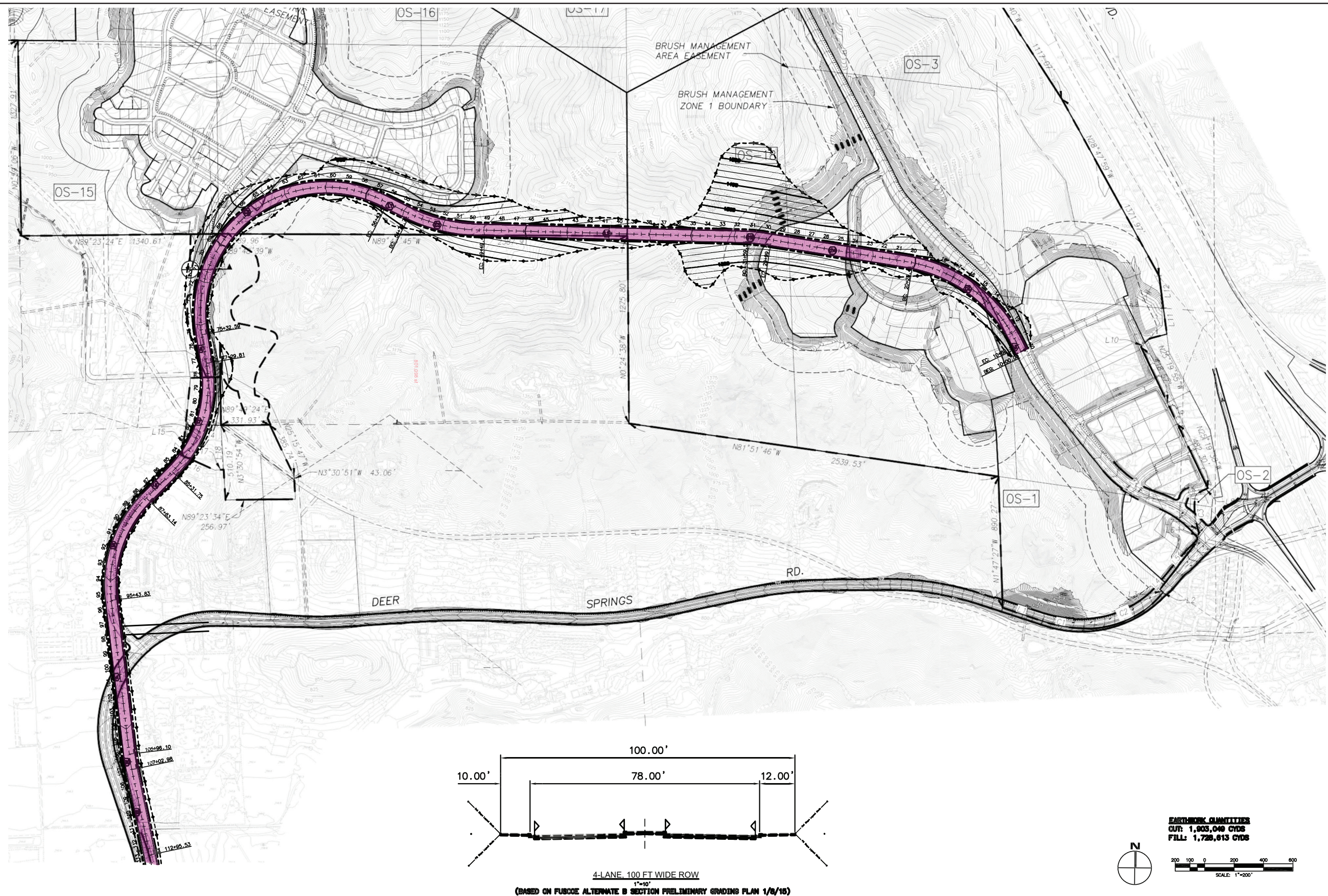
FIGURE 4-5 Newland Sierra Parkway Alternative B
