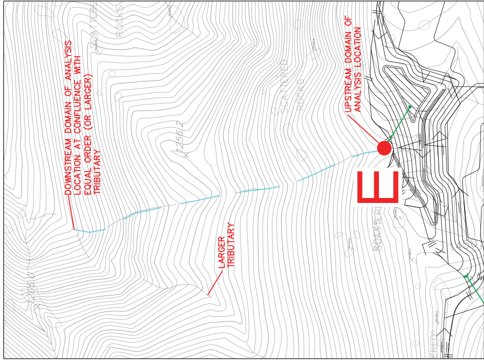
DETAIL - REACH 5 SCALE 1"=120'
