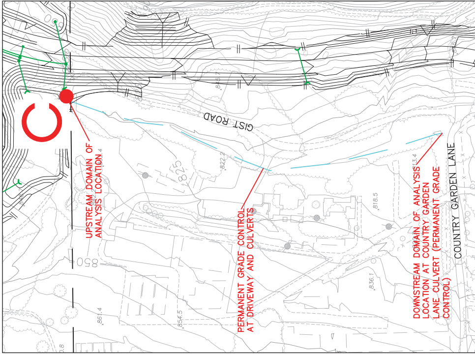
DETAIL - REACH 3 SCALE 1"=120'
