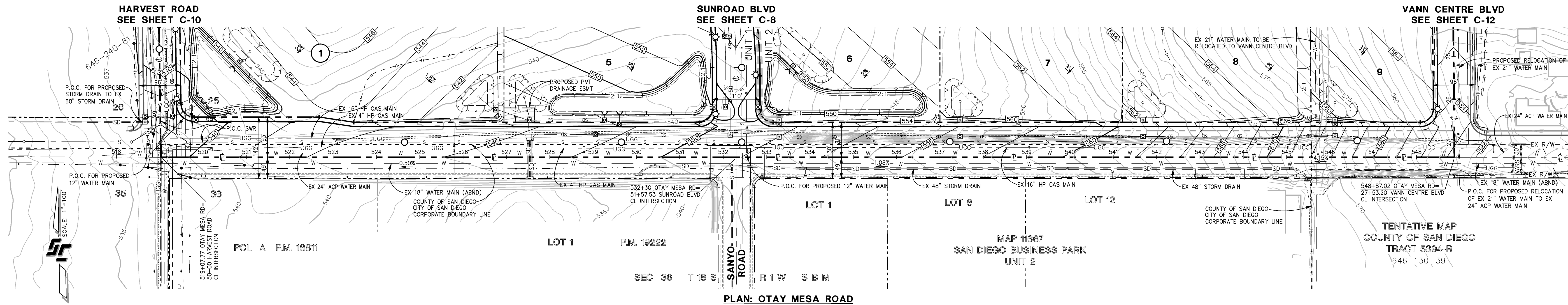
PLAN: OTAY MESA ROAD SCALE: 1"= 100'
