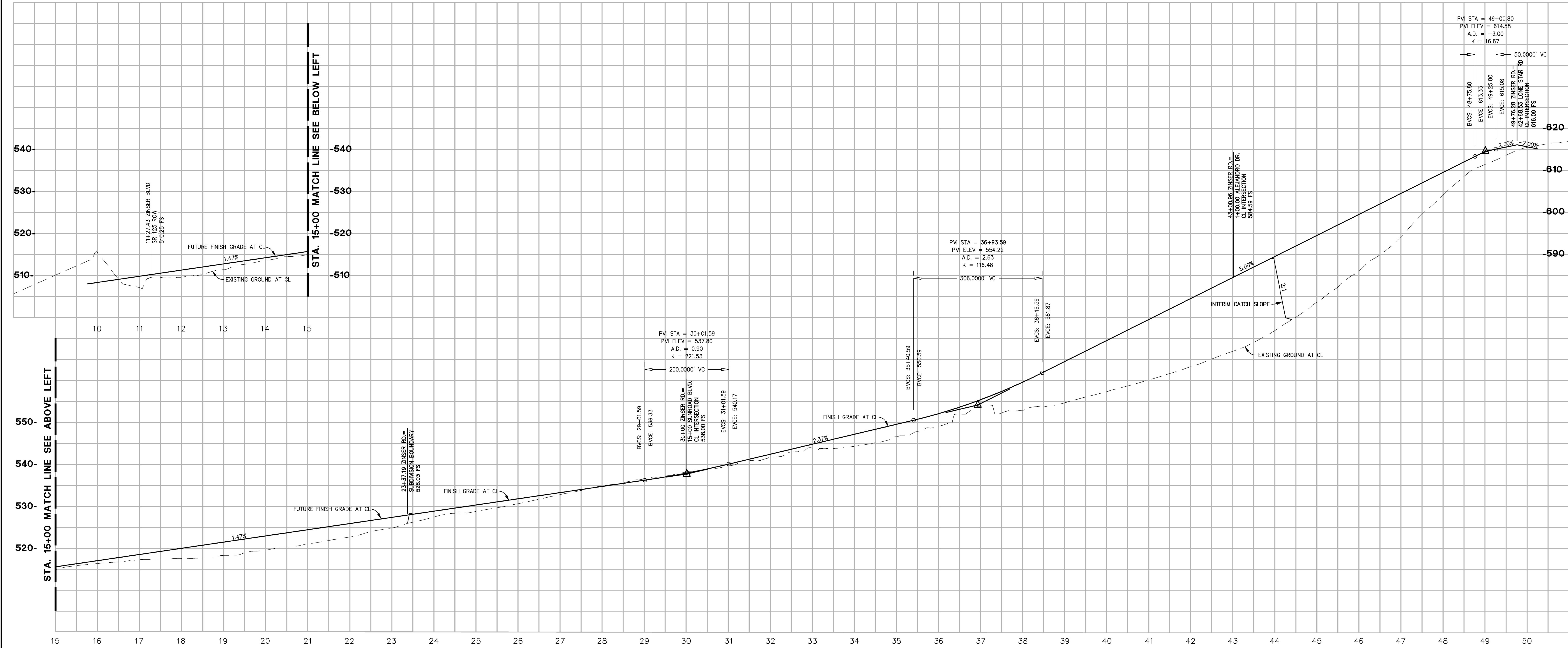
PROFILE: ZINSER ROAD SCALE: 1"= 100' HORIZ.; 1"= 10' VERT.
