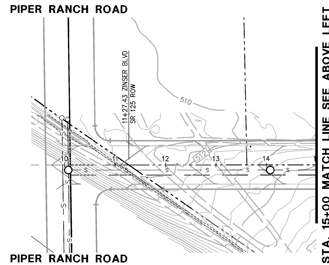
PLAN: ZINSER ROAD SCALE: 1"= 100'
