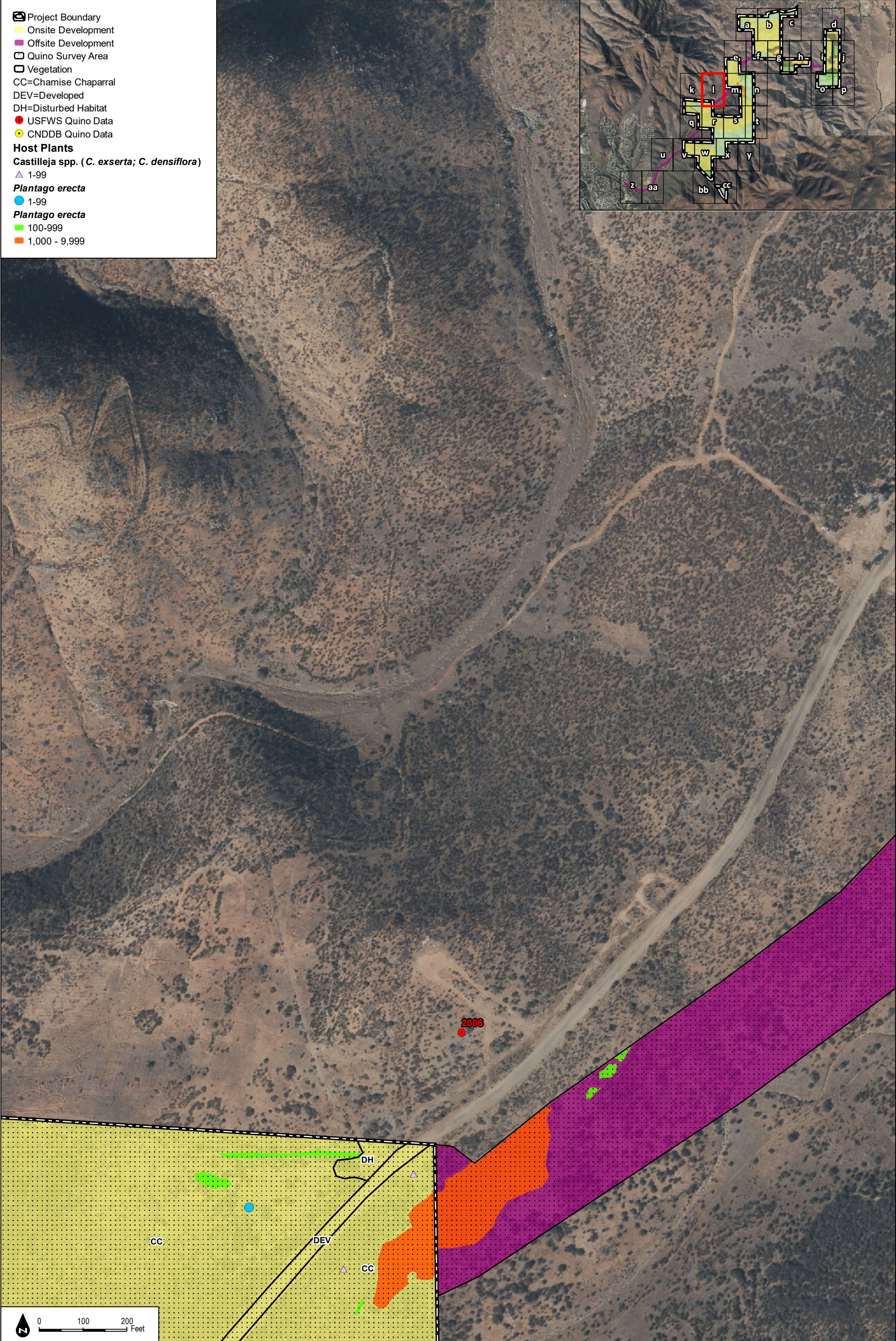
Figure 4-21 2016 Quino Host Plant Mapping and Historical Locations
