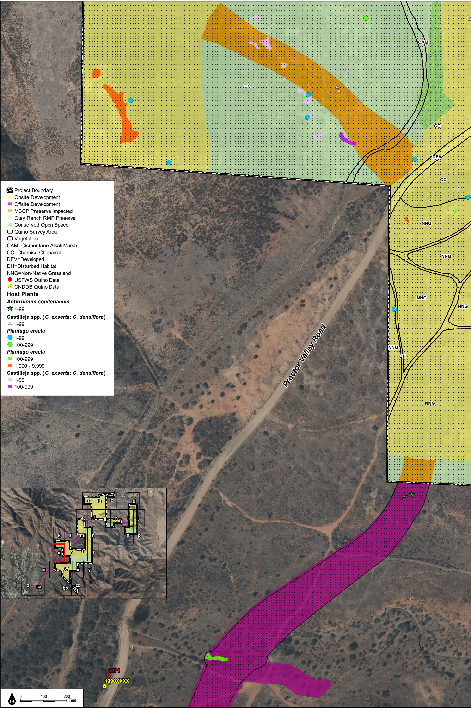
Figure 4-2q 2016 Quino Host Plant Mapping and Historical Locations
