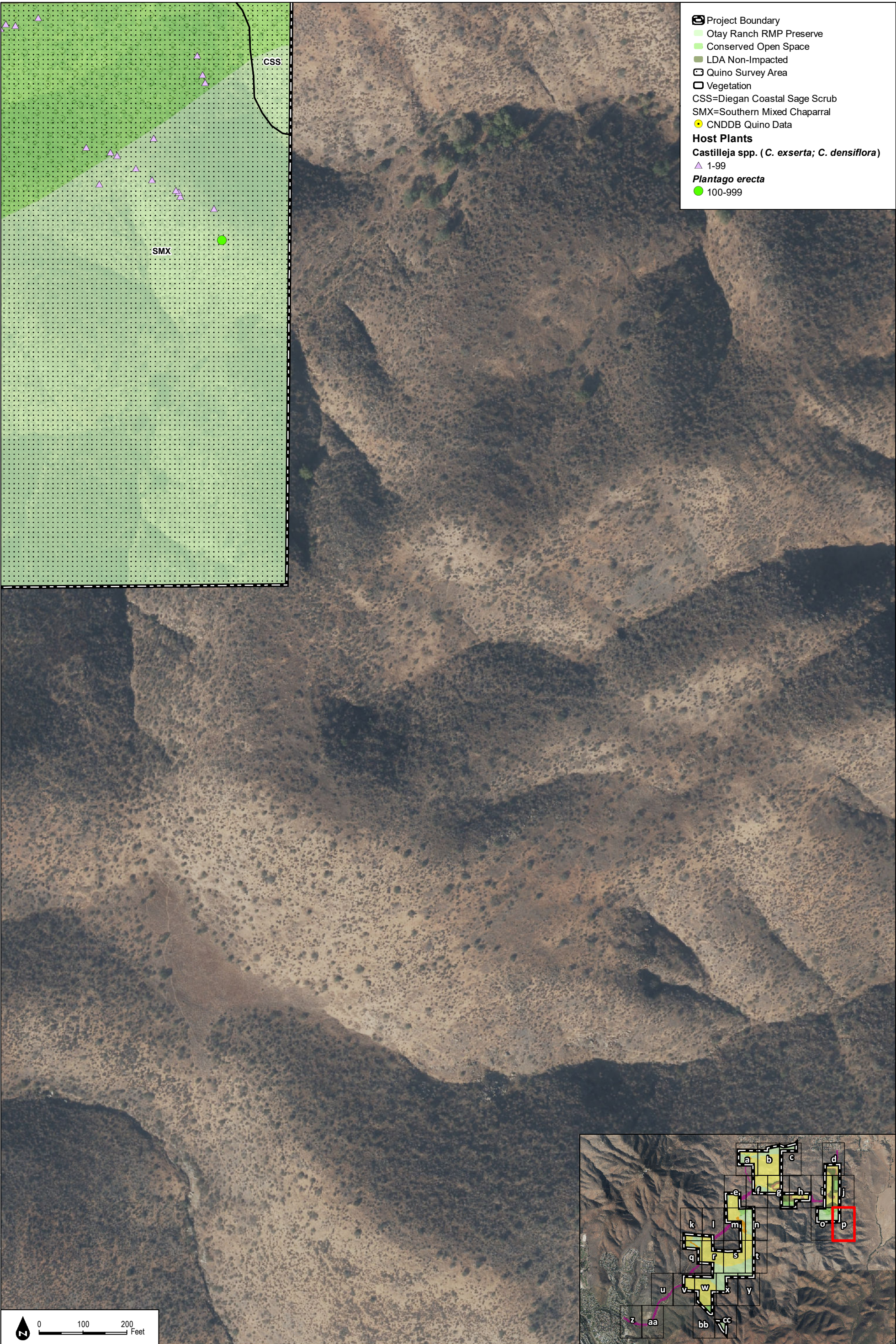
Figure 4-2p 2016 Quino Host Plant Mapping and Historical Locations
