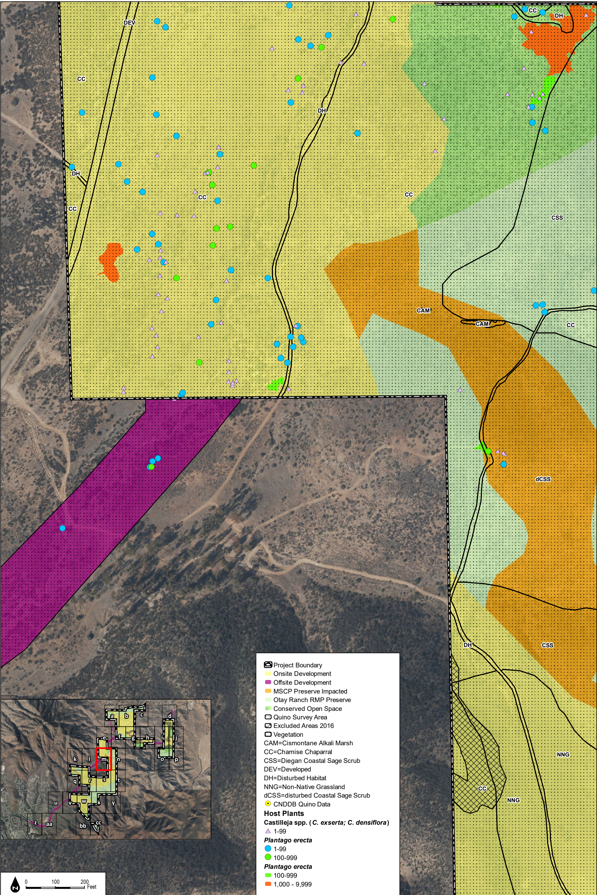
Figure 4-2m 2016 Quino Host Plant Mapping and Historical Locations
