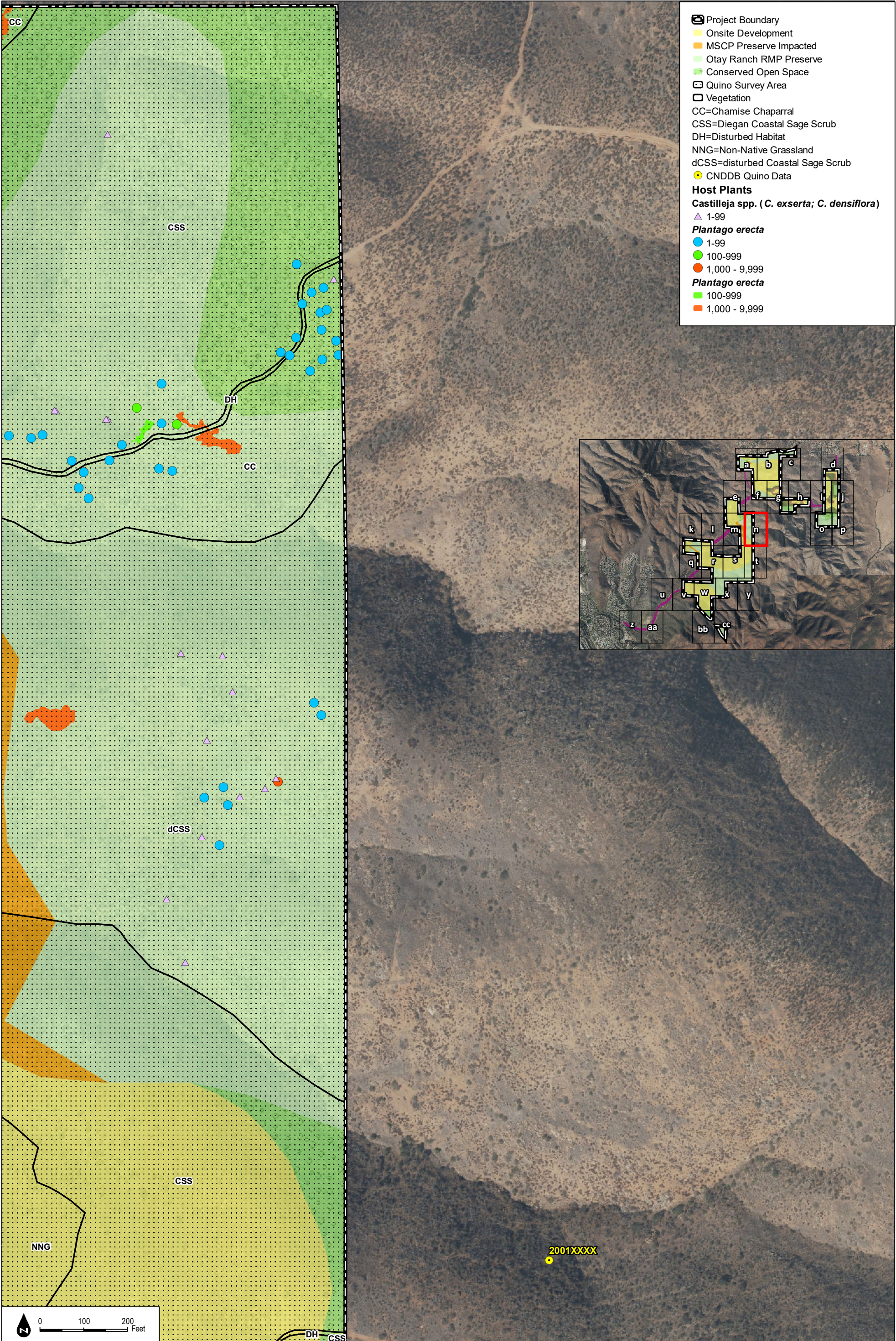
Figure 4-2n 2016 Quino Host Plant Mapping and Historical Locations
