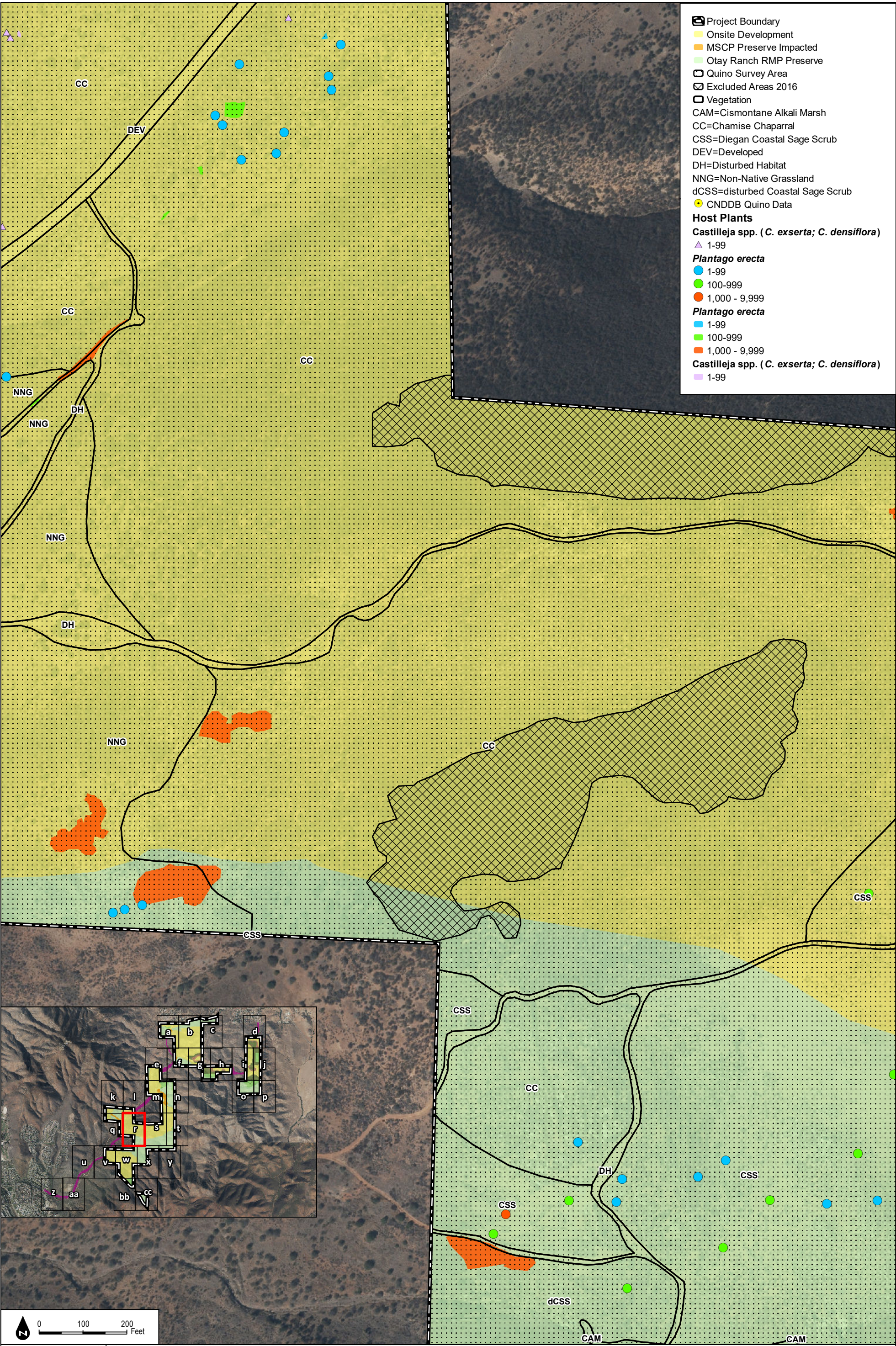
Figure 4-2r 2016 Quino Host Plant Mapping and Historical Locations
