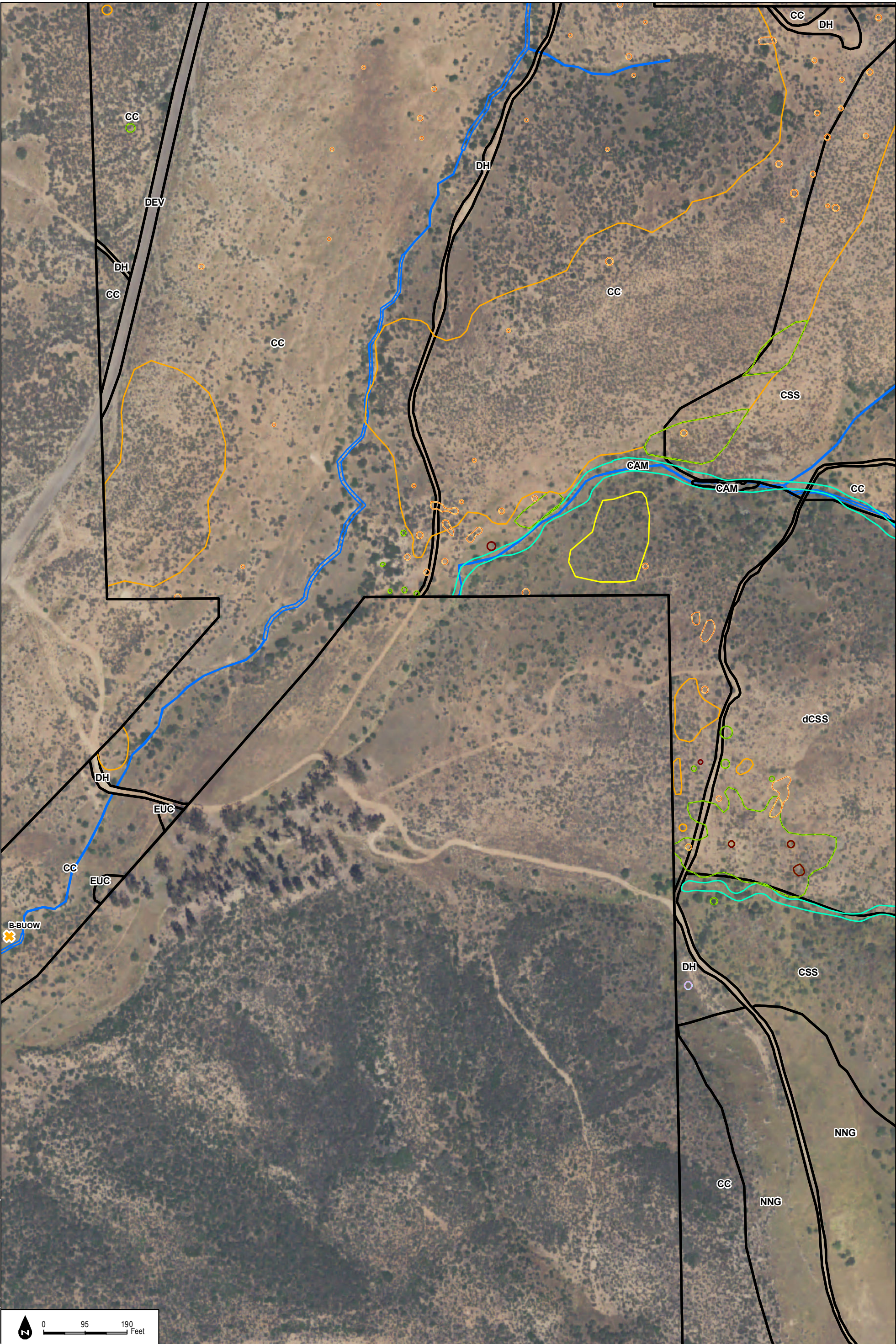
Figure 2.4-10m Biological Resources
