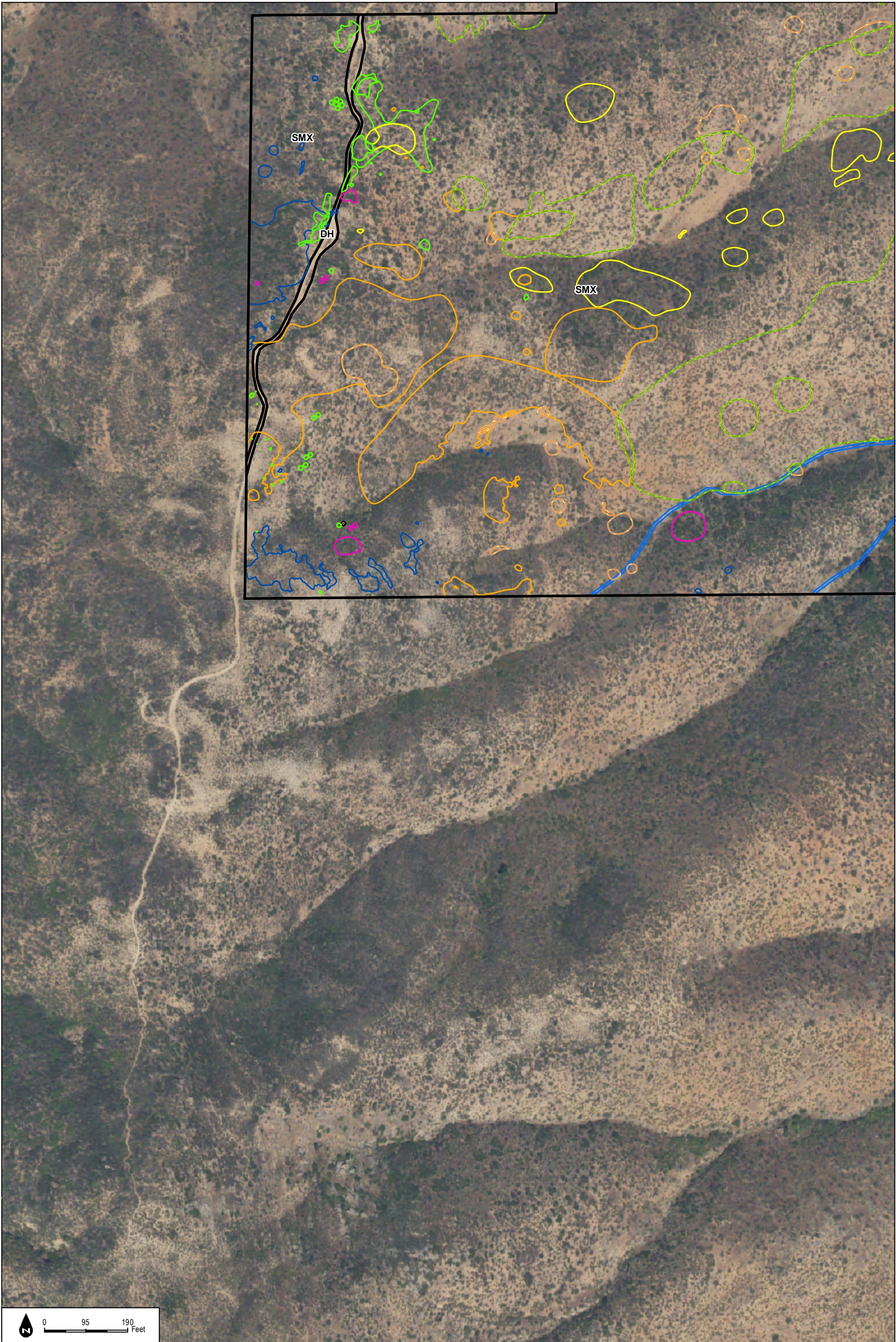
Figure 2.4-10o Biological Resources
