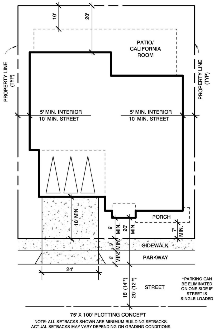
Exhibit 54 - SF-I Typical Single Family Plot (75' x 100')
