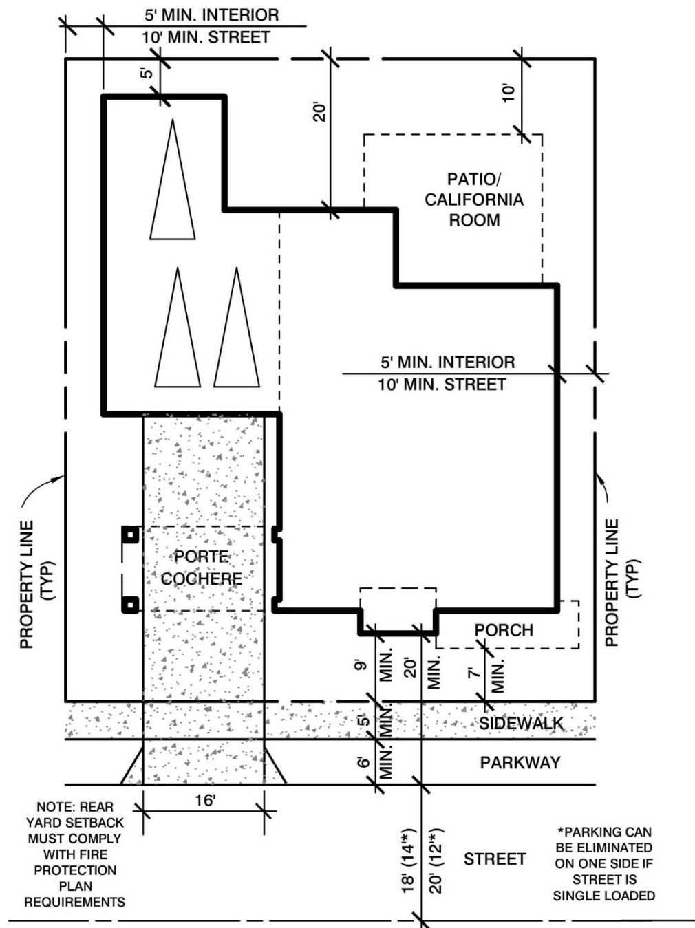
70' X 85' PLOTTING CONCEPT
