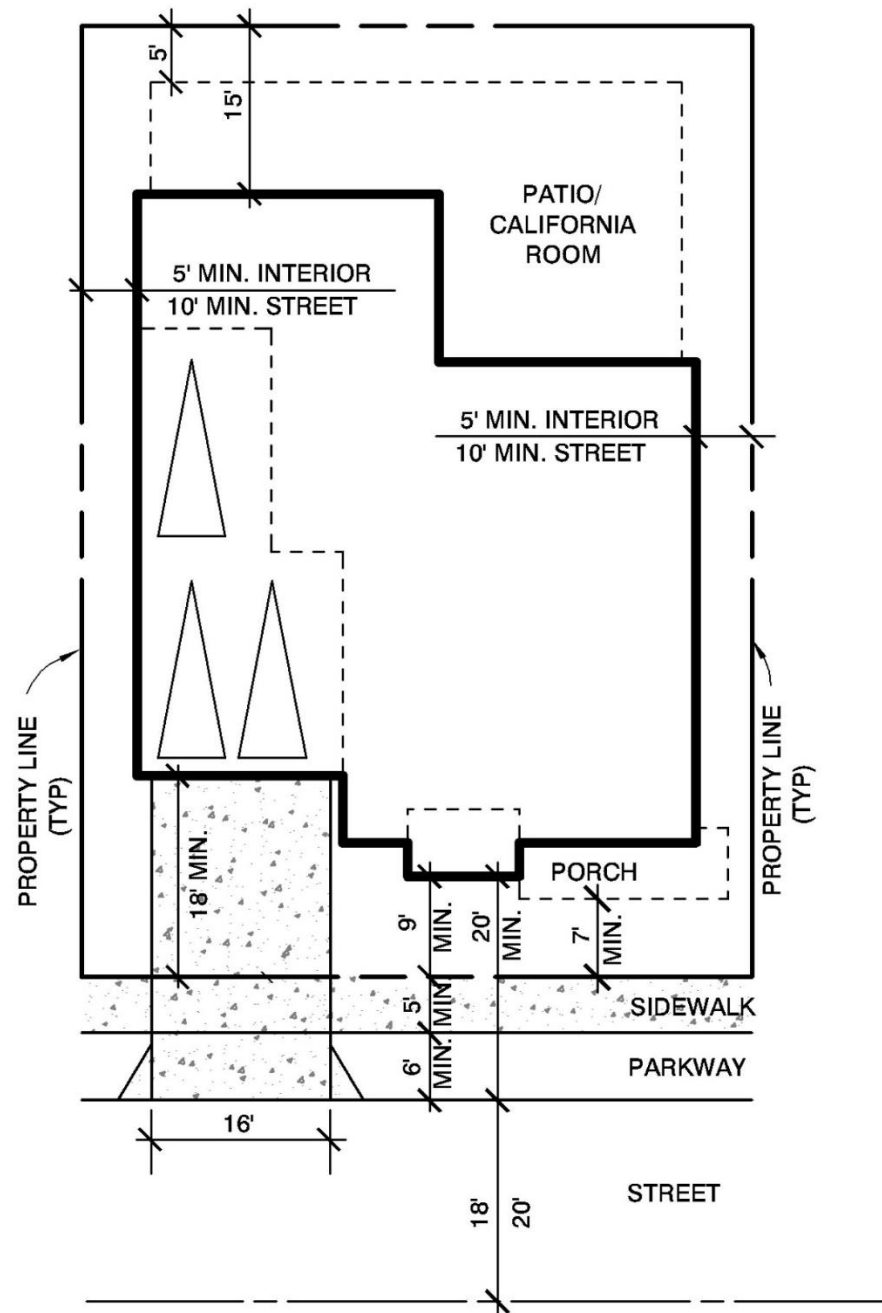
60' X 85' PLOTTING CONCEPT
