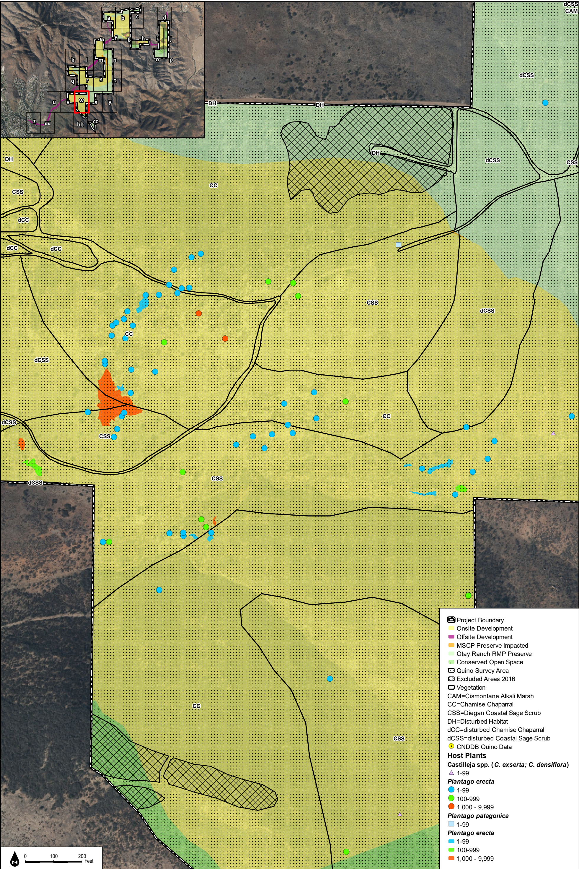
Figure 4-2w 2016 Quino Host Plant Mapping and Historical Locations
