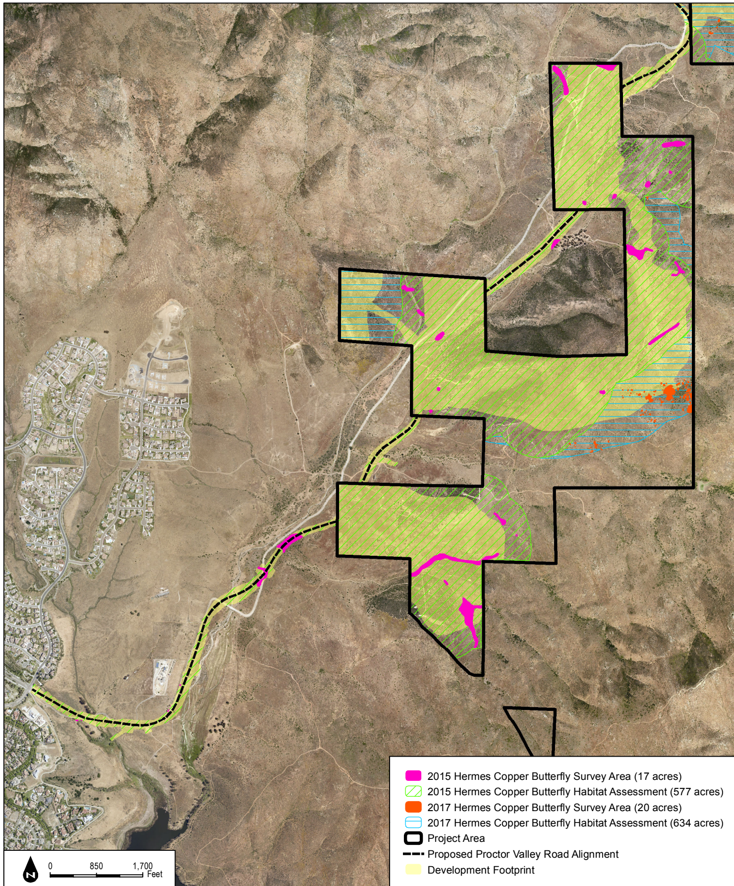
FIGURE 2.4-7a Hermes Copper Survey Area
