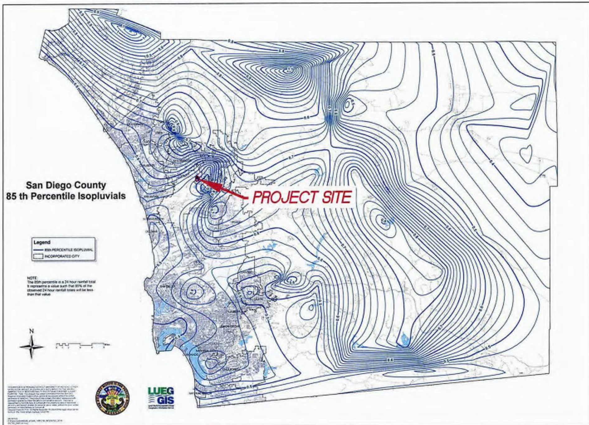
Figure B.1-1: 85th Percentile 24-hour Isopluvial Map
