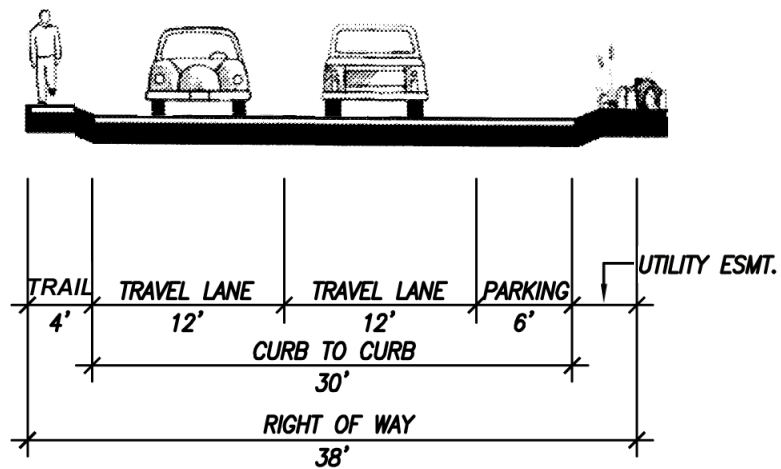
Cross Section
