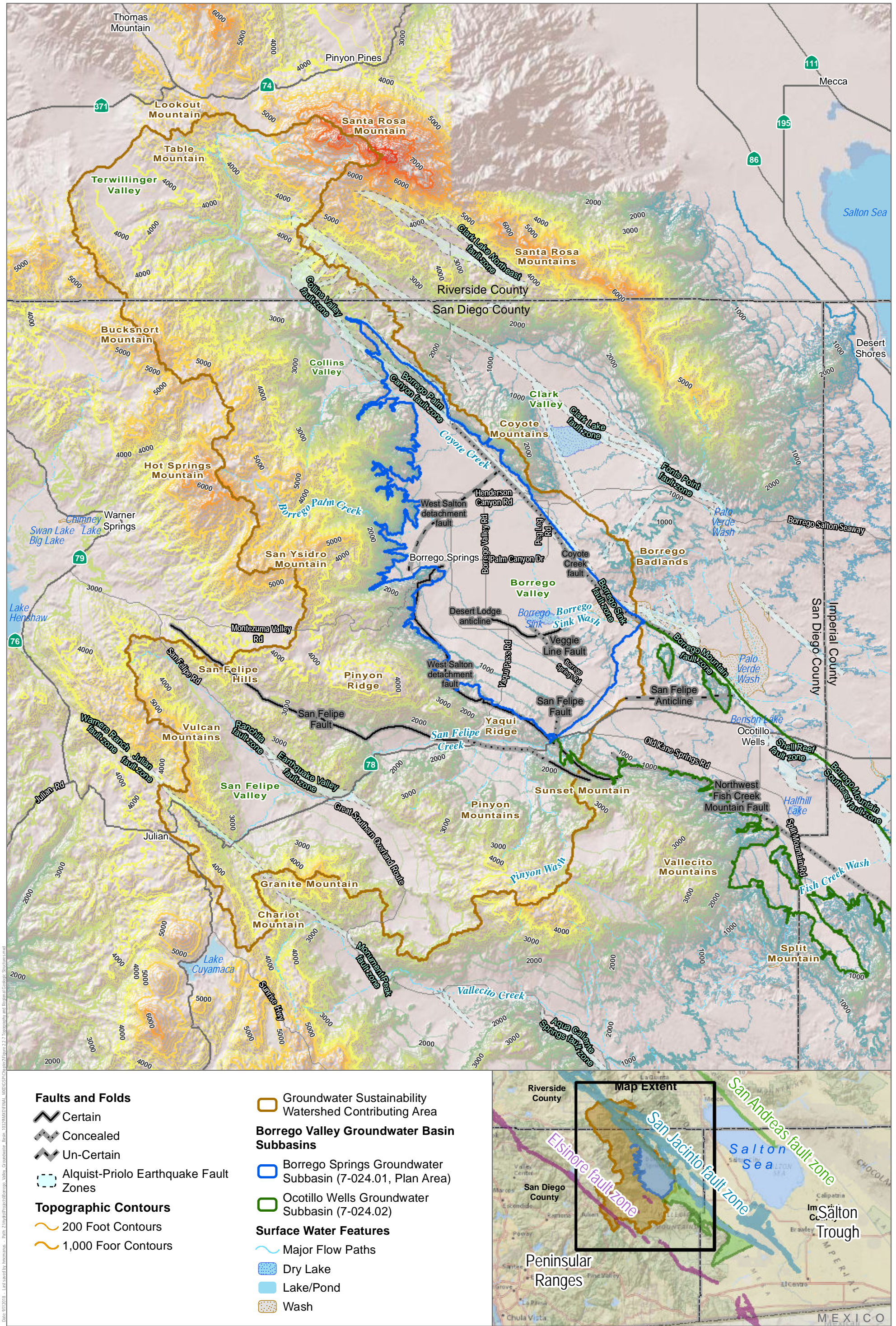
Figure 2.2-7 Topography and Regional Geologic Structures Groundwater Sustainability Plan for the Borrego Valley Groundwater Basin
