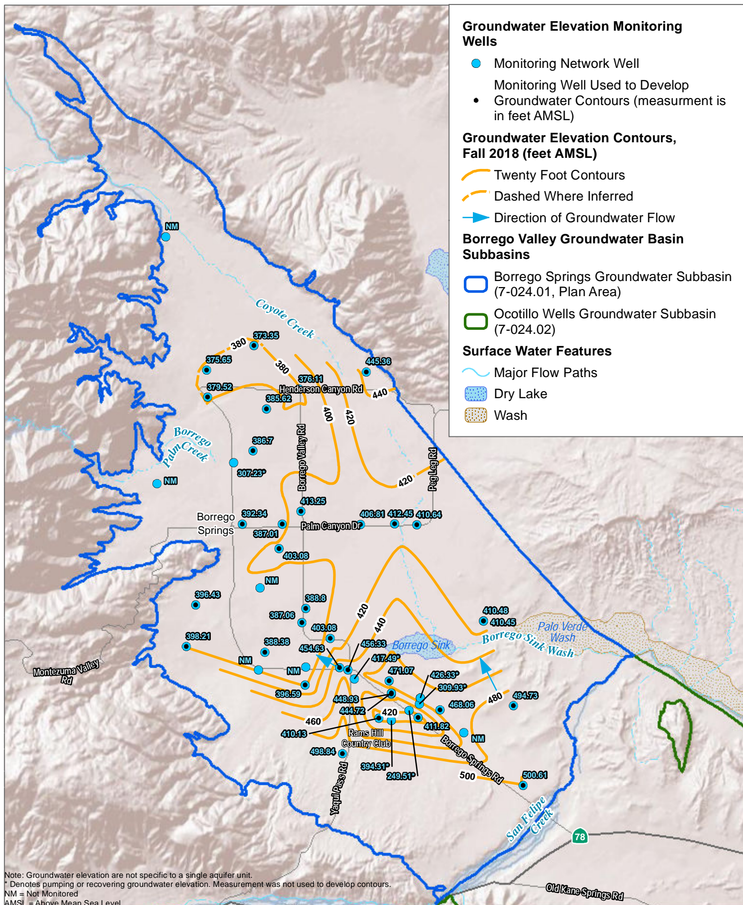
Figure 2.2-13B Current Groundwater Levels in the Plan Area (Fall 2018)
