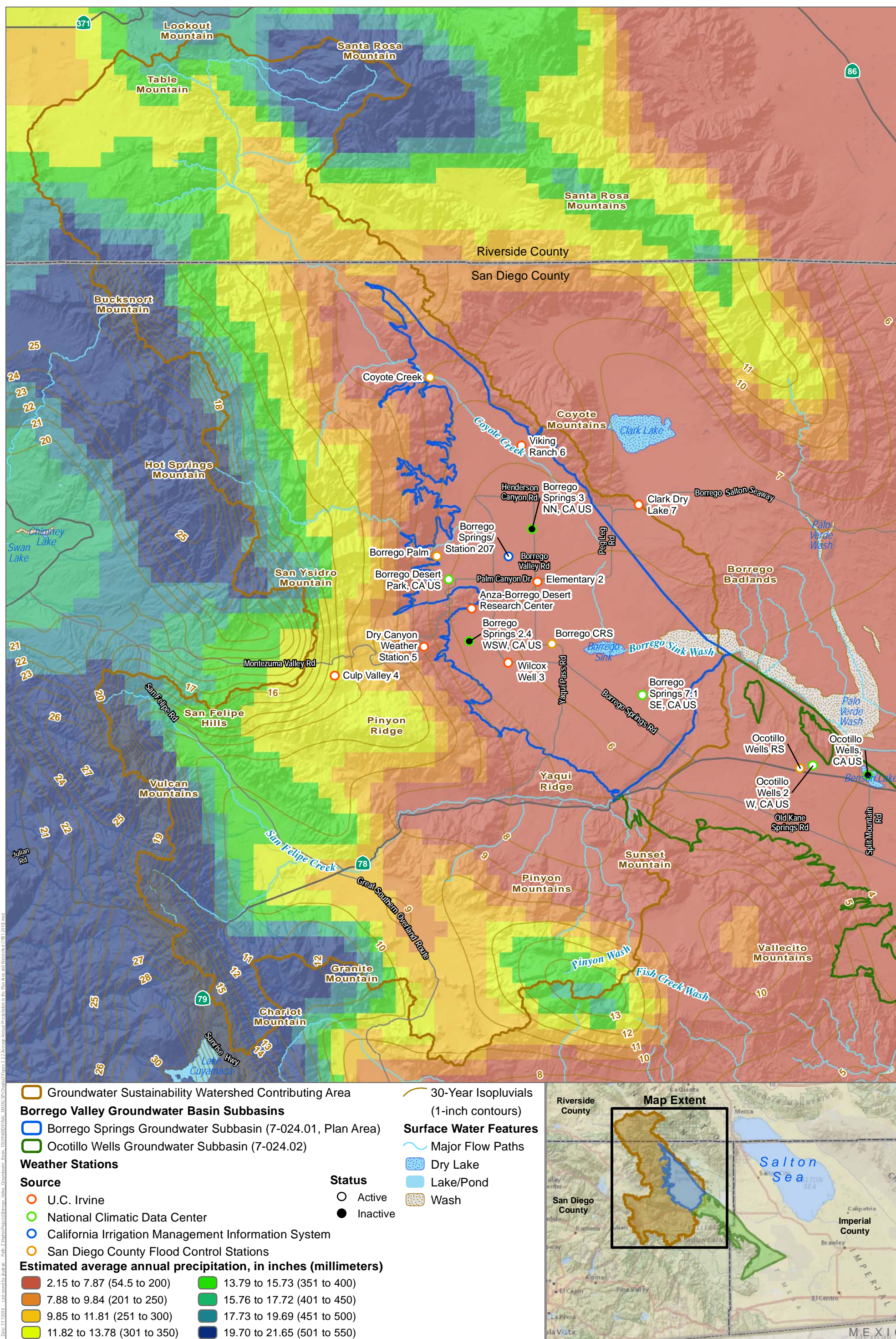
Figure 2.2-2 Average Annual Precipitation in the Plan Area and Watershed (1981-2010) Groundwater Sustainability Plan for the Borrego Valley Groundwater Basin
