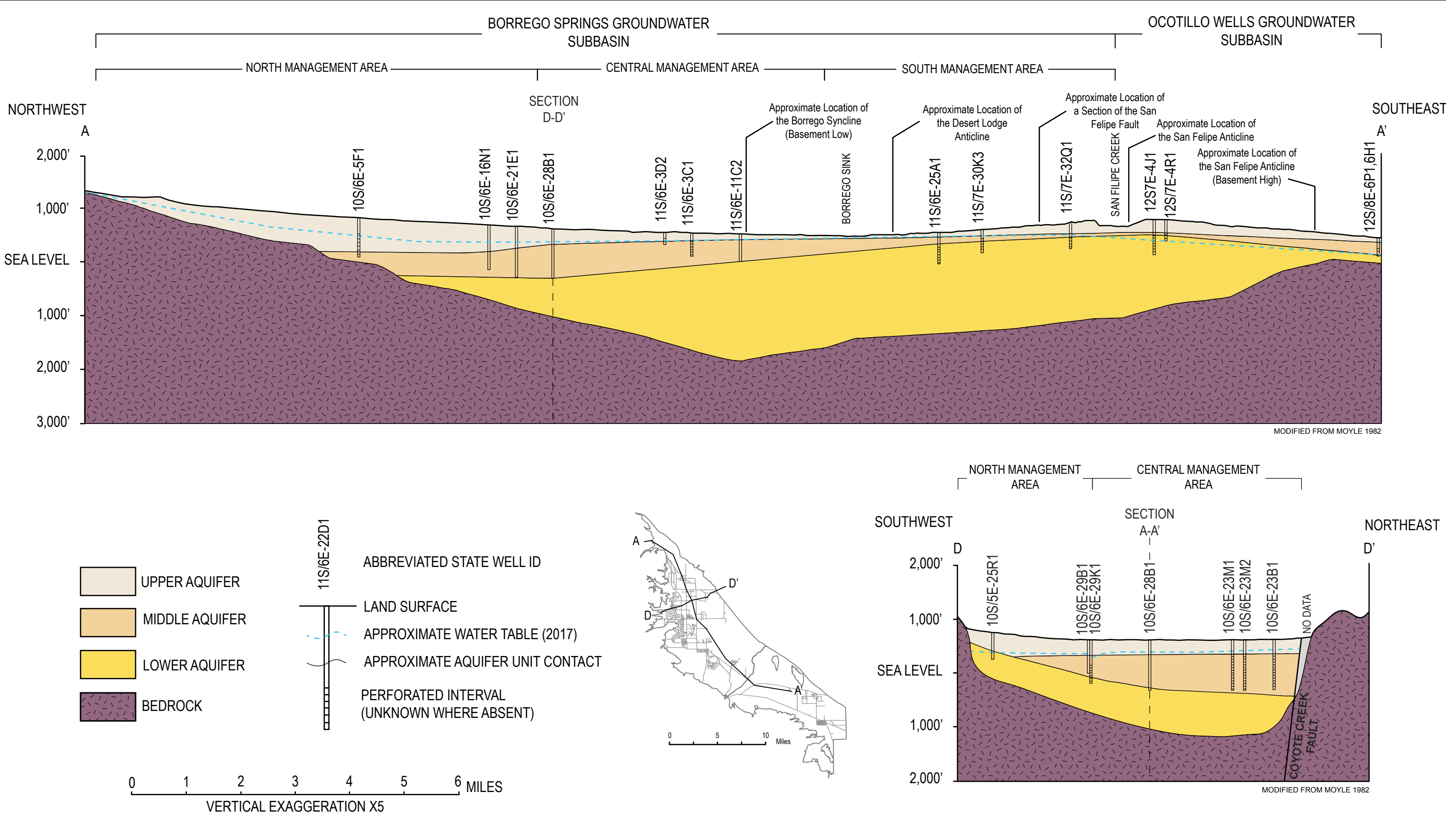
FIGURE 2.2-10 Hydrogeologic Cross Sections of the Plan Area Borrego Valley Groundwater Basin Groundwater Sustainability Plan
