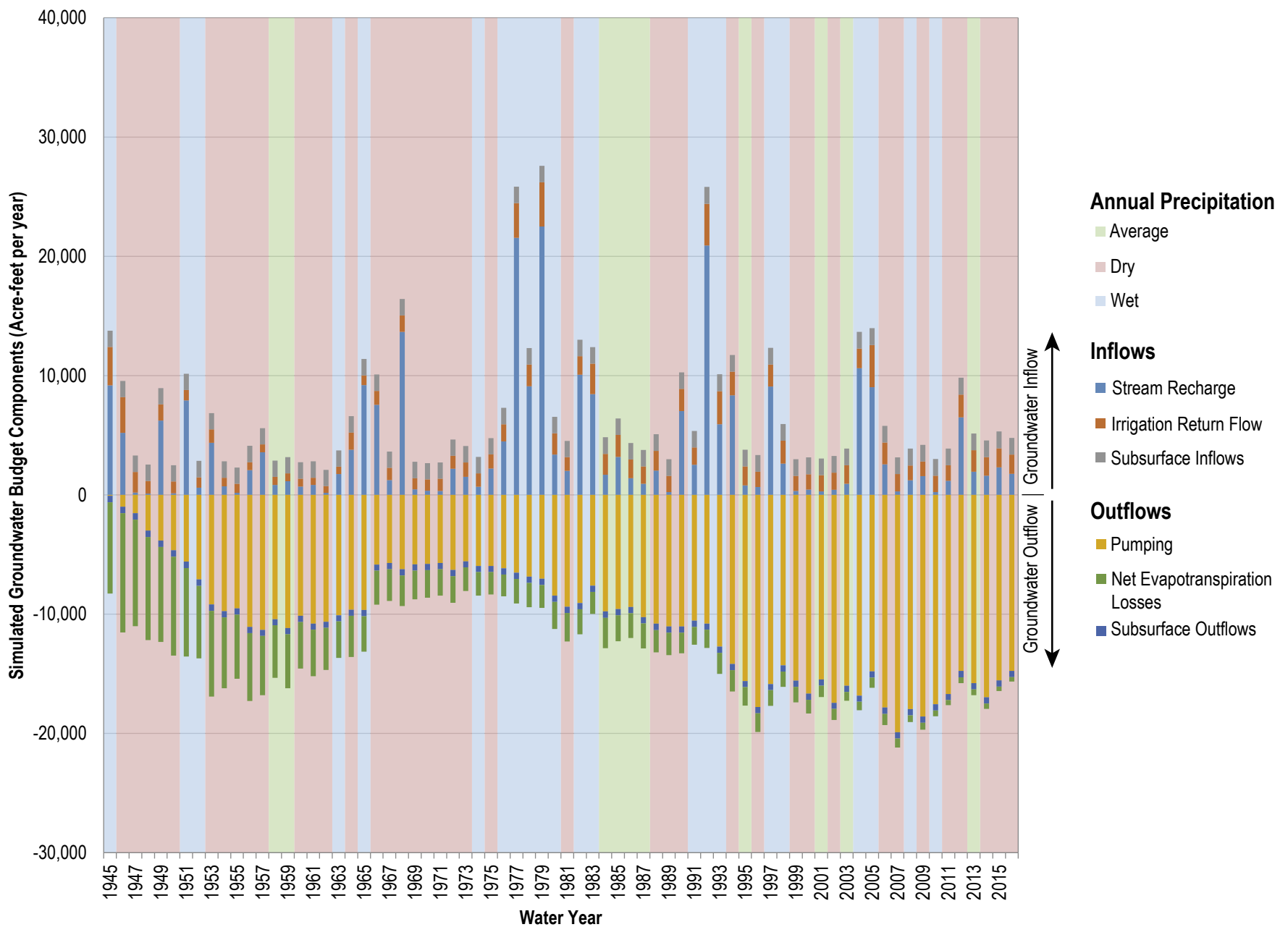
FIGURE 2.2-22A Groundwater Inflows and Outflows by Year (1945 - 2016) Groundwater Sustainability Plan for the Borrego Valley Groundwater Basin
