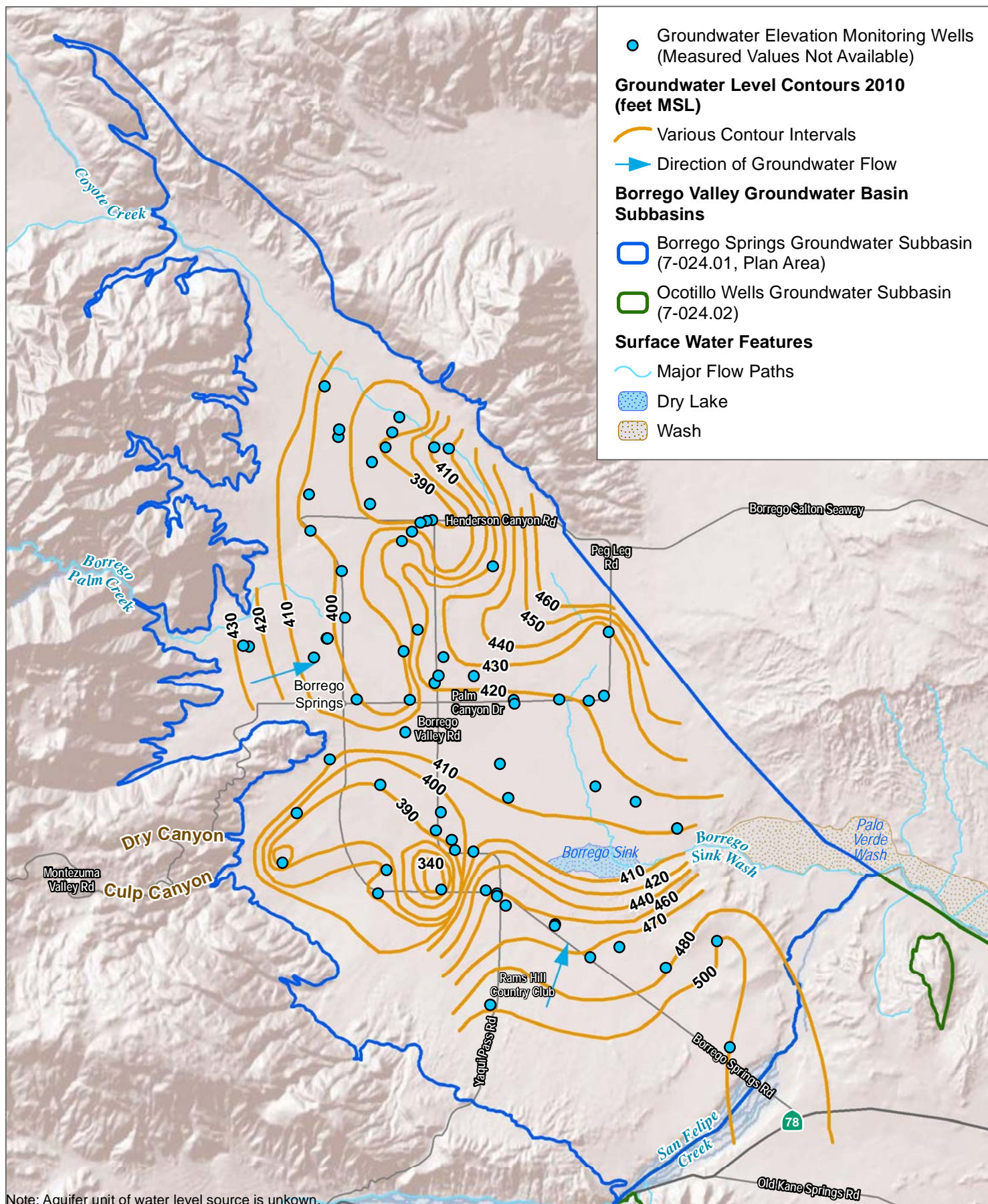
Figure 2.2-13C Historical Groundwater Levels in the Plan Area (2010) Groundwater Sustainability Plan for the Borrego Valley Groundwater Basin
