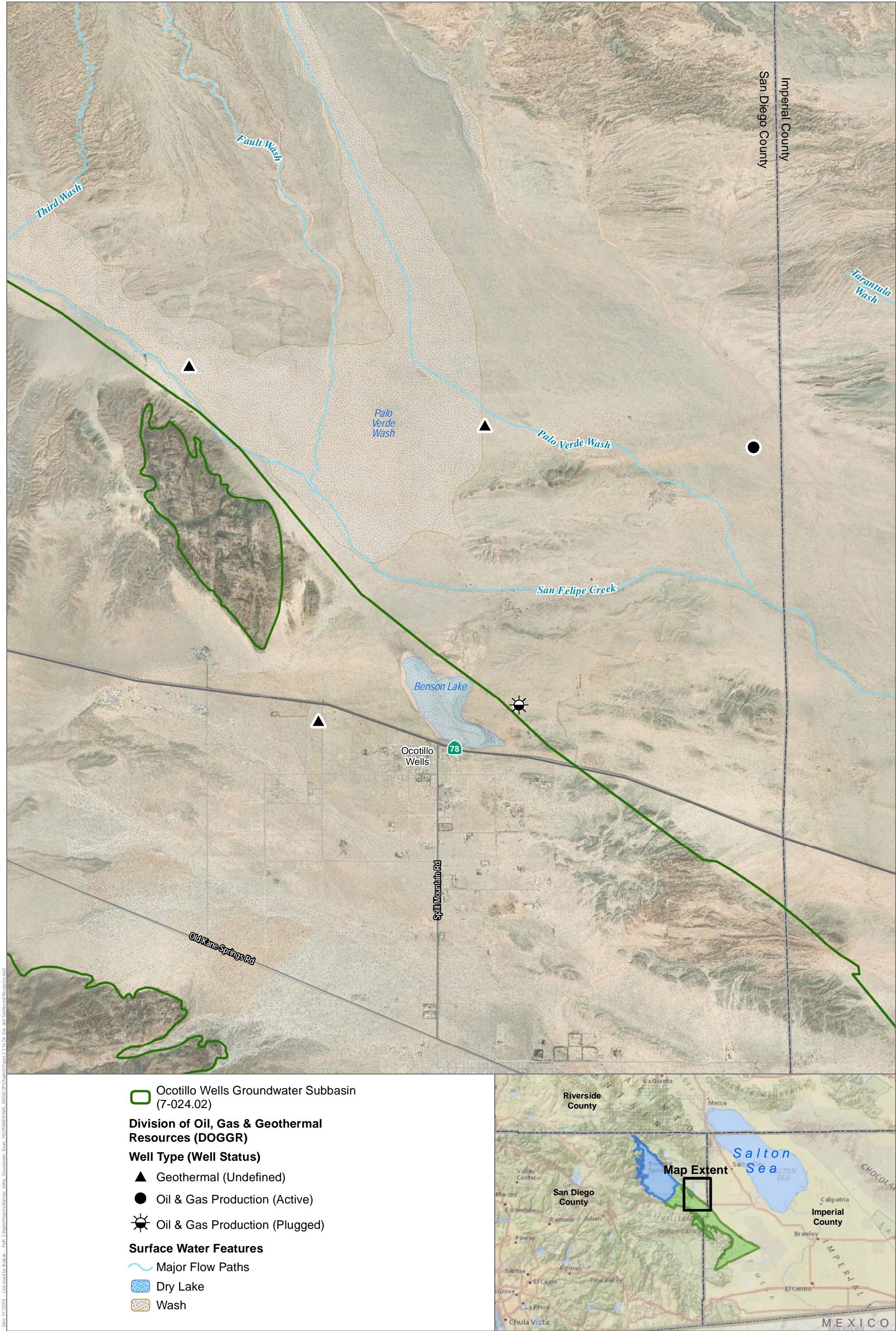
DRAFT February 2019 DATUM: NAD 1983. DATA SOURCE: DOGGR 2017 DUDEK 0 2,000 4,000 Feet Figure 2.2-16 Oil, Gas, and Geothermal Resources Groundwater Sustainability Plan for the Borrego Valley Groundwater Basin
