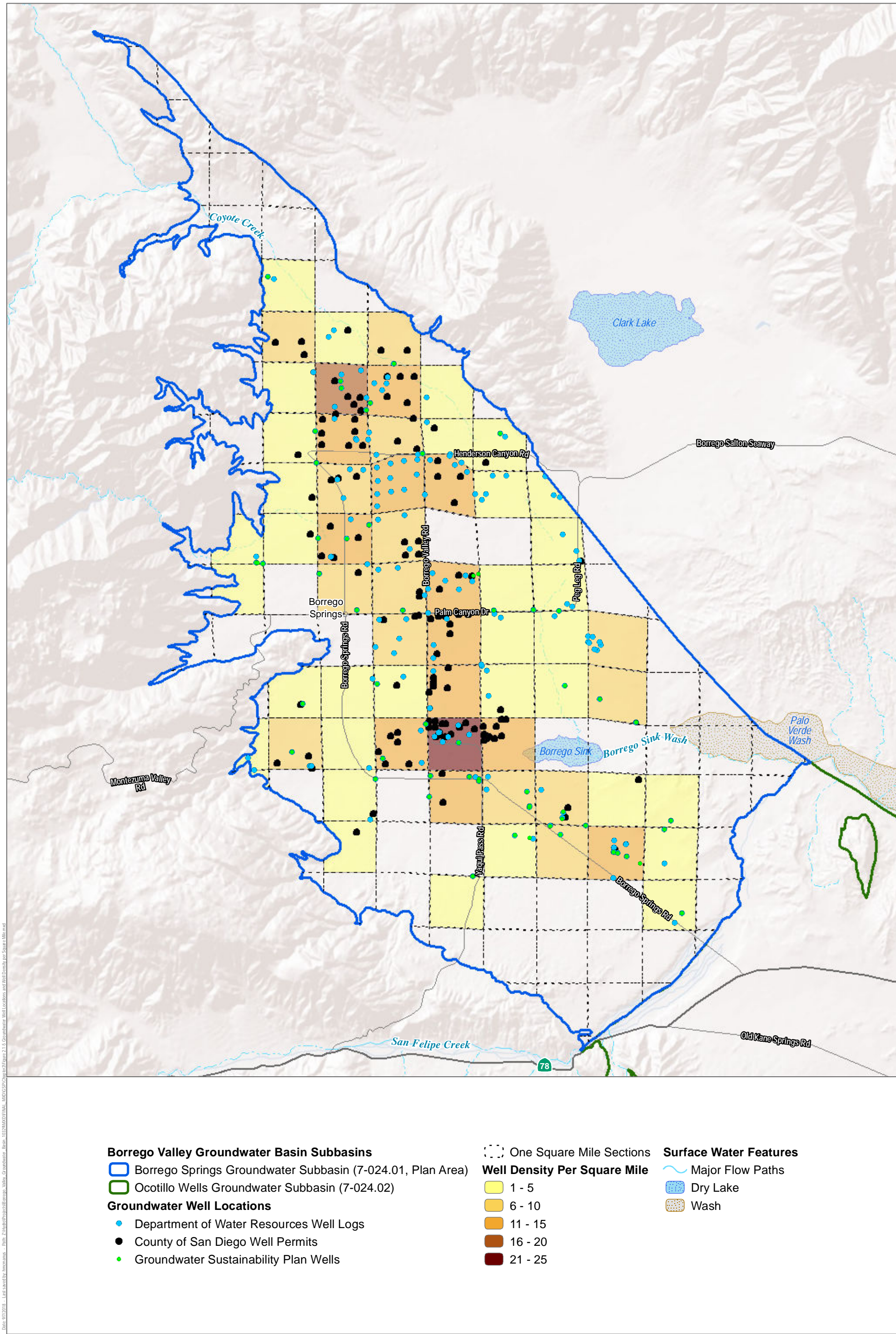
Figure 2.1-5 Groundwater Well Locations and Well Density per Square Mile Groundwater Sustainability Plan for the Borrego Valley Groundwater Basin
