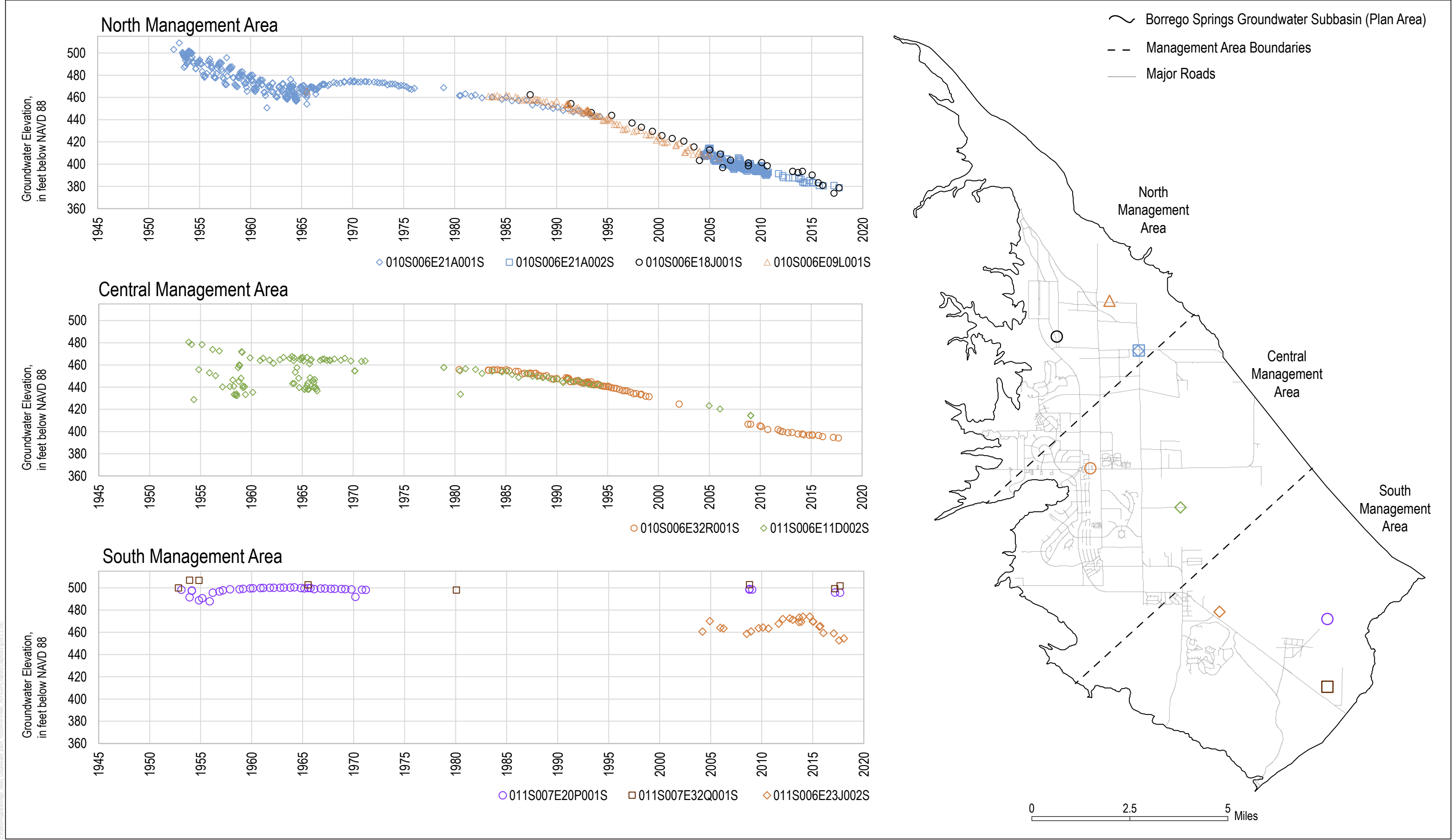
FIGURE 2.2-13E Groundwater Levels in Selected Wells in Parts of the Plan Area, 1952 - 2018 Groundwater Sustainability Plan for the Borrego Valley Groundwater Basin
