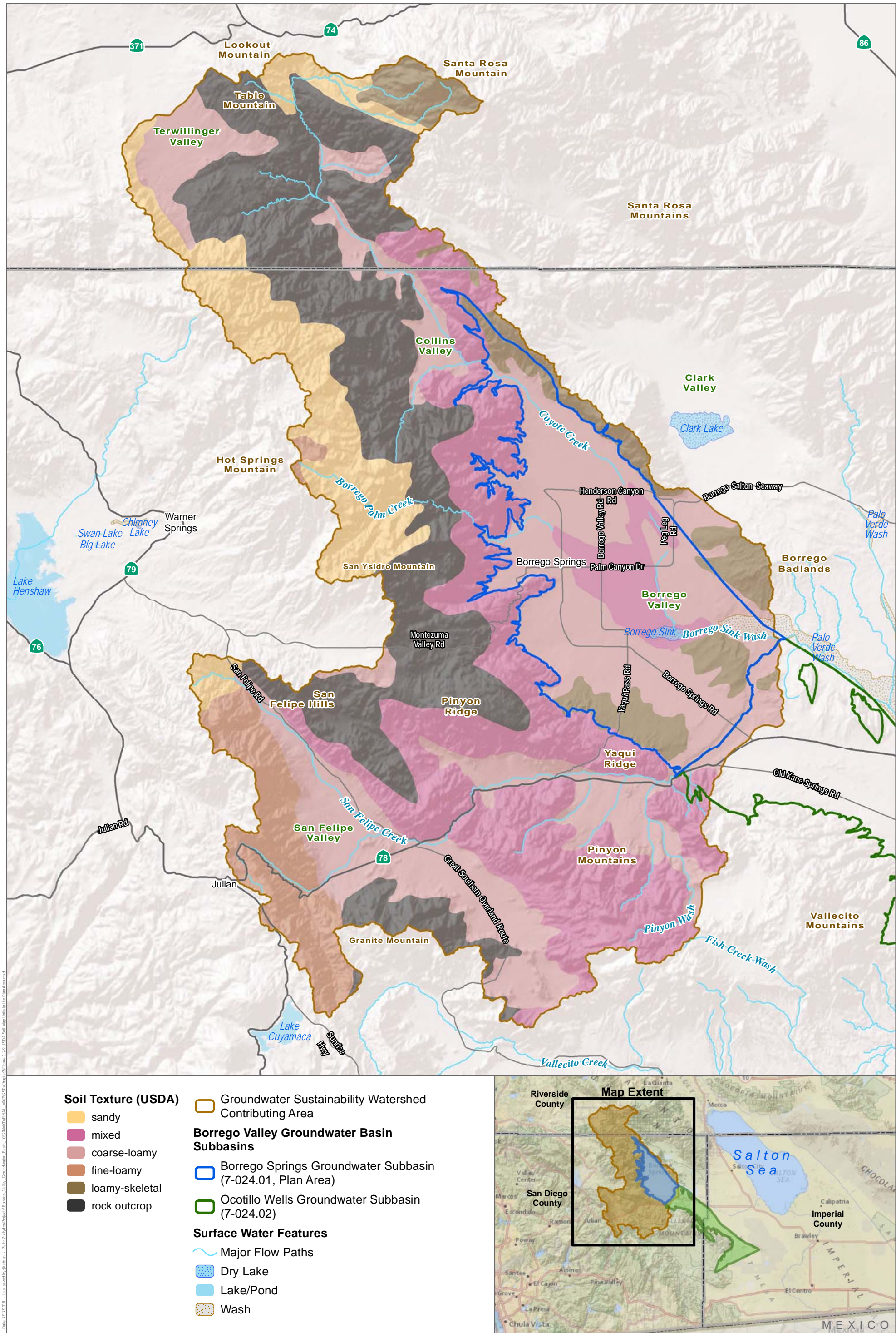
Figure 2.2-9 USDA Soil Map Units in the Plan Area
