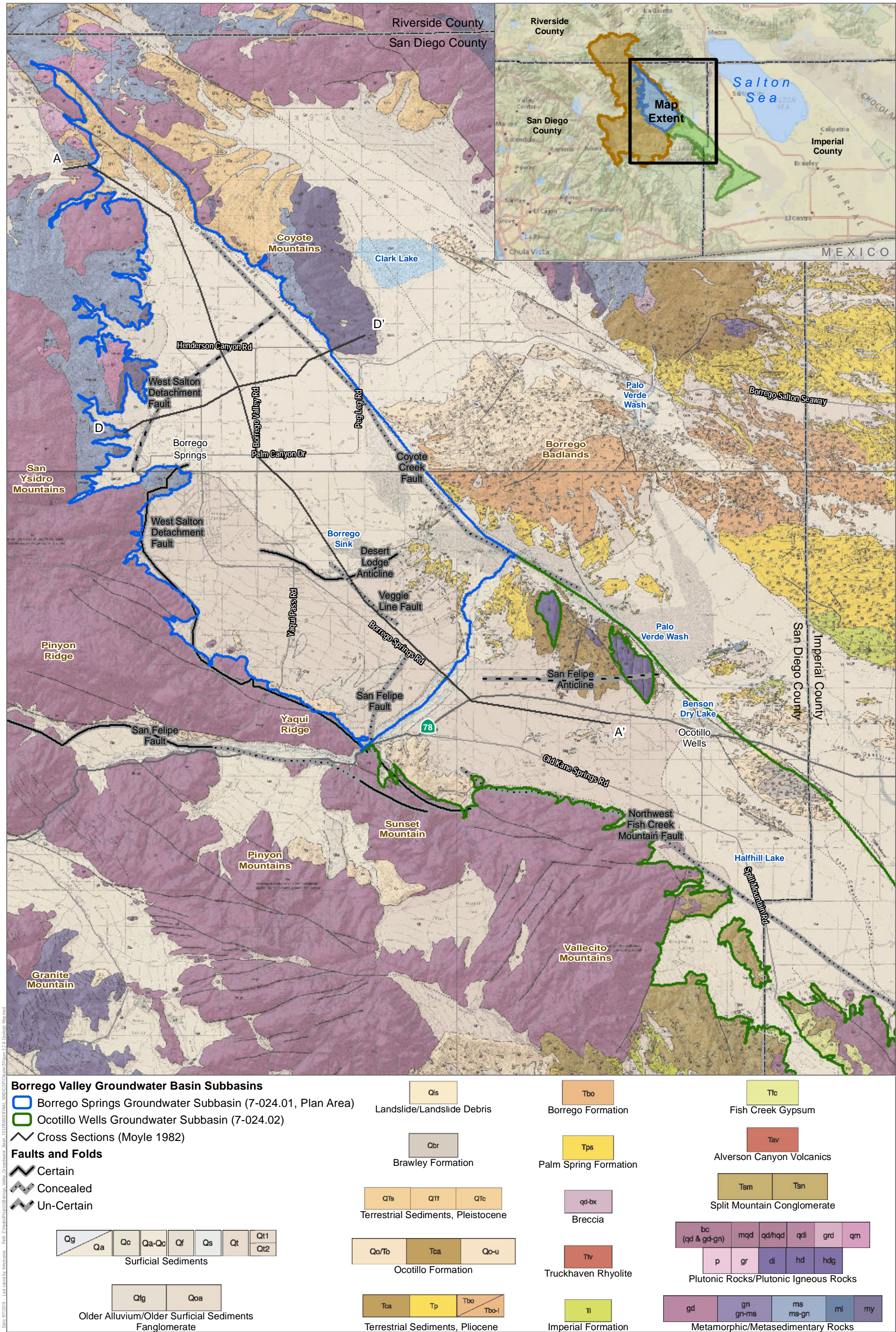
Figure 2.2-8 Geologic Map
