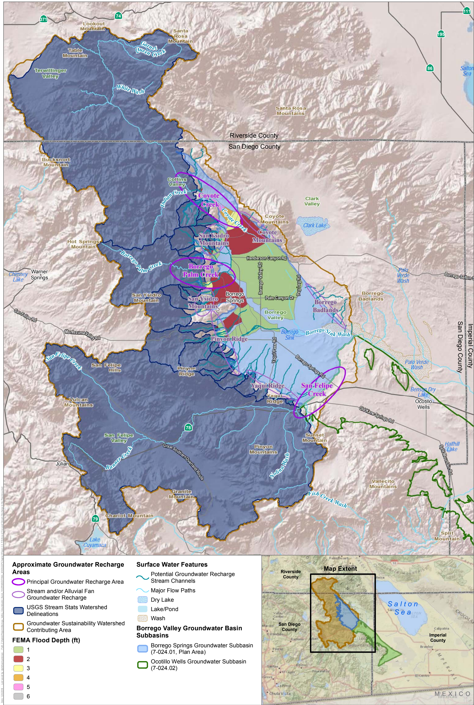
Figure 2.2-11 Areas of Focused Stream Recharge in the Plan Area Groundwater Sustainability Plan for the Borrego Valley Groundwater Basin
