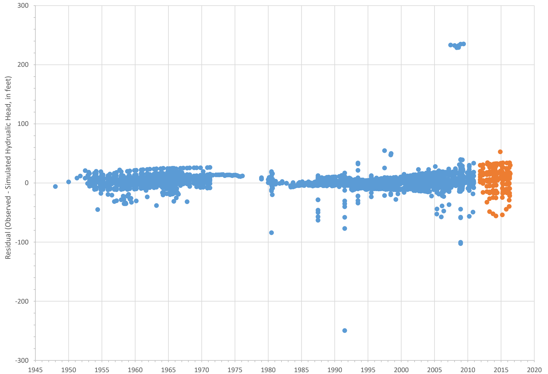
Figure 11. Observed - Simulated Hydraulic Heads (Residuals) from 1945 to 2016
