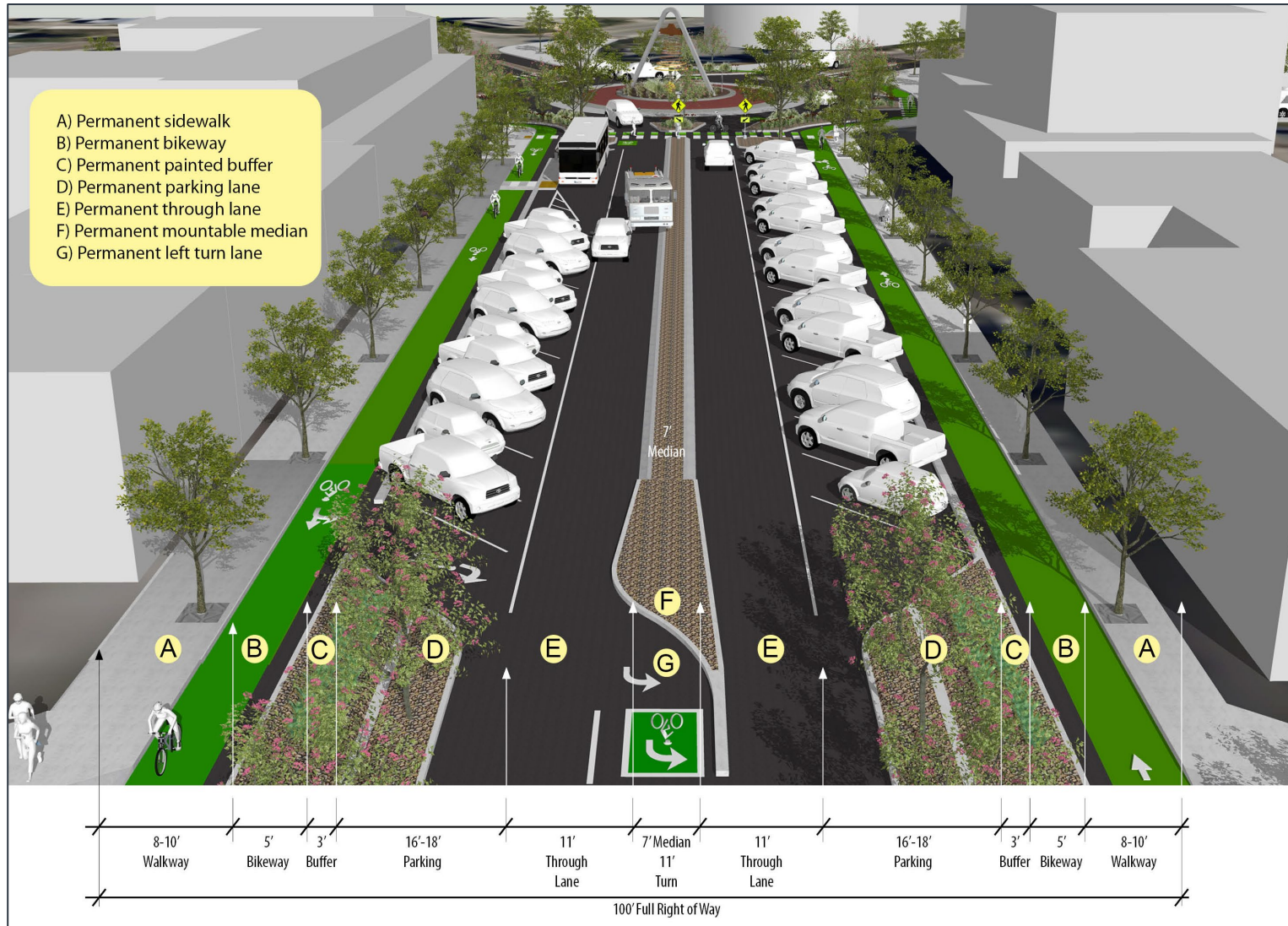
Figure 2-28D: Campo Road Looking East Toward East-end Roundabout at Granada Avenue (100-foot total public right-of-way) Phase 3 Geometrics
