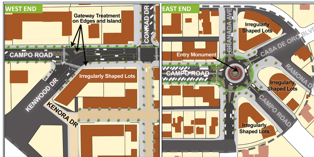
Figure 2-8: Potential Gateway Layout
