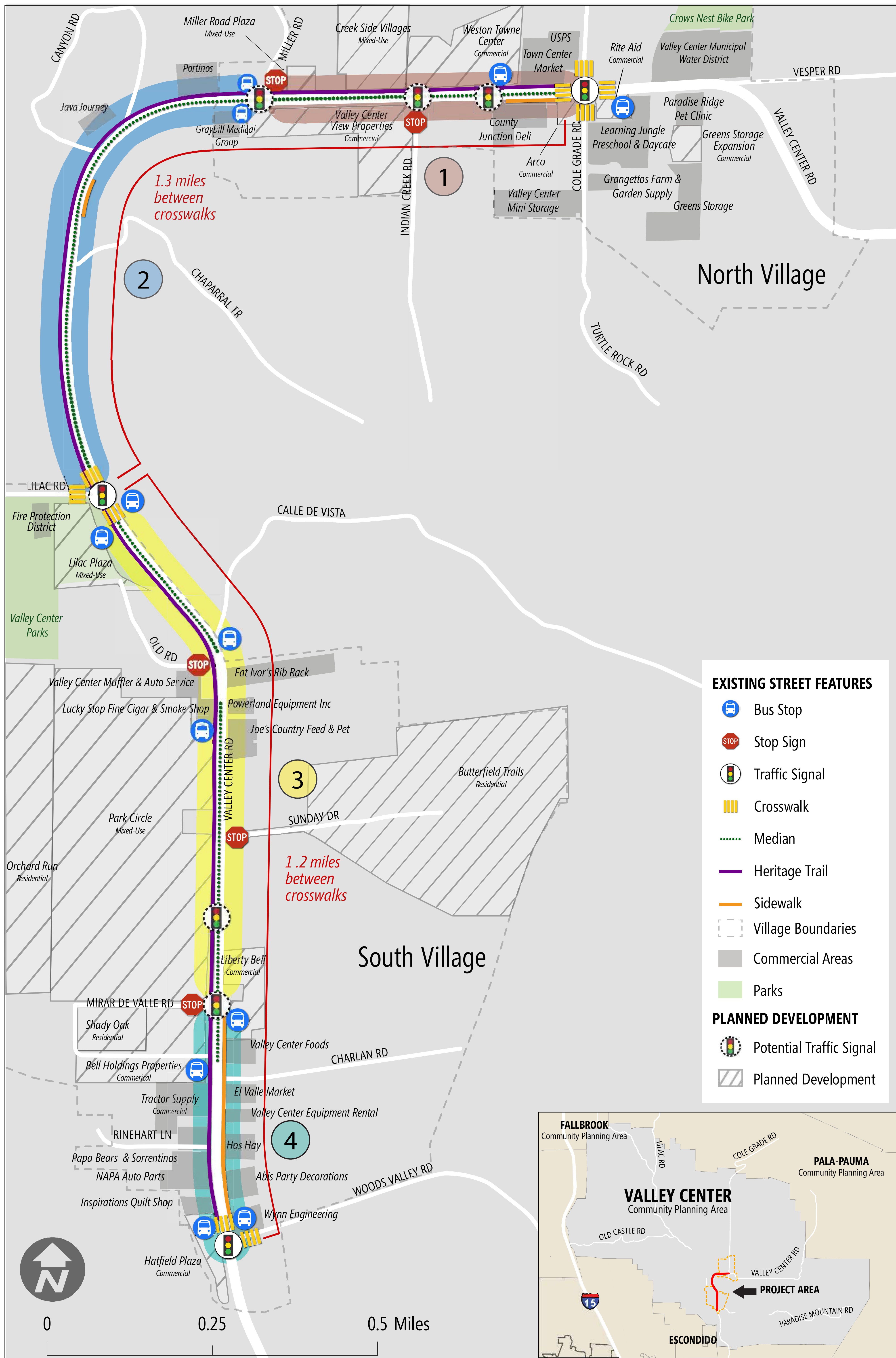
COLE GRADE RD to MILLER RD: Boulevard with raised median
