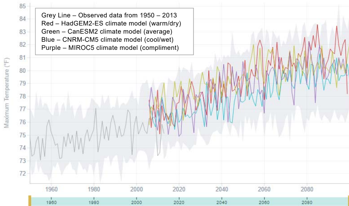
Figure 2: Projected Changes in Annual Average Maximum Temperatures under the Low-Emissions Scenario (1950–2100) (CEC 2017a)
