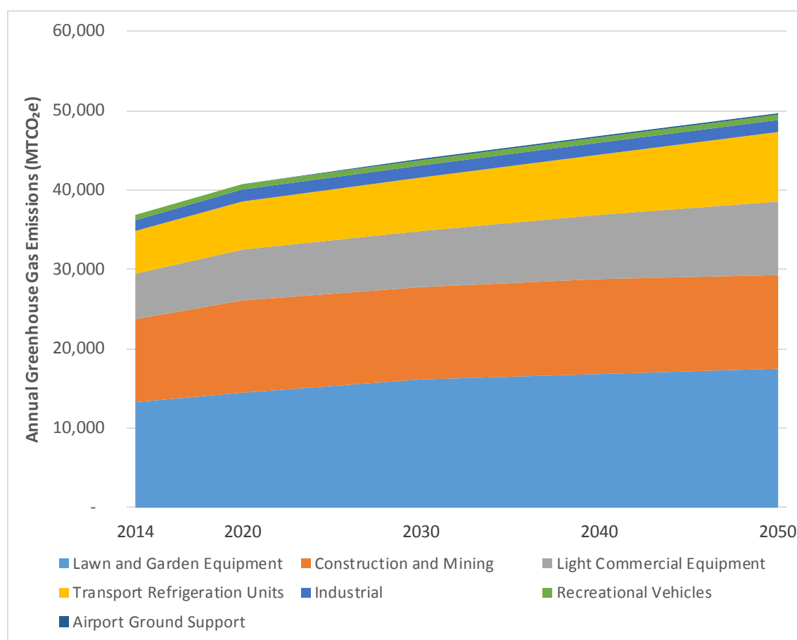
Figure 20: Off-Road Emissions Projections (2014-2050)
