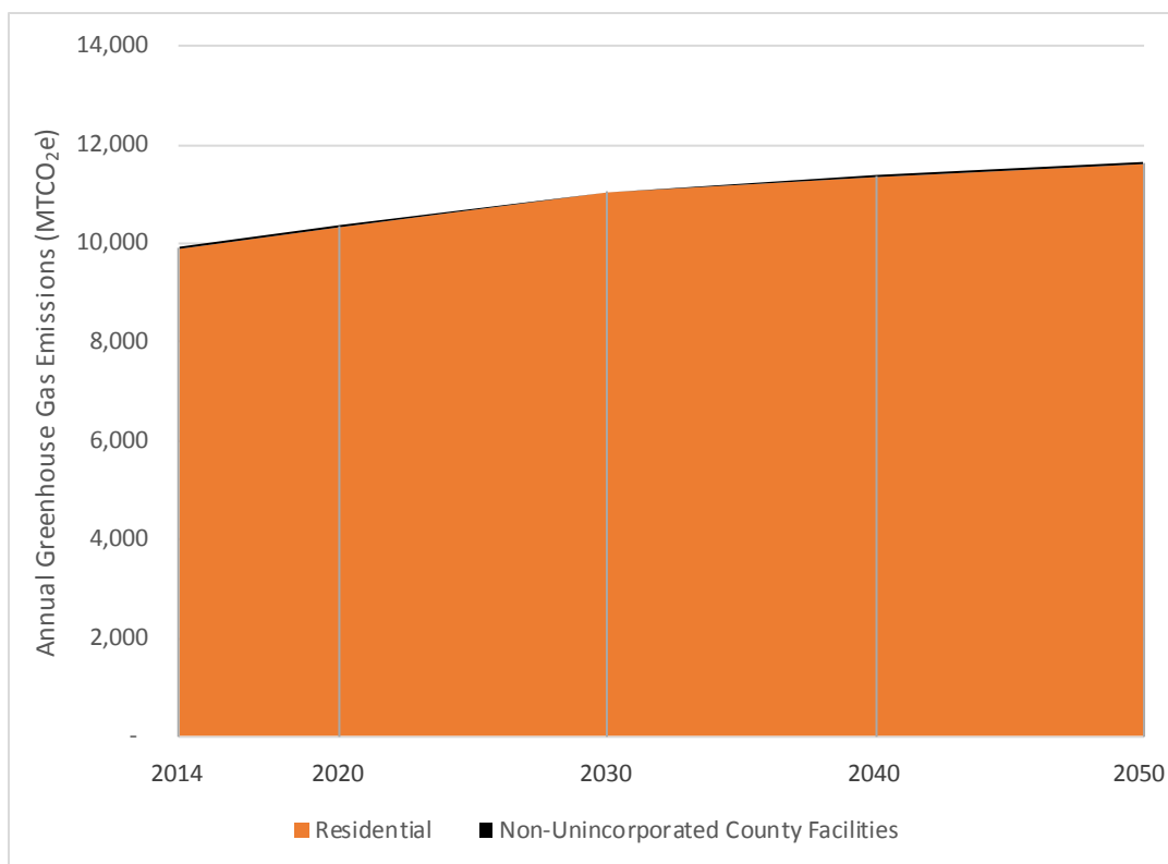
Figure 16: Propane Emissions Projections (2014-2050)
