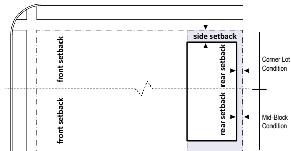
D. PARKING AND STORAGE LOCATION DIAGRAM
