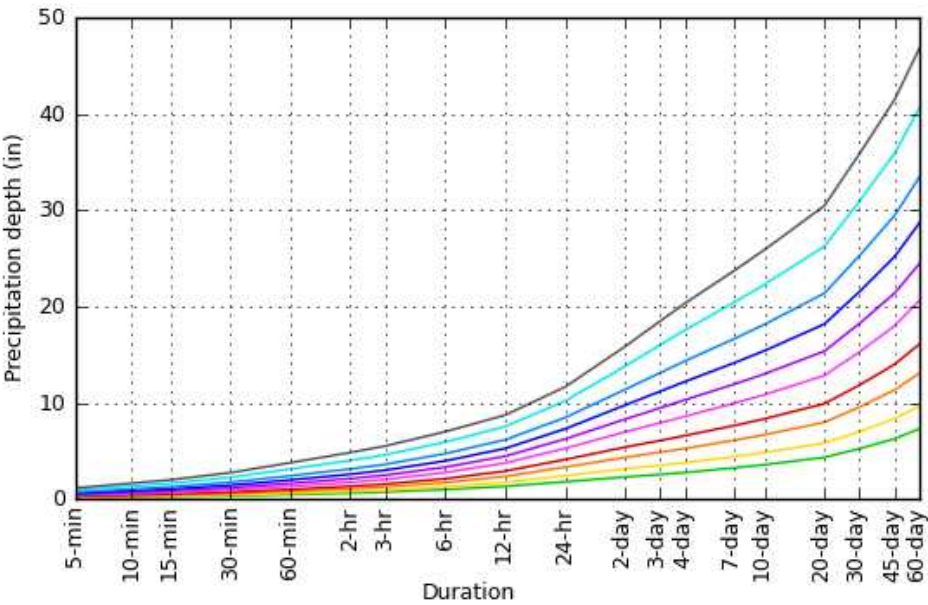
PDS-based depth-duration-frequency (DDF) curves Latitude: 32.6713°, Longitude: -116.3648°
