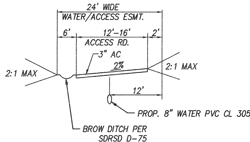
WATER LINE ACCESS EASEMENT NOT TO SCALE
