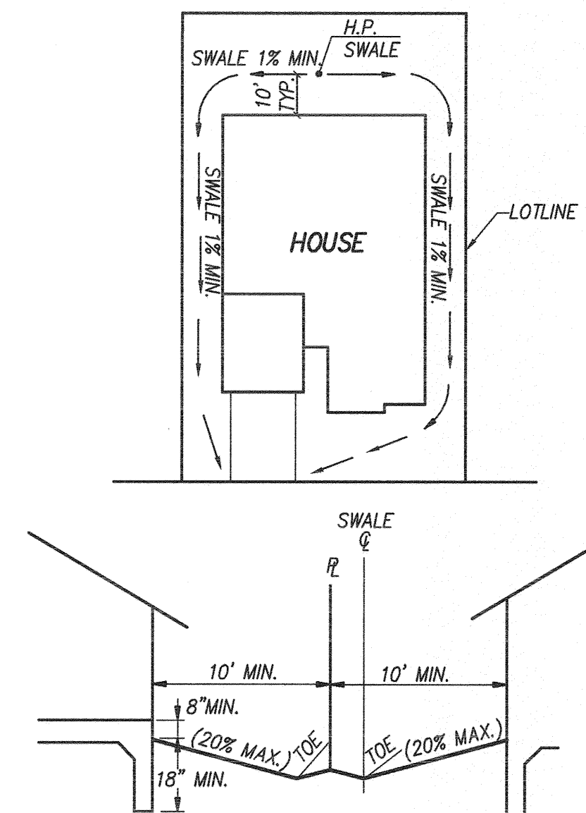
TYPICAL SWALE-SLOPE NOT TO SCALE
