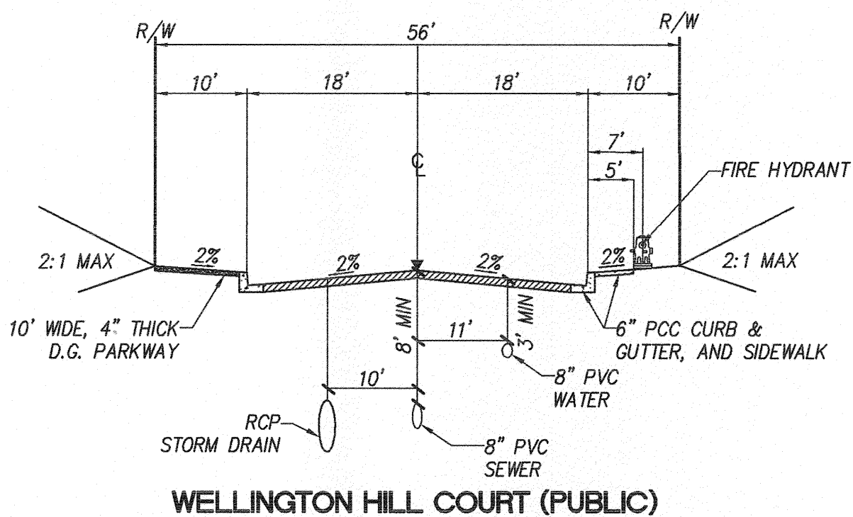
WELLINGTON HILL COURT (PUBLIC) WELLINGTON HILL CT.-FROM STA. 10+47.98 TO 19+81.41, FROM STA. 21+34.57 TO 26+17.37, FROM STA. 27+73.35 TO 29+50.89
