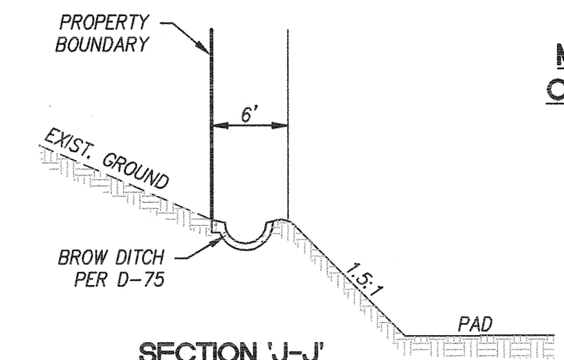
SECTION 'J-J' NOT TO SCALE
