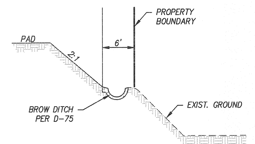
SECTION 'K-K' NOT TO SCALE
