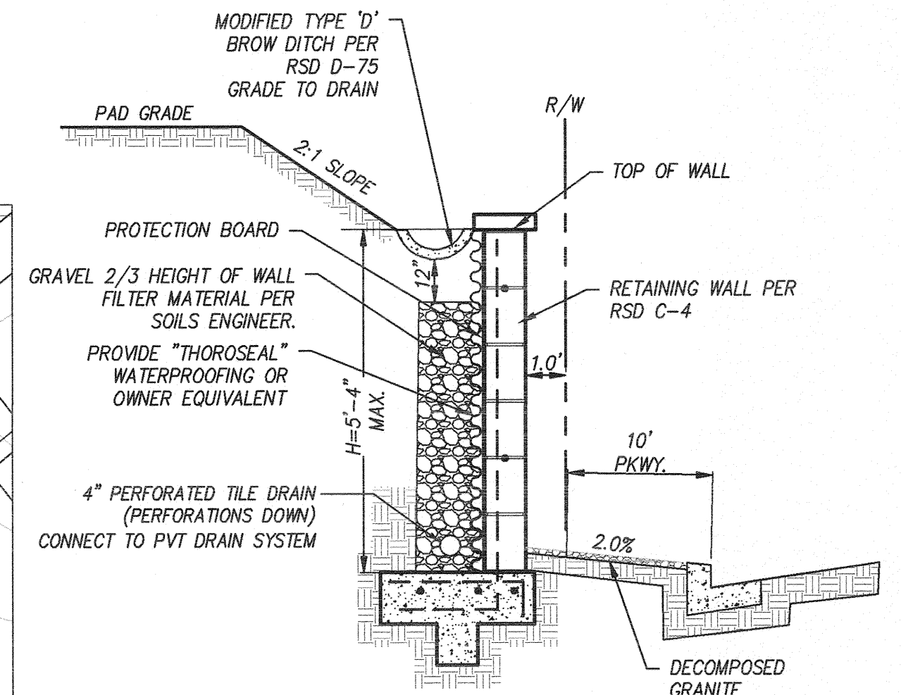
SECTION 'A-A' TYPICAL RET. WALL/SWALE SECTION NOT TO SCALE
