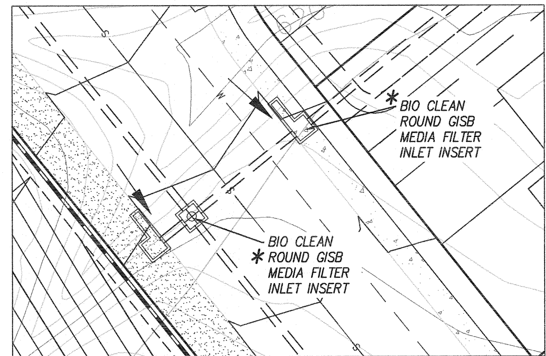
DETAIL S SCALE 1" = 20'
