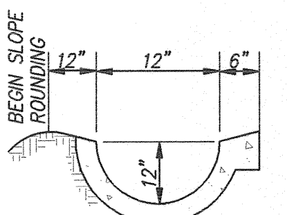
MODIFIED TYPE 'D' CONC. BROW DITCH NOT TO SCALE
